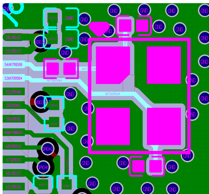
Fig. 5: ESP32-S3 Crystal Layout (without Keep-out Area on Top Layer)
