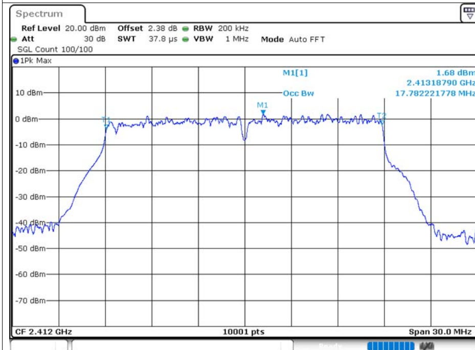
OBW NVNT n20 2412MHz Ant1
