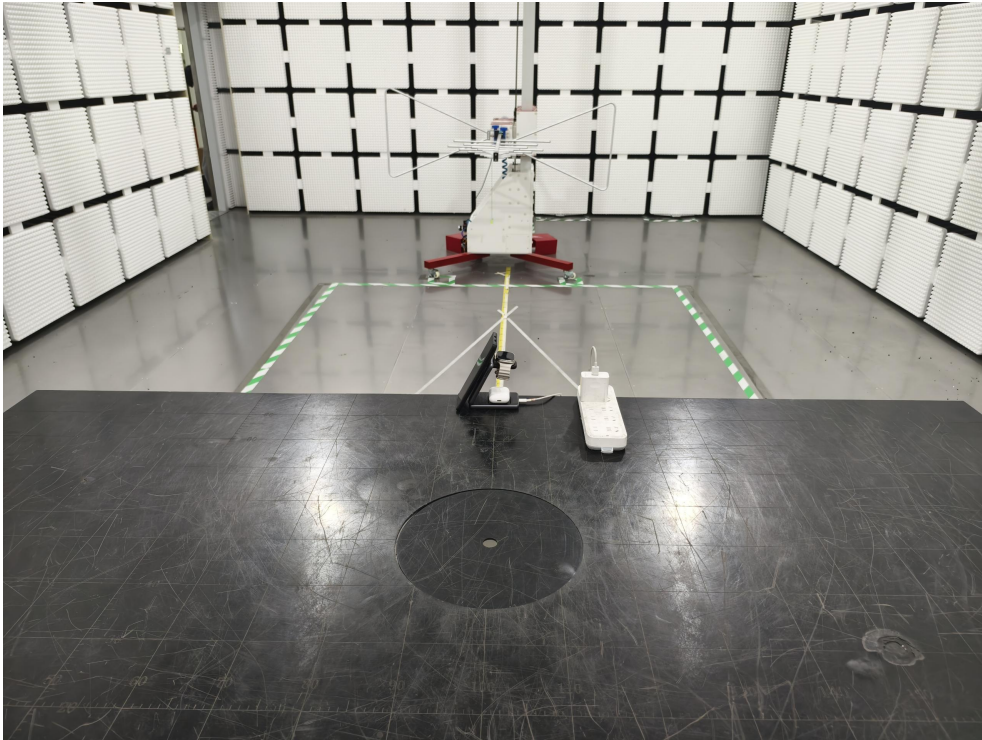
Spurious Radiation Emissions Test (30MHz-1GHz)
