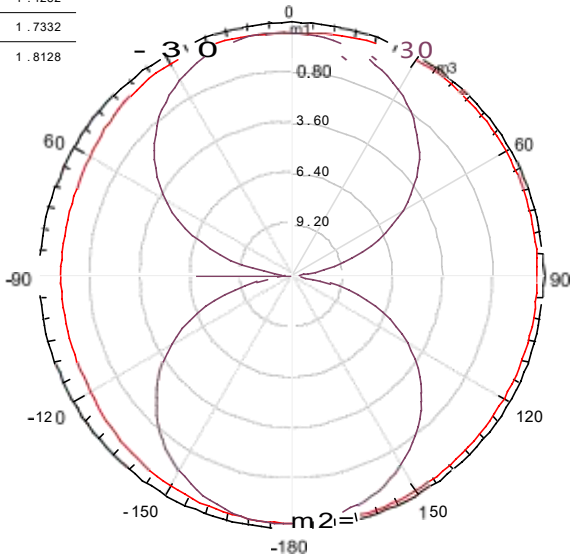
Radiation Patterns(GAIN @ 2440MHz)
