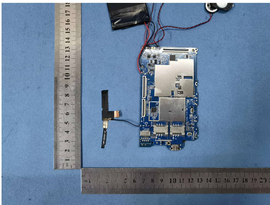
Wifi and BT ANT
