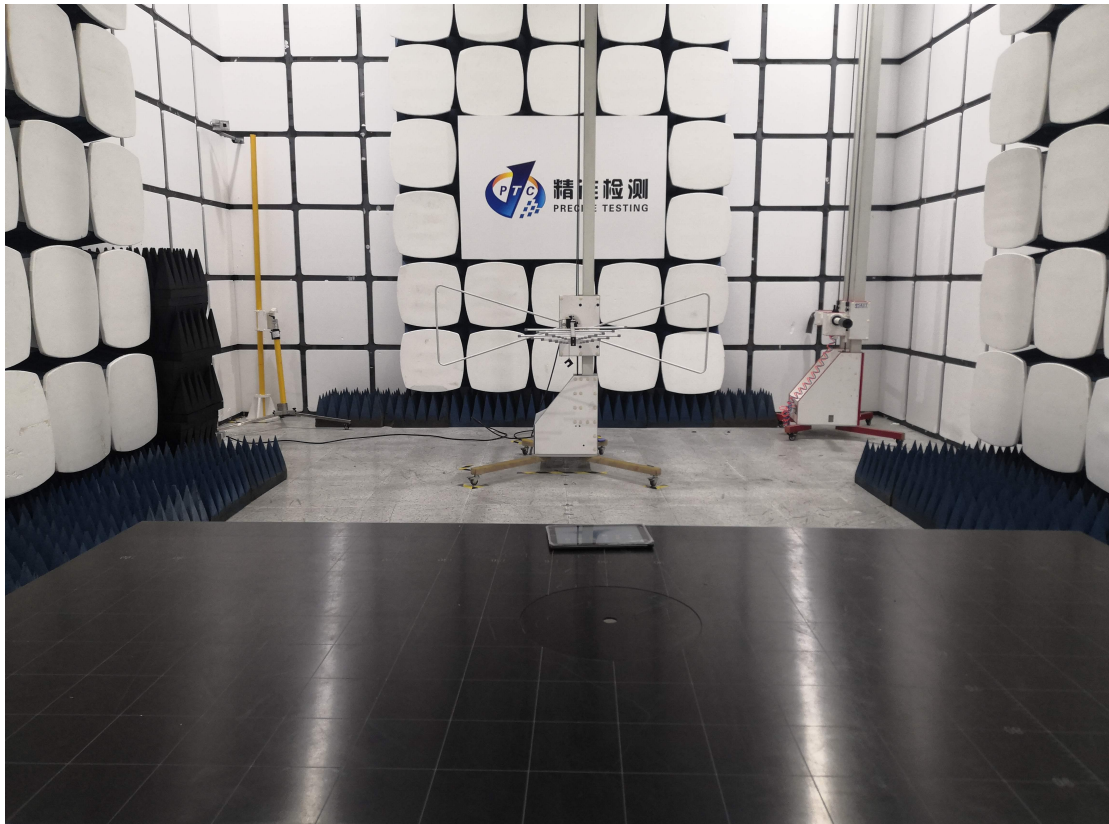
Radiated Spurious Emissions From 30MHz-1000MHz
