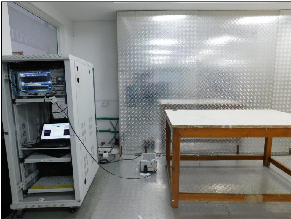
Conducted Emission Test Setup Photo
