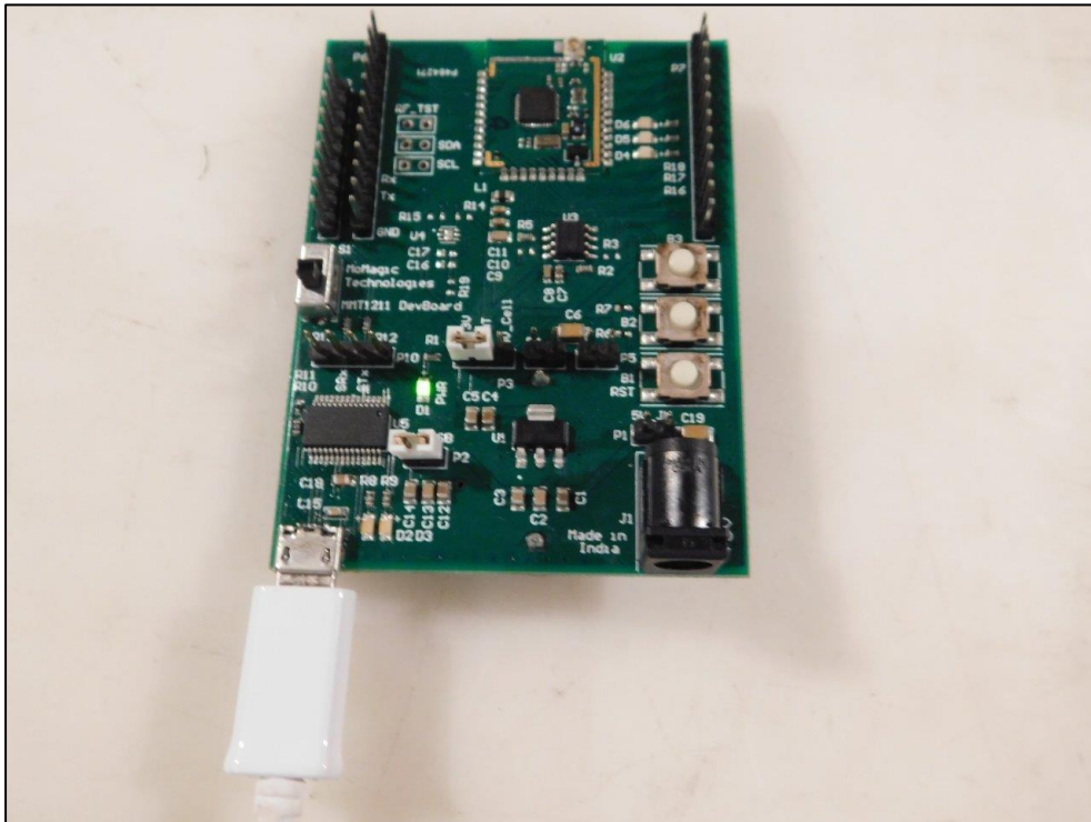
Radiated Test setup close-up
