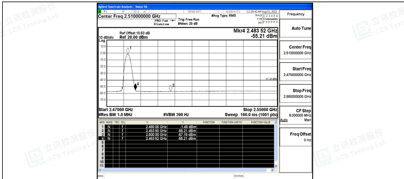
3DH5_Ant1_High_2480_Peak
