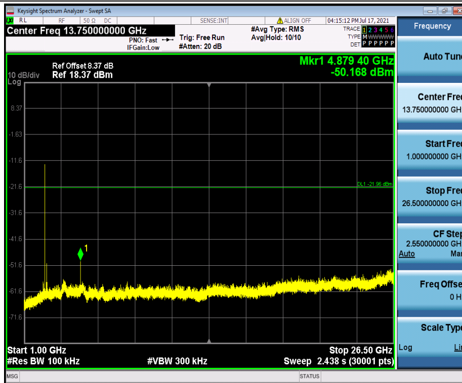
BLE_2M_Ant1_2440_1000~26500
