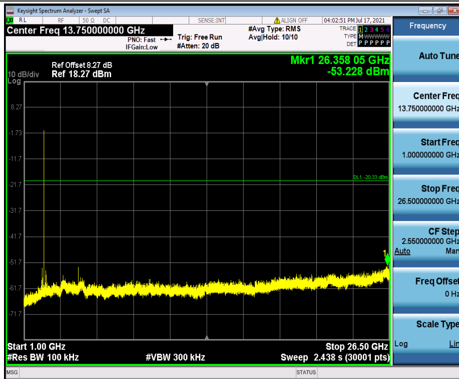
BLE_1M_Ant1_2402_1000~26500
