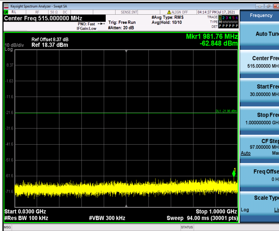
BLE_2M_Ant1_2440_30~1000
