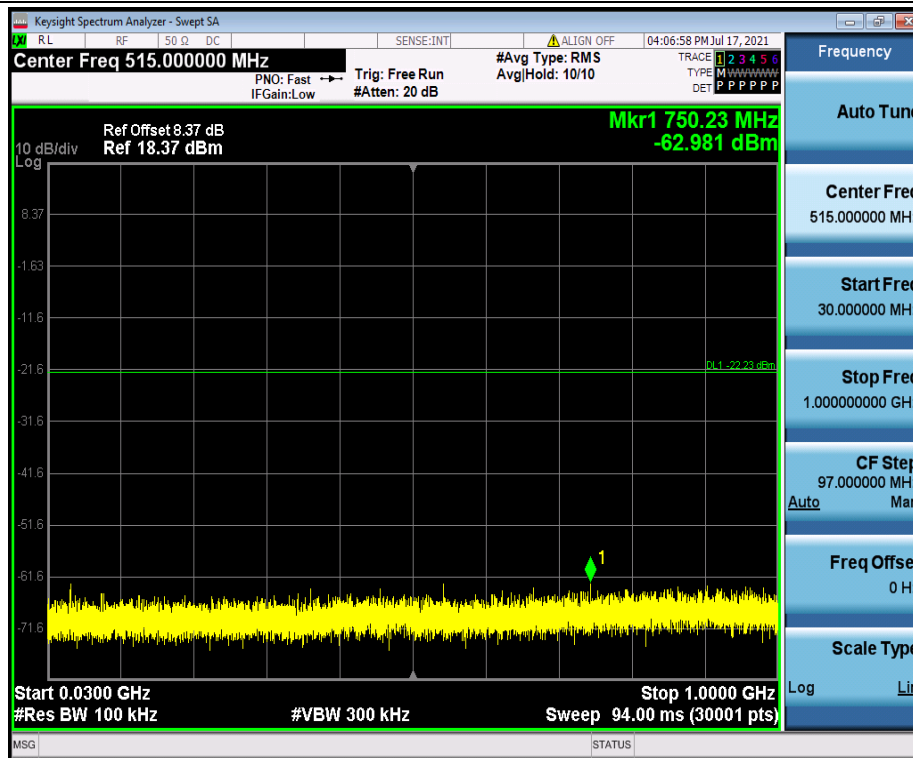
BLE_1M_Ant1_2440_30~1000
