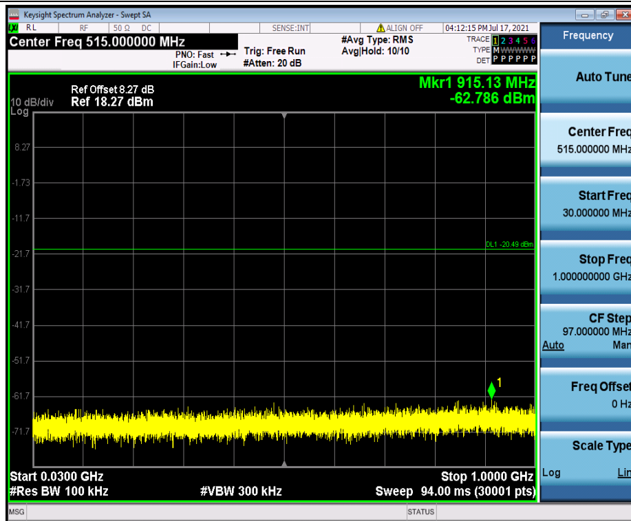
BLE_2M_Ant1_2402_30~1000
