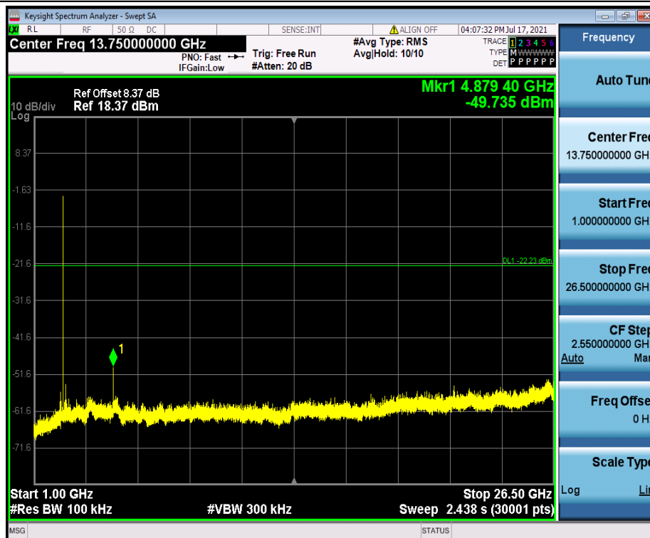
BLE_1M_Ant1_2440_1000~26500
