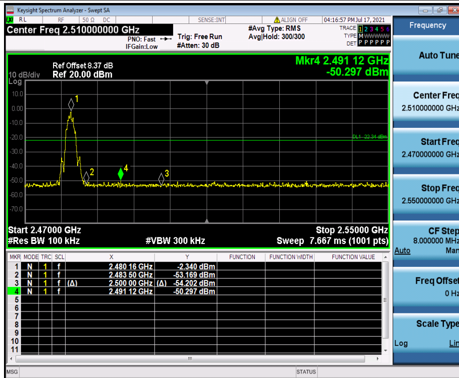
BLE_2M_Ant1_High_2480
