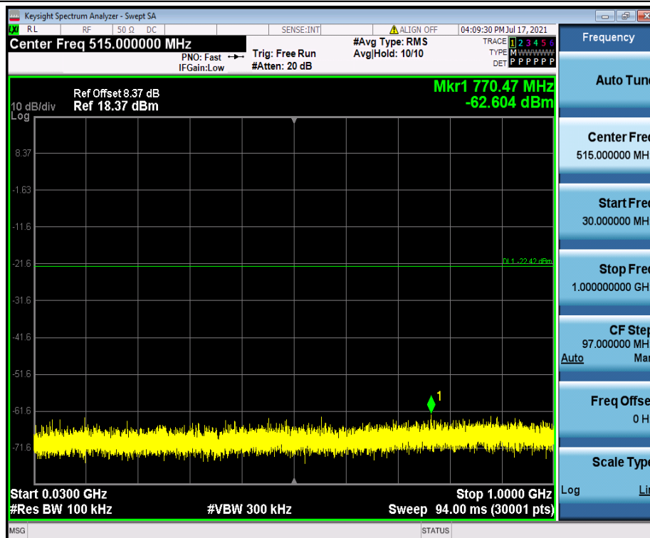
BLE_1M_Ant1_2480_30~1000
