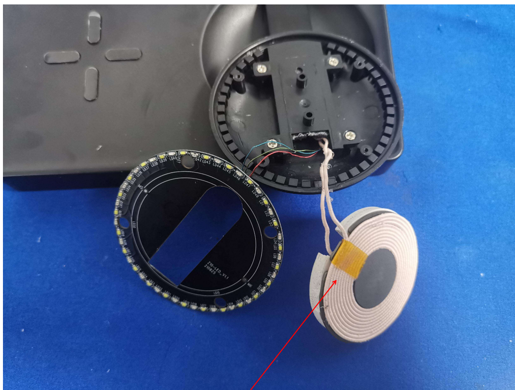
Phone Antenna
