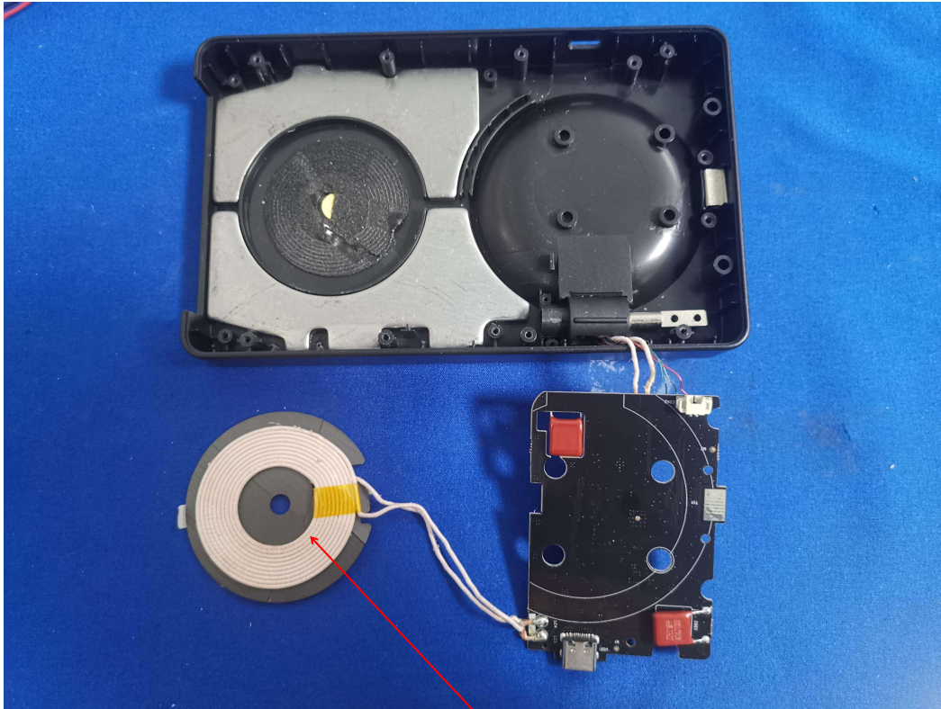
Earbuds Antenna
