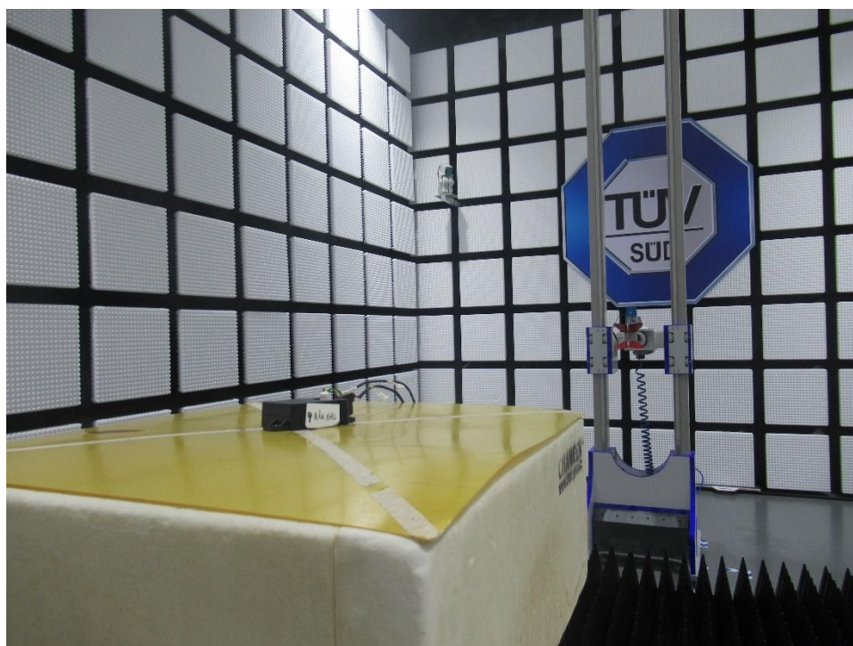
Radiated Emission test (1GHz-10GHz)
