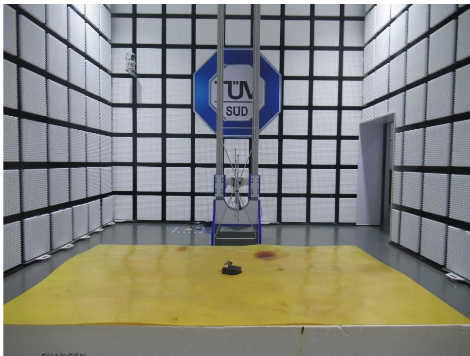
Radiated Emission test (30MHz to 1000MHz)
