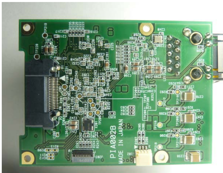
PCB2(Rear)
