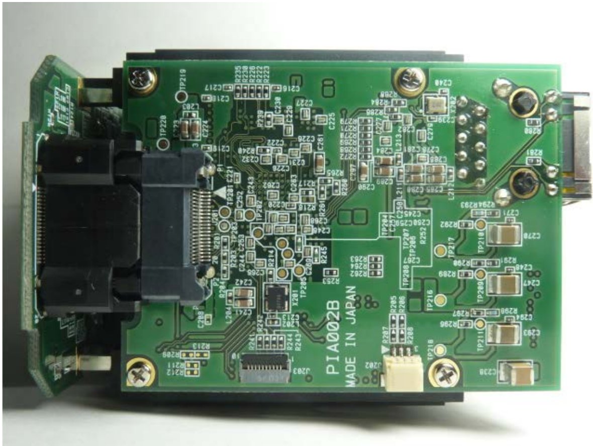
AssembledState_PCB2
