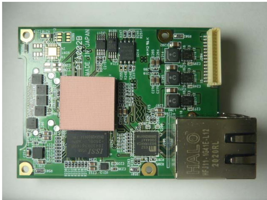
PCB2(Front)
