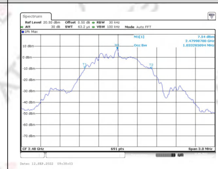
99% Bandwidth Mode3 CH 11
