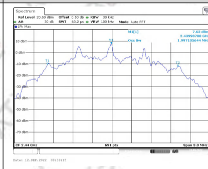
99% Bandwidth Mode5 CH19
