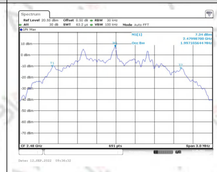
99% Bandwidth Mode6 CH39
