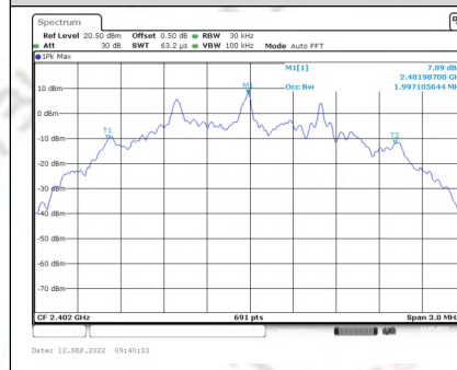
99% Bandwidth Mode4 CH00
