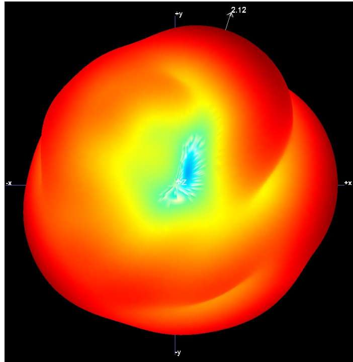
B1.1 3D Pattern for 2400MHz
