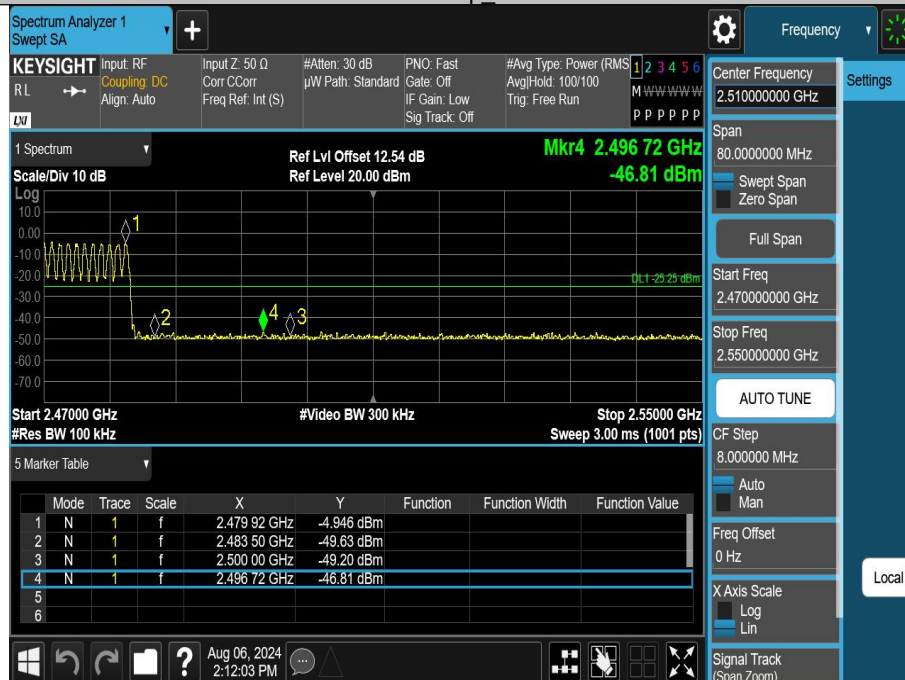
GFSK-Ant1-Hop_2480-PASS
