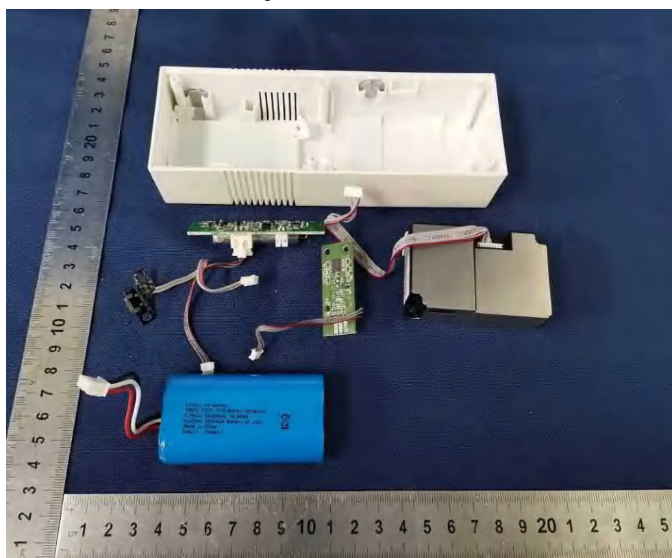
Fig.10 Internal view-04
