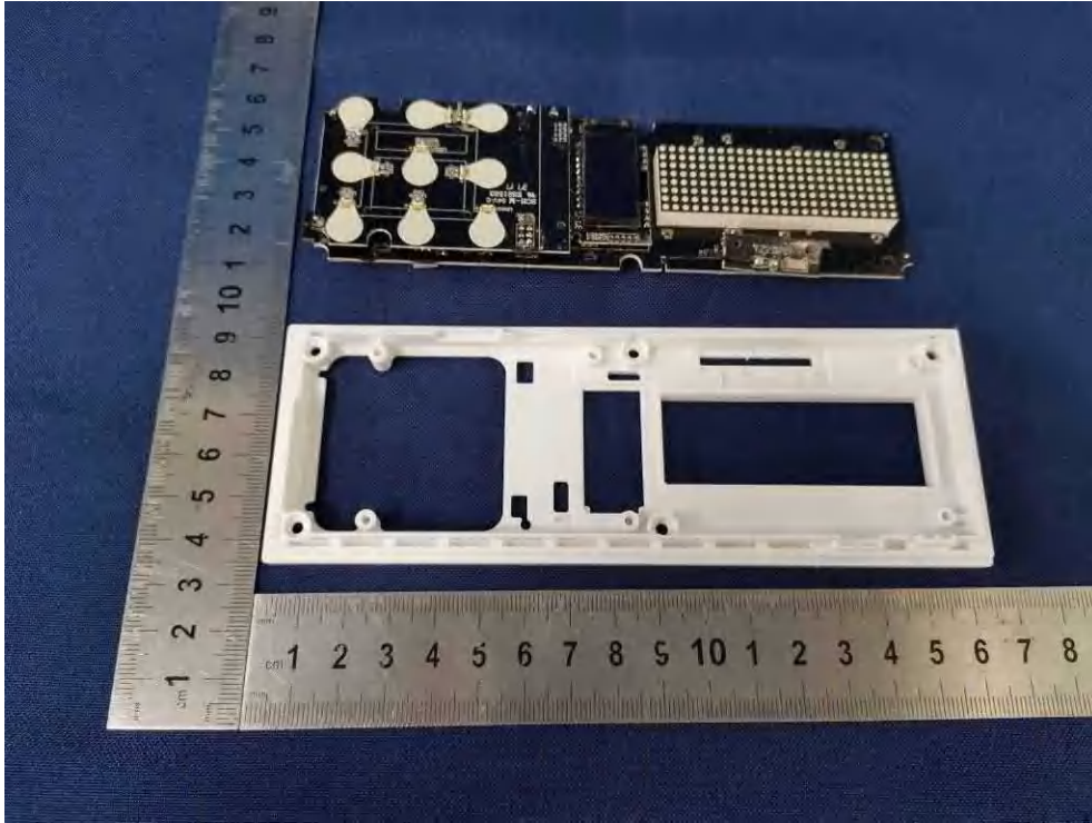
Fig.12 Internal view-06
