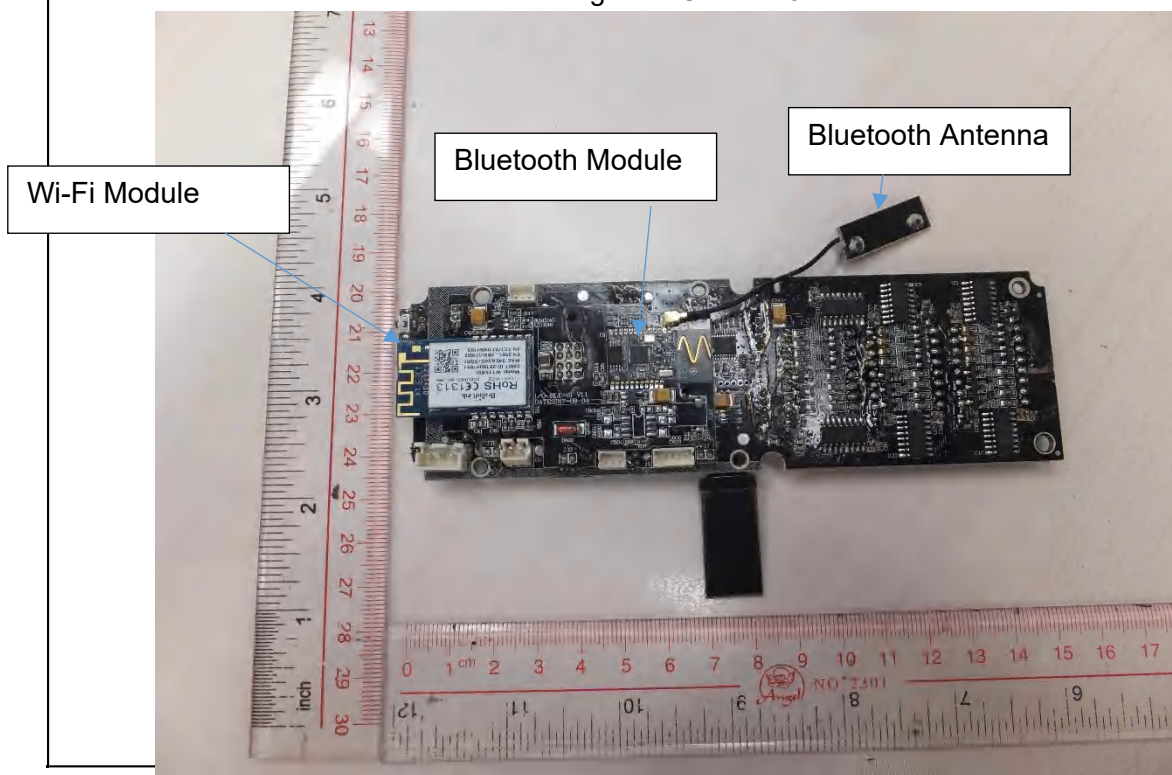
Fig.14 PCB view-01
