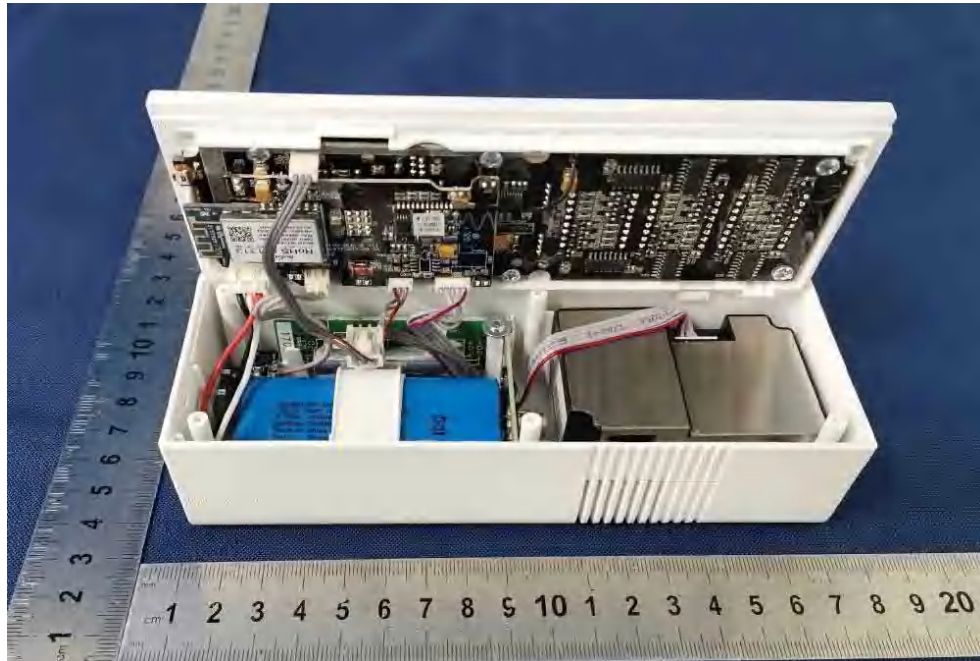
Fig.8 Internal view-02
