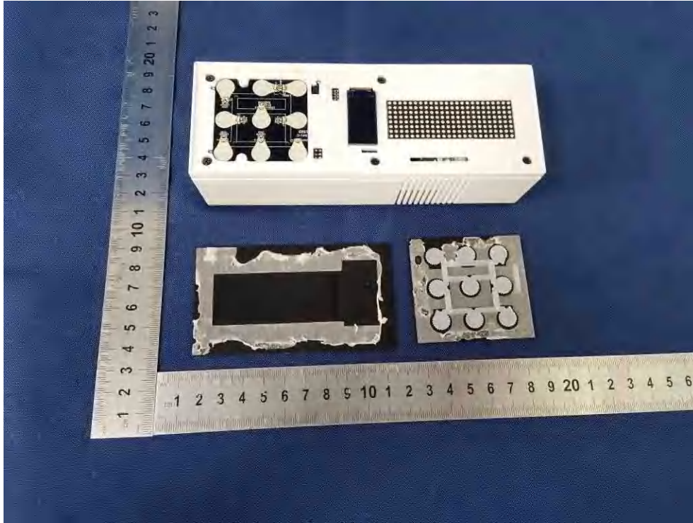
Fig.8 Internal view-02
