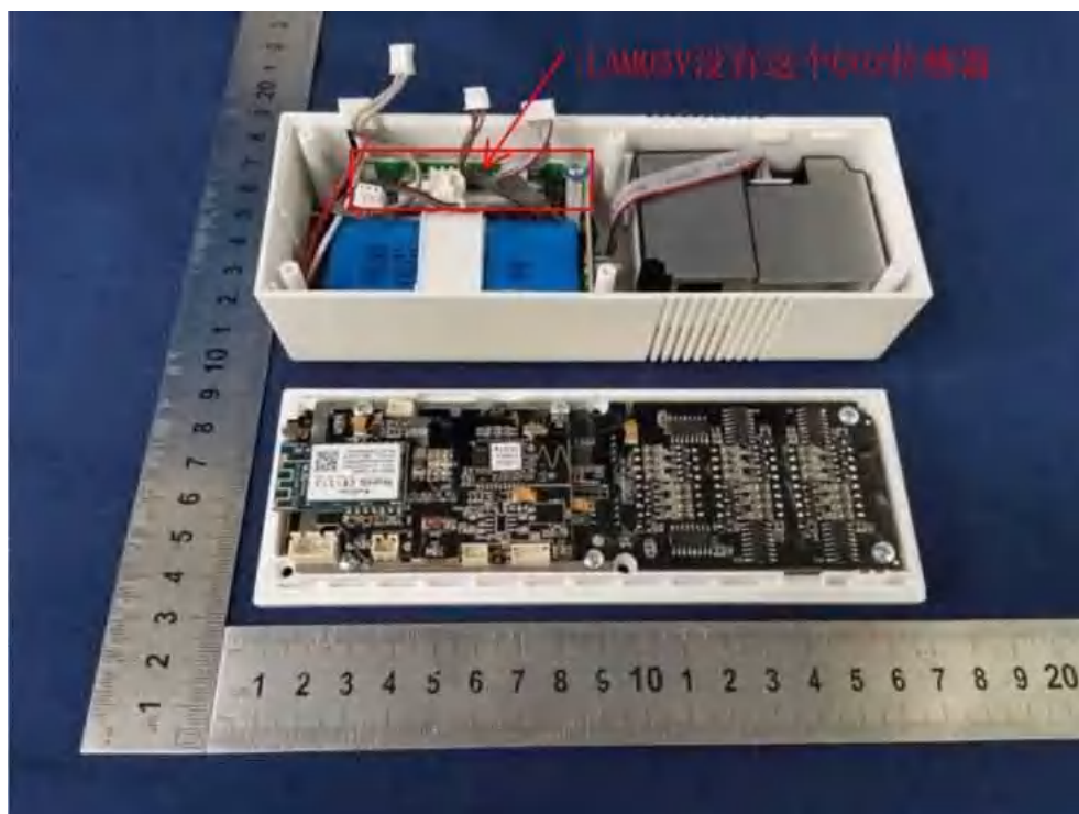
Fig.10 Internal view-04
