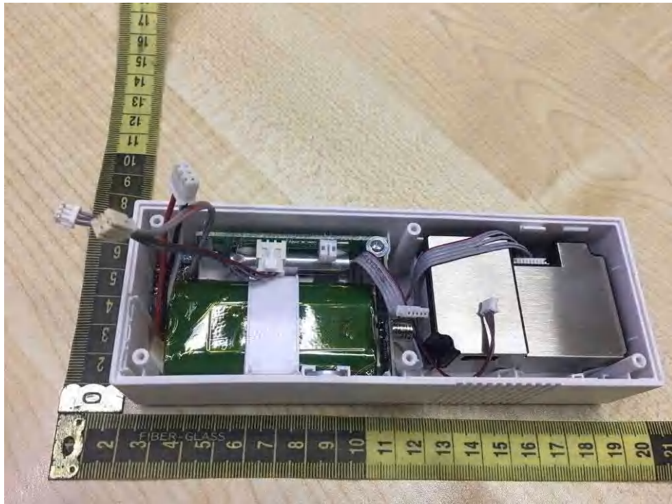
Fig.12 Internal view-06
