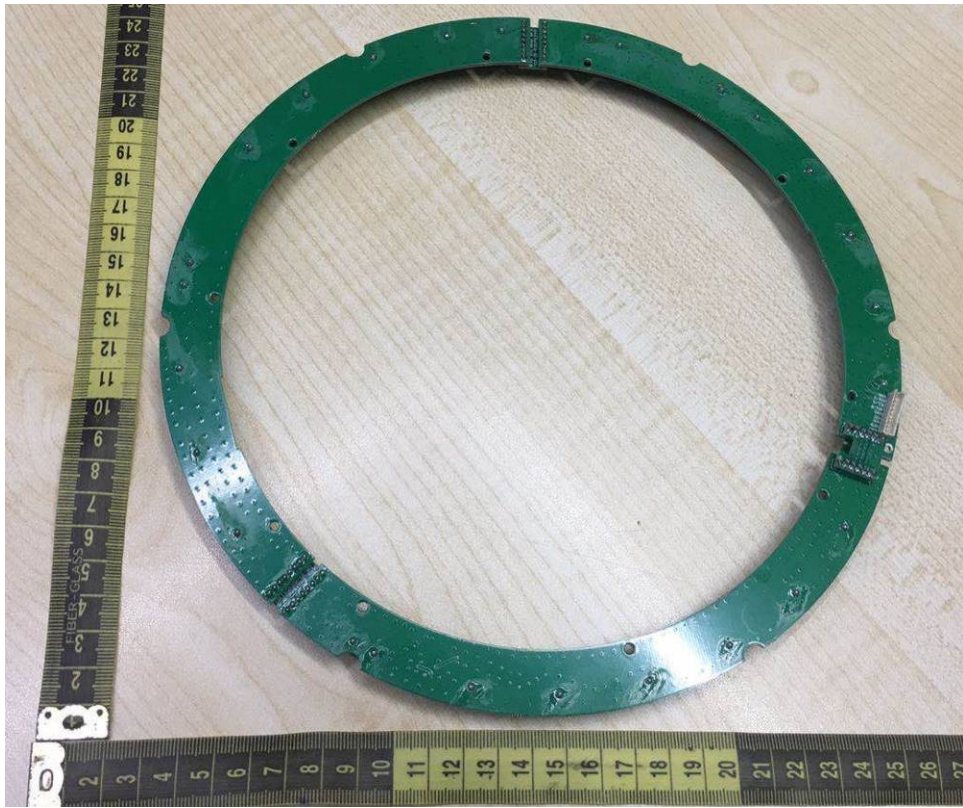
Figure 25. View of control PCB
