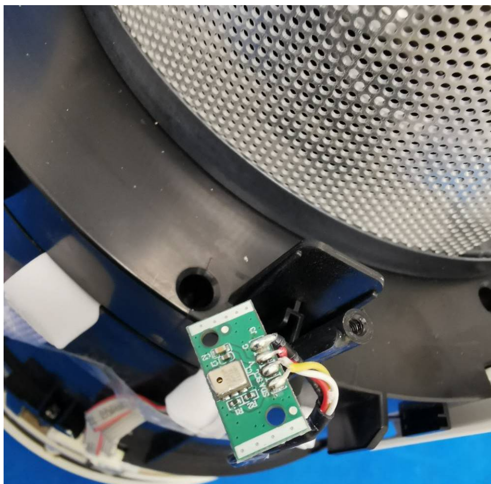
Figure 4. Internal view
