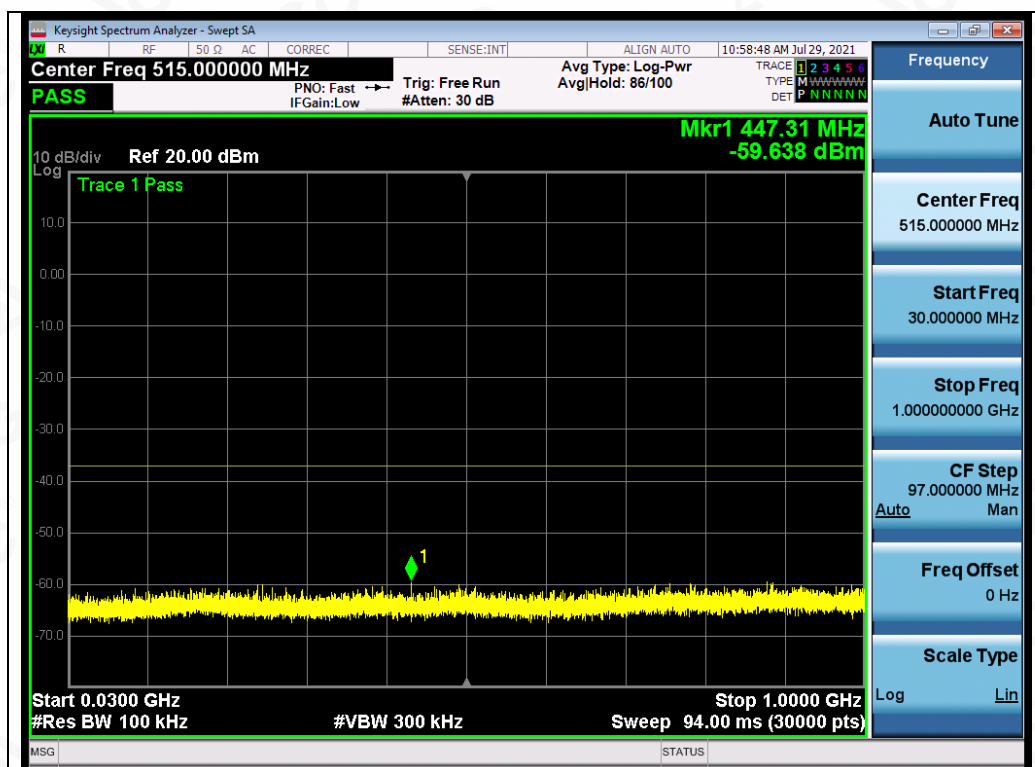
Test_Graph_802.11n40_ANT1_5670_MCS0_Frequency Band 1
