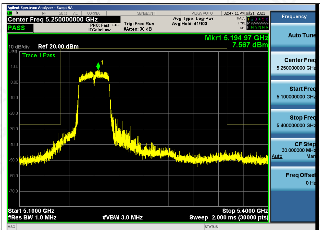
Test_Graph_802.11n40_ANT1_5190_MCS0_Frequency Band 3
