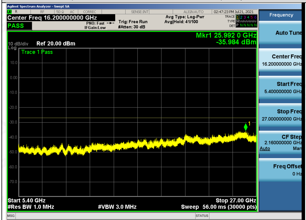
Test_Graph_802.11n40_ANT1_5190_MCS0_Frequency Band 4
