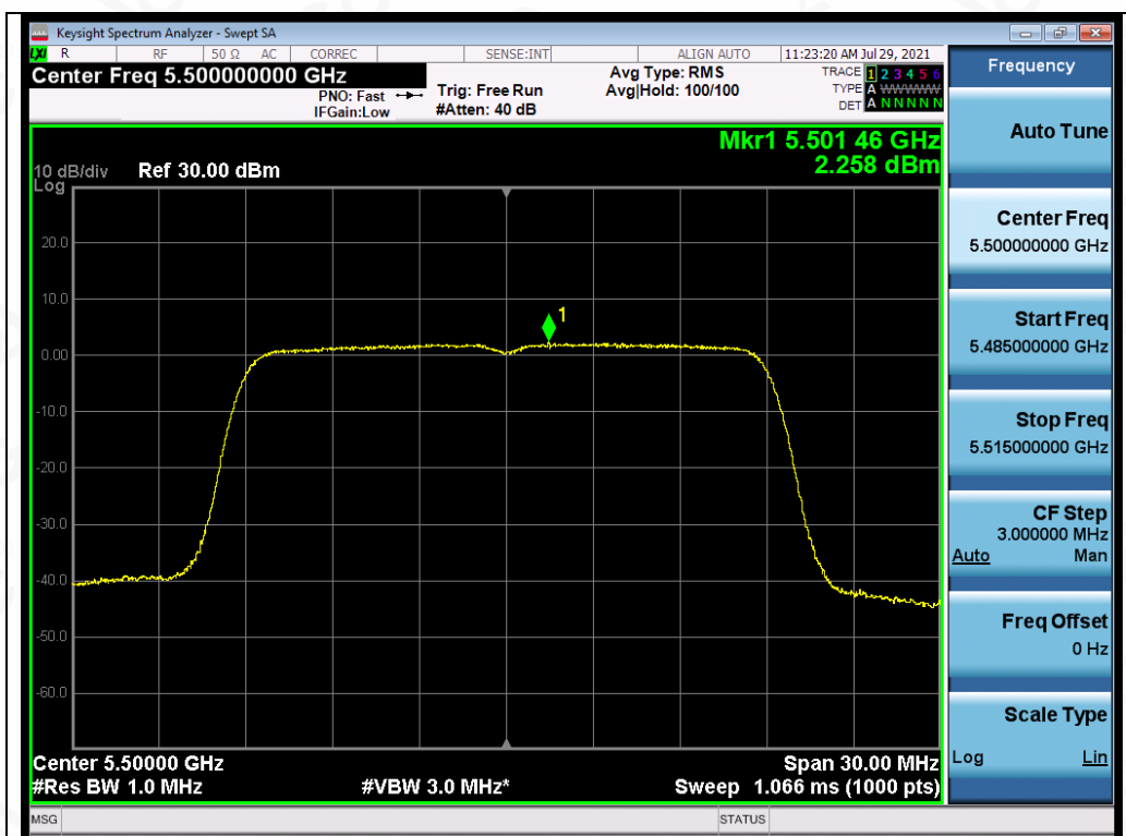
Test_Graph_802.11n20_ANT2_5500_MCS0_PSD
