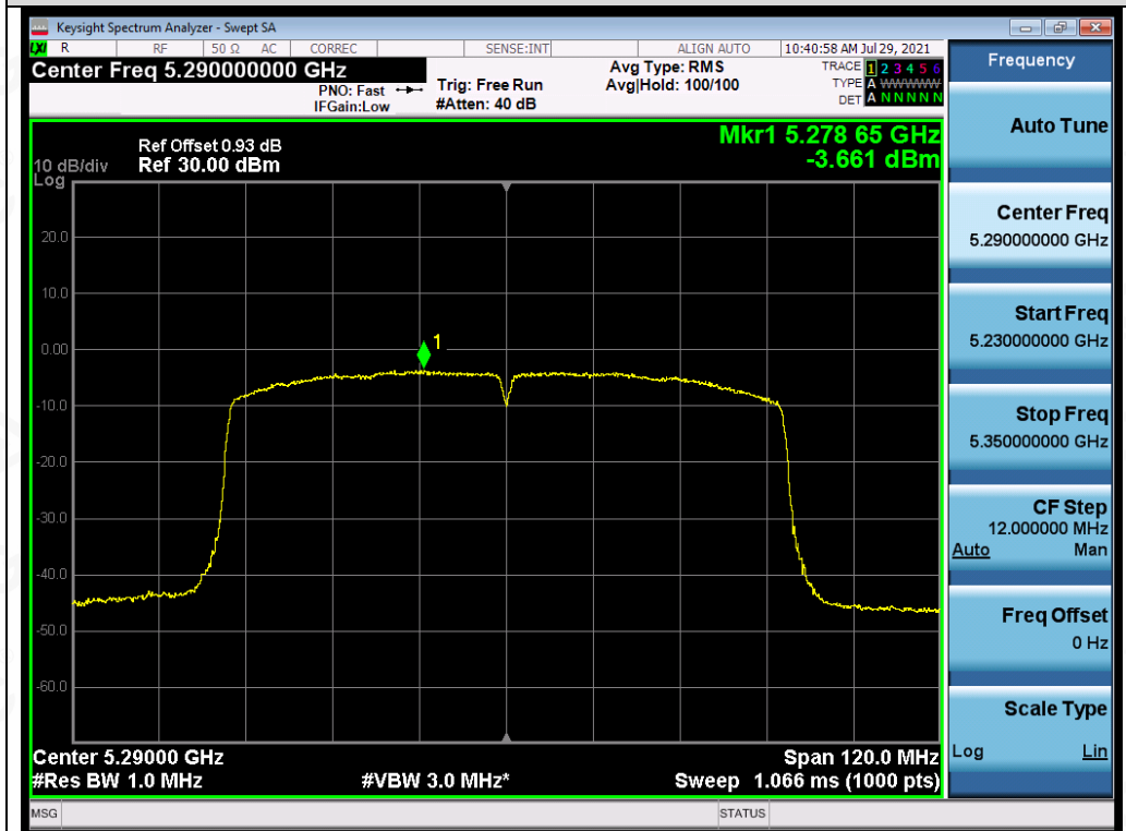
Test_Graph_802.11ac80_ANT2_5290_MCS9_PSD
