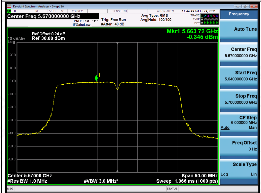
Test_Graph_802.11ac40_ANT2_5670_MCS9_PSD
