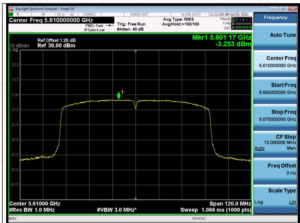
Test_Graph_802.11ac80_ANT1_5610_MCS9_PSD
