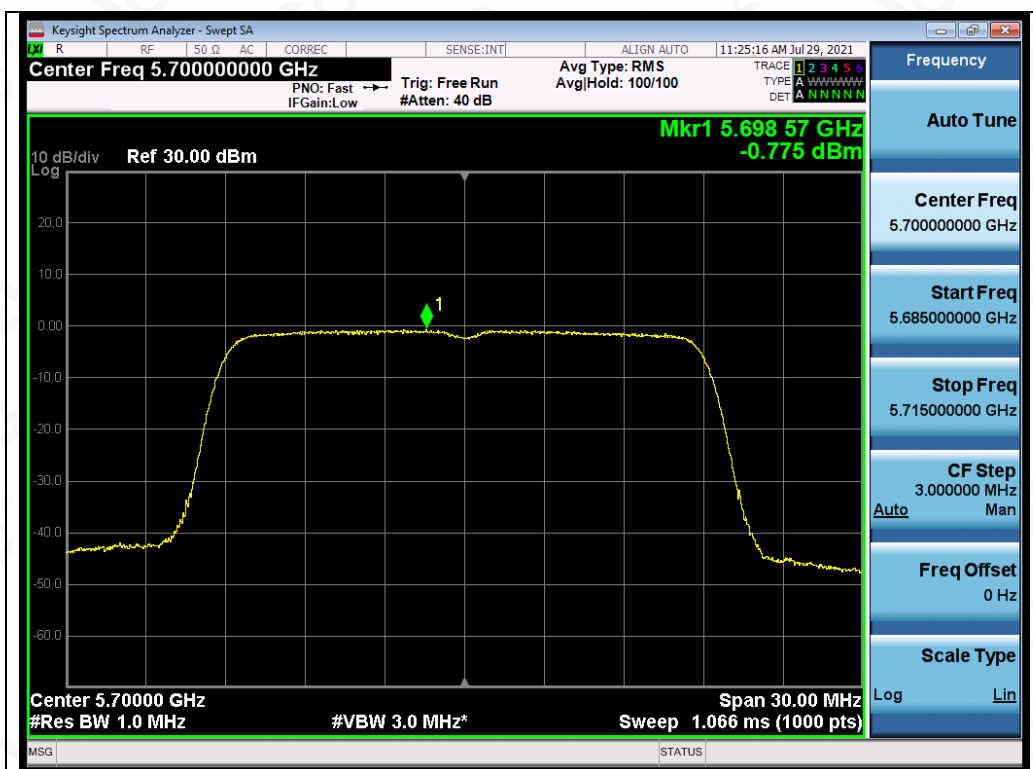
Test_Graph_802.11n20_ANT2_5700_MCS0_PSD
