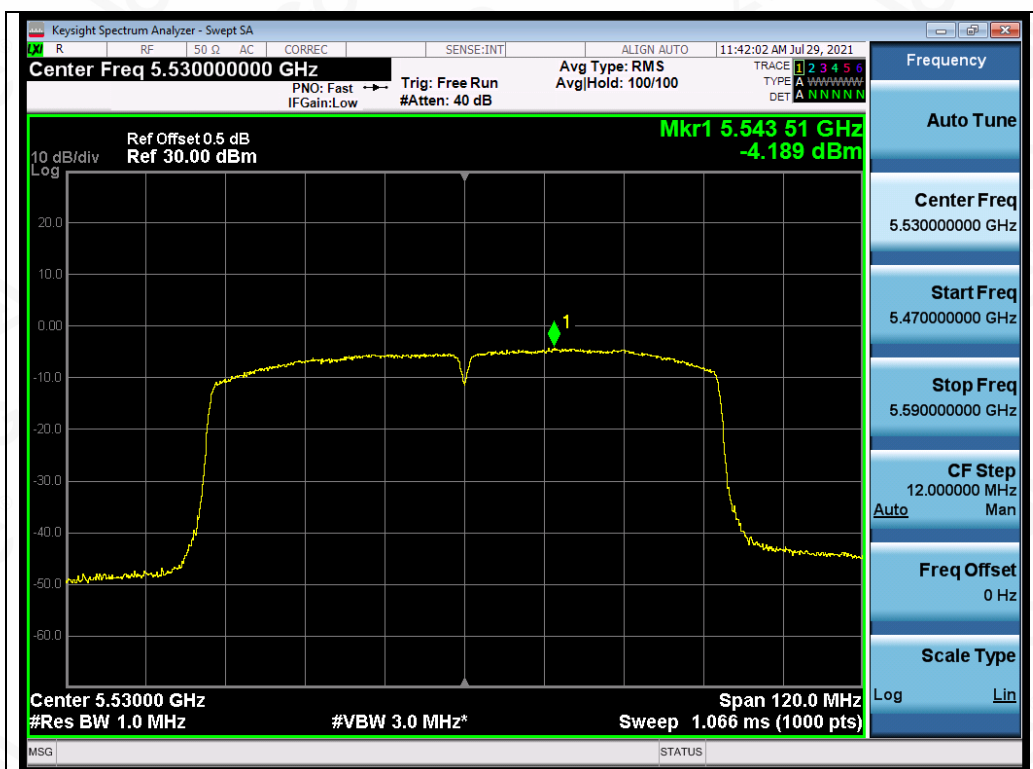
Test_Graph_802.11ac80_ANT2_5530_MCS9_PSD
