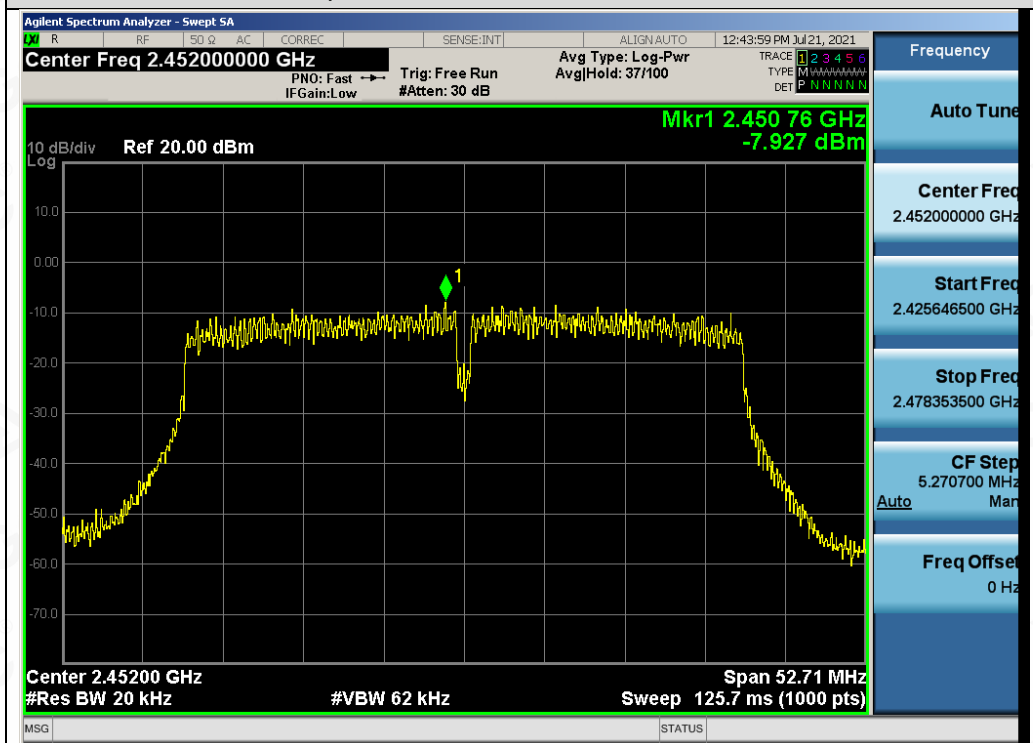
Test_Graph_802.11n40_ANT2_2452_MCS0_PSD
