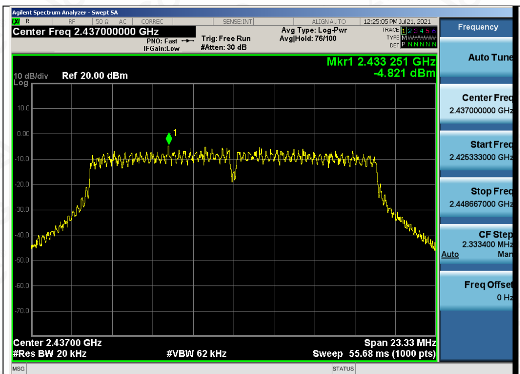
Test_Graph_802.11g_ANT2_2437_6Mbps_PSD
