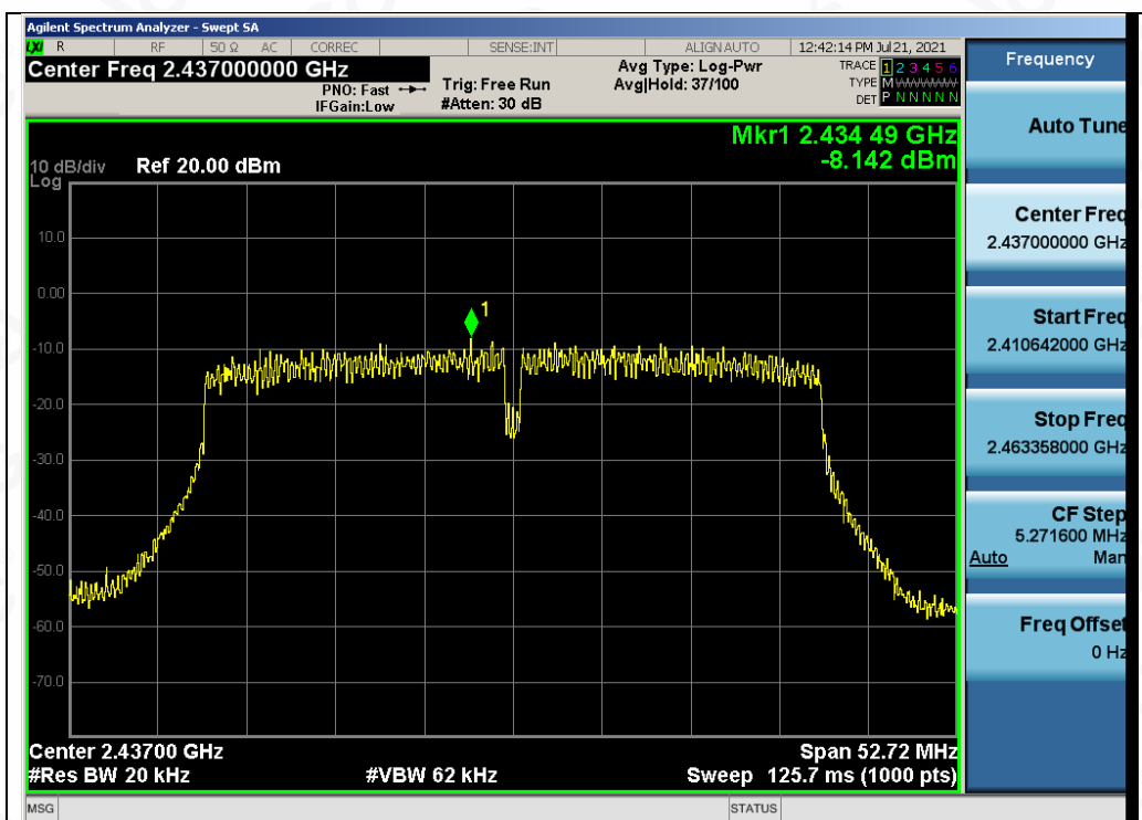
Test_Graph_802.11n40_ANT2_2437_MCS0_PSD
