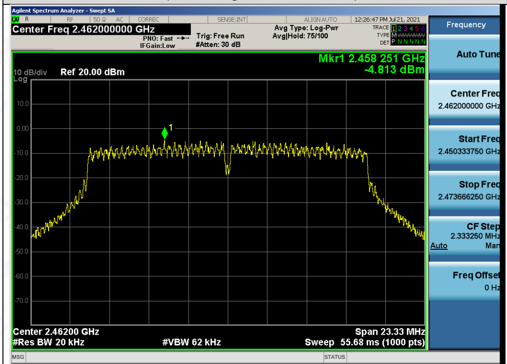
Test_Graph_802.11g_ANT2_2462_6Mbps_PSD
