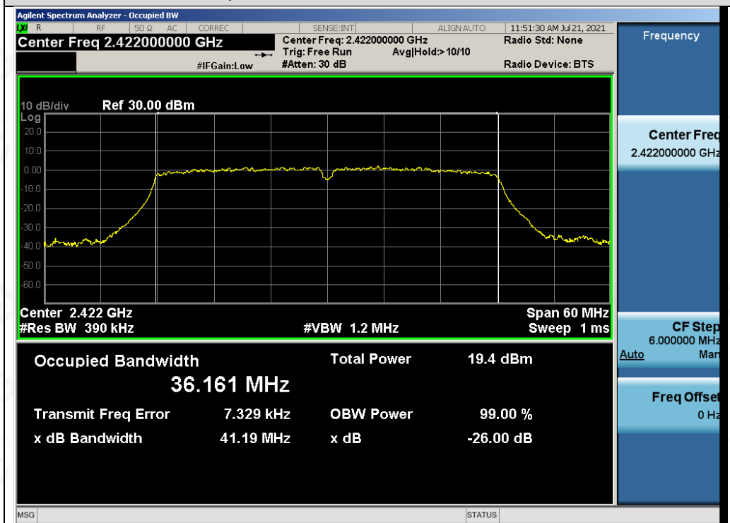
Test_Graph_802.11n40_ANT1_2422_MCS0_OBW
