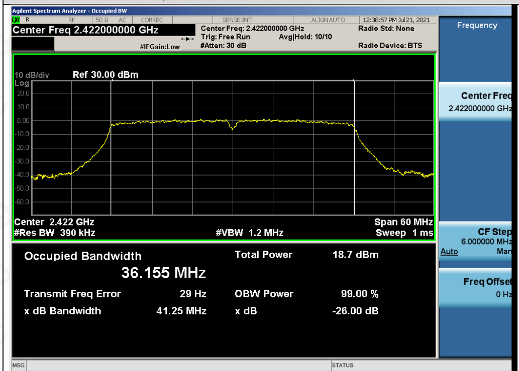
Test_Graph_802.11n40_ANT2_2422_MCS0_OBW
