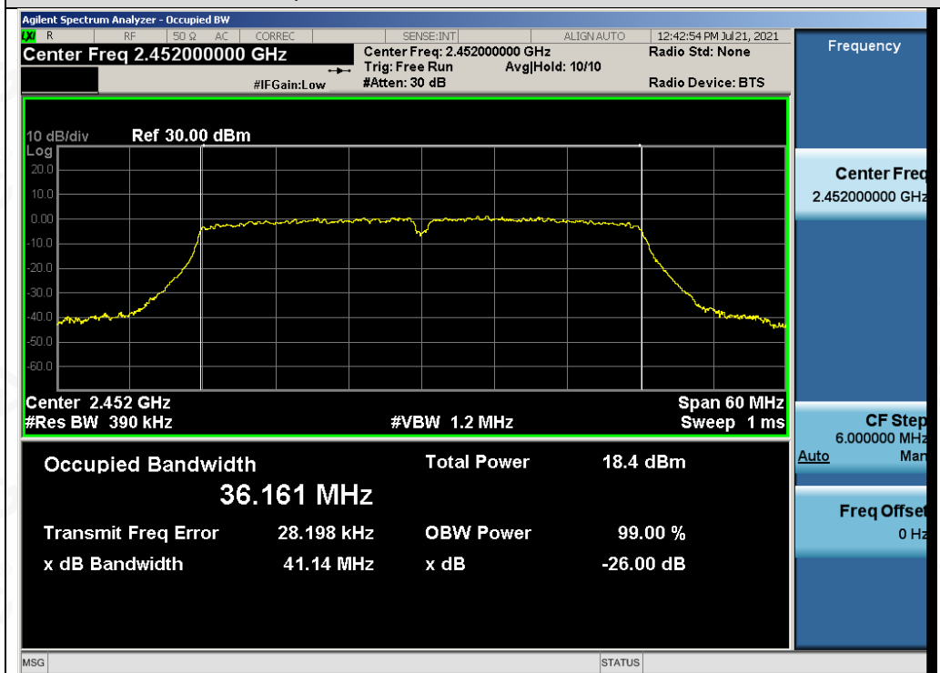
Test_Graph_802.11n40_ANT2_2452_MCS0_OBW
