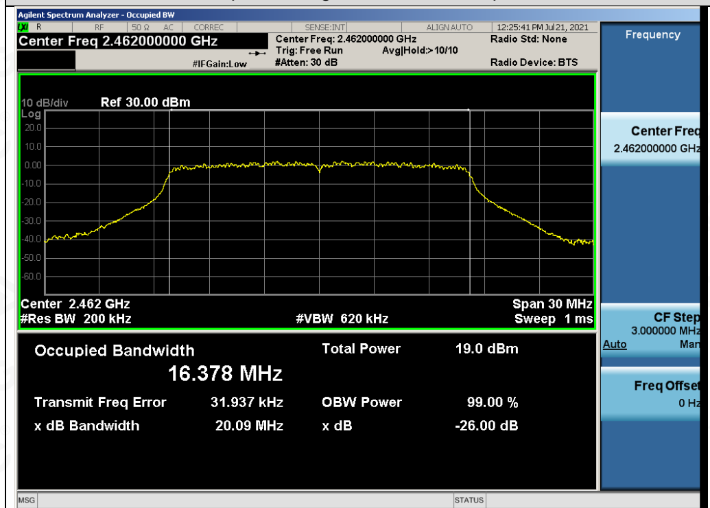
Test_Graph_802.11g_ANT2_2462_6Mbps_OBW
