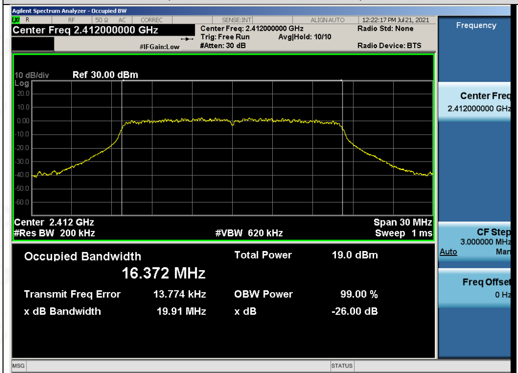
Test_Graph_802.11g_ANT2_2412_6Mbps_OBW
