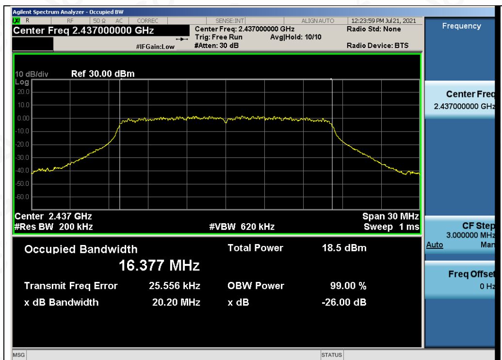
Test_Graph_802.11g_ANT2_2437_6Mbps_OBW
