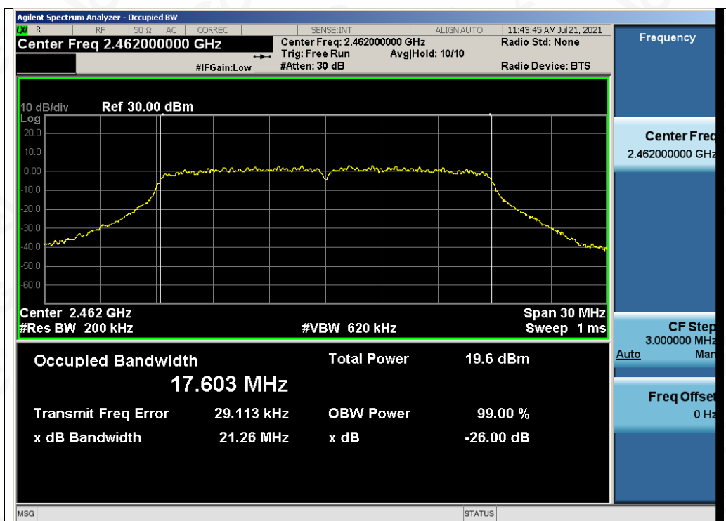
Test_Graph_802.11n20_ANT1_2462_MCS0_OBW
