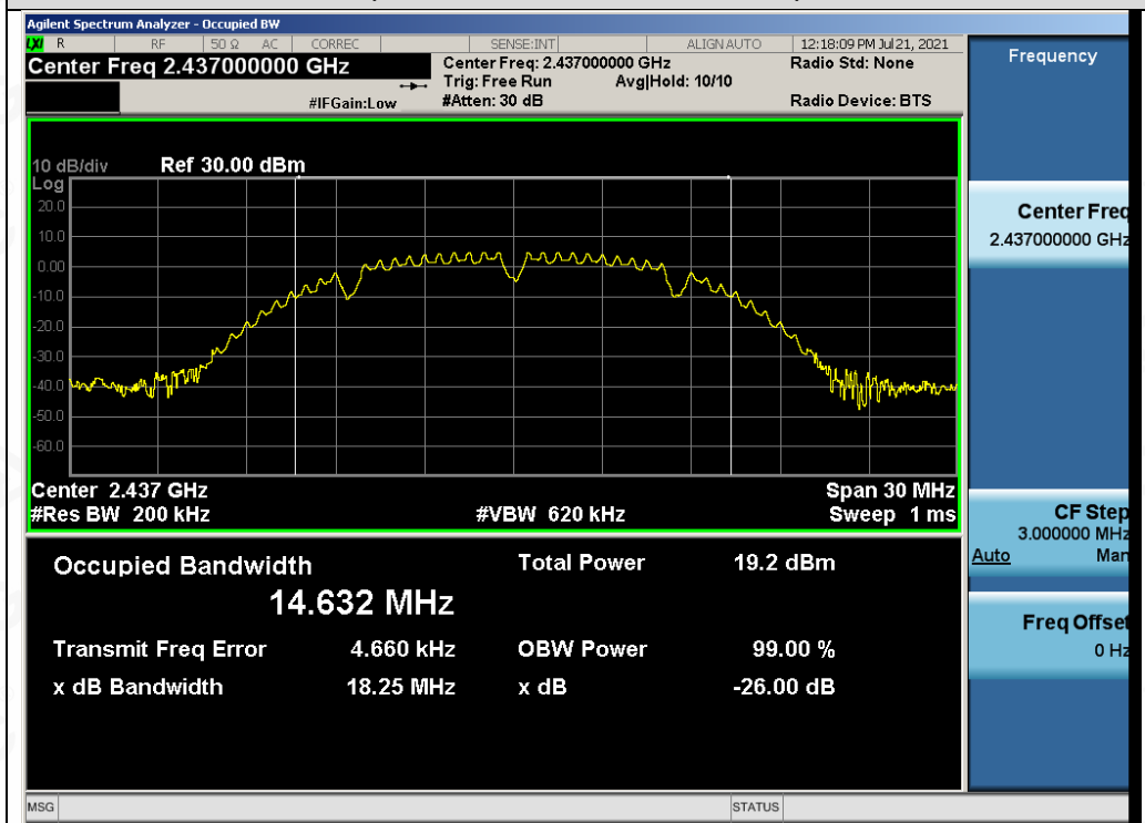
Test_Graph_802.11b_ANT2_2437_1Mbps_OBW
