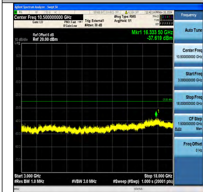
Band41_20MHz_16QAM_40140_1RB#0_3000~18000_3000~18000
