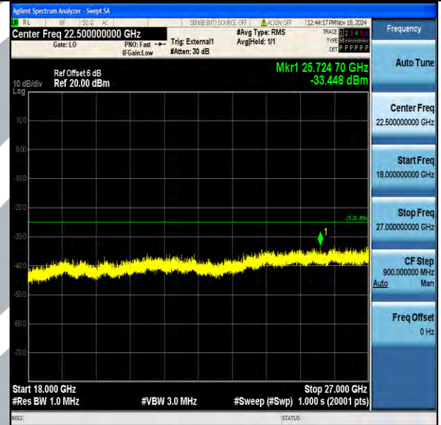
Band41_20MHz_QPSK_40590_1RB#0_18000~27000_18000~27000
