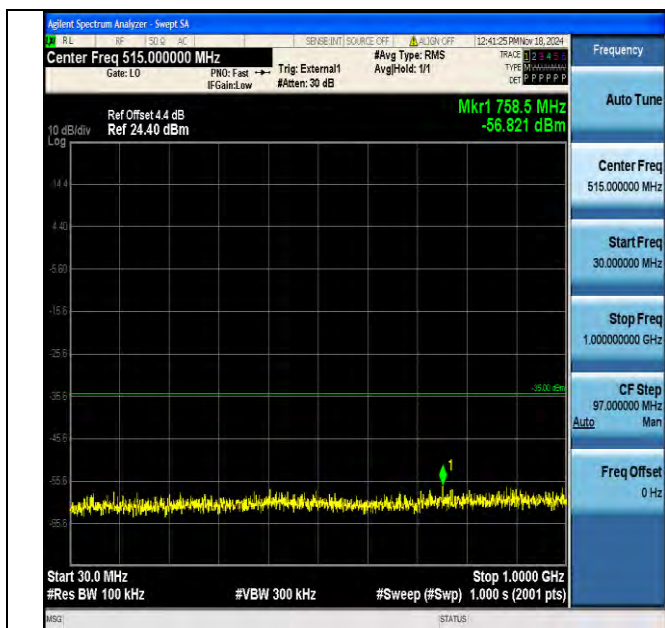
Band41_20MHz_16QAM_40140_1RB#0_30~1000_30~1000
