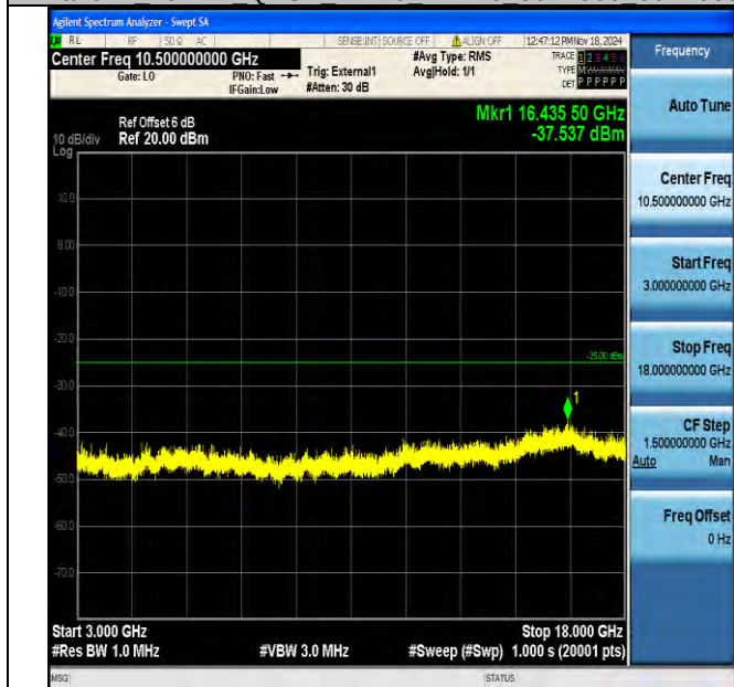
Band41_20MHz_QPSK_41140_1RB#0_3000~18000_3000~18000
