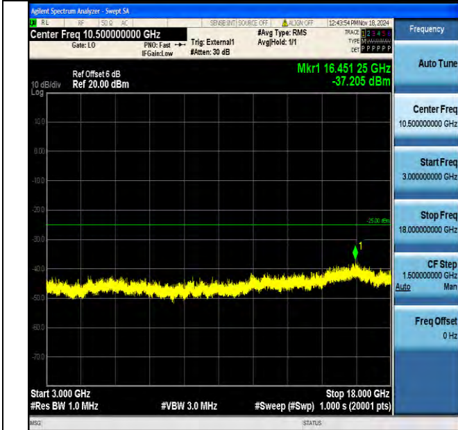
Band41_20MHz_QPSK_40590_1RB#0_3000~18000_3000~18000
