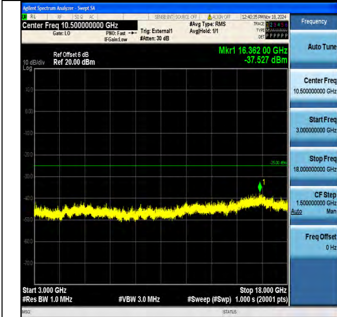
Band41_20MHz_QPSK_40140_1RB#0_3000~18000_3000~18000
