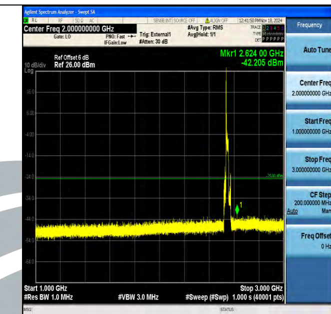
Band41_20MHz_16QAM_40140_1RB#0_1000~3000_1000~3000
