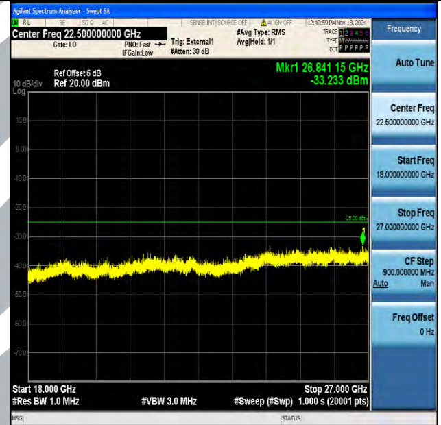
Band41_20MHz_QPSK_40140_1RB#0_18000~27000_18000~27000
