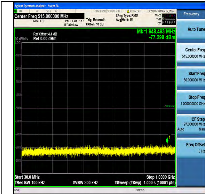
Band40_5MHz_16QAM_39200_1RB#0_30~1000_30~1000
