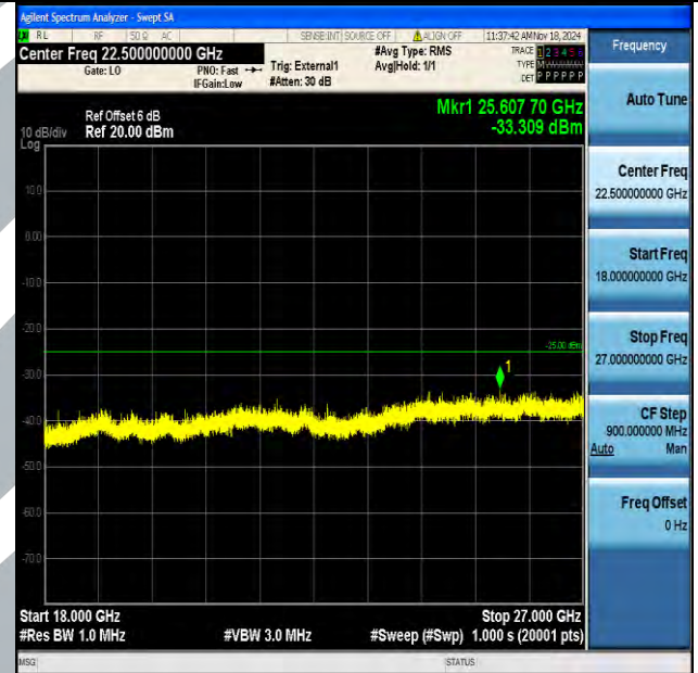
Band41_10MHz_QPSK_40590_1RB#0_18000~27000_18000~27000
