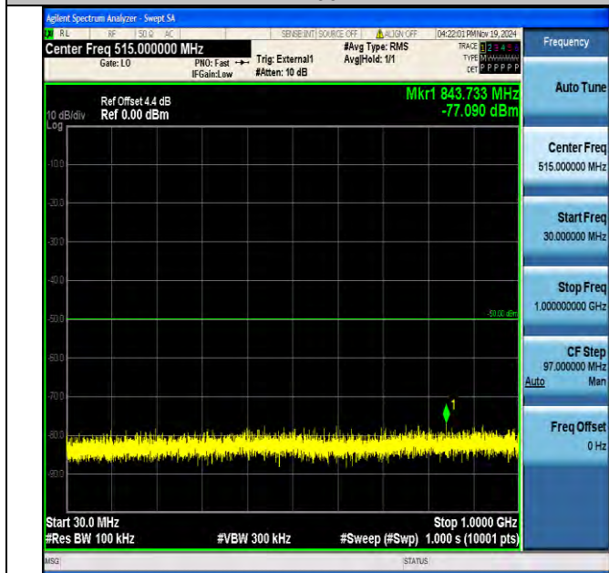
Band40_10MHz_QPSK_39200_1RB#0_30~1000_30~1000
