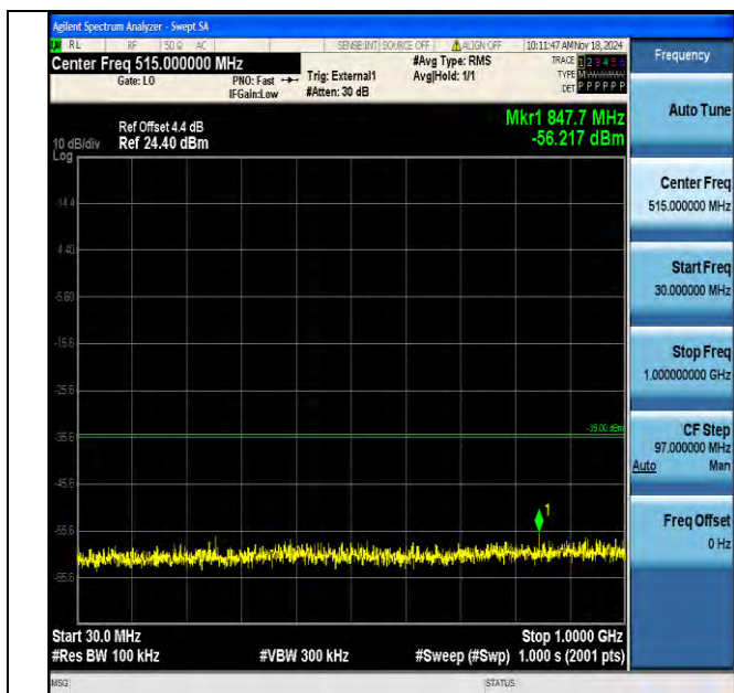
Band41 5MHz 16QAM 40065 1RB#0 30~1000 30~1000
