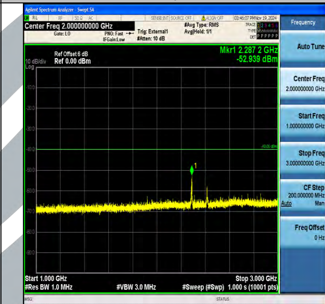
Band40_5MHz_QPSK_38775_1RB#0_1000~3000_1000~3000
