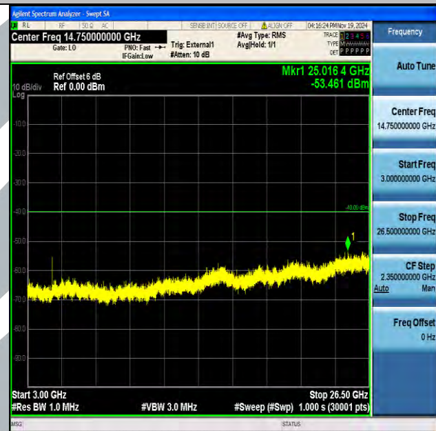
Band40_5MHz_16QAM_39175_1RB#0_3000~26500_3000~26500
