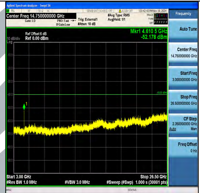
Band40_5MHz_16QAM_38725_1RB#0_3000~26500_3000~26500
