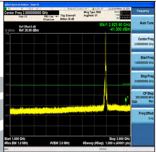
Band41 15MHz QPSK 40590 1RB#0 1000~3000 1000~3000
