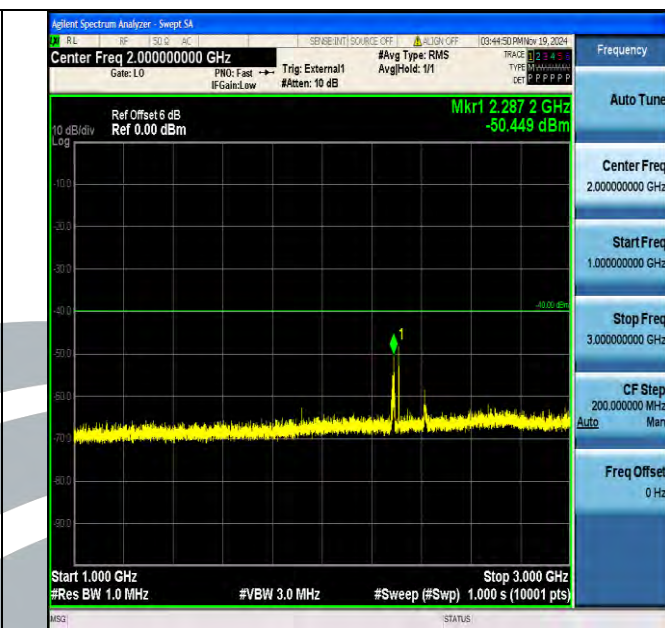
Band40_5MHz_16QAM_38750_1RB#0_1000~3000_1000~3000
