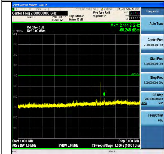
Band40_5MHz_16QAM_39175_1RB#0_1000~3000_1000~3000
