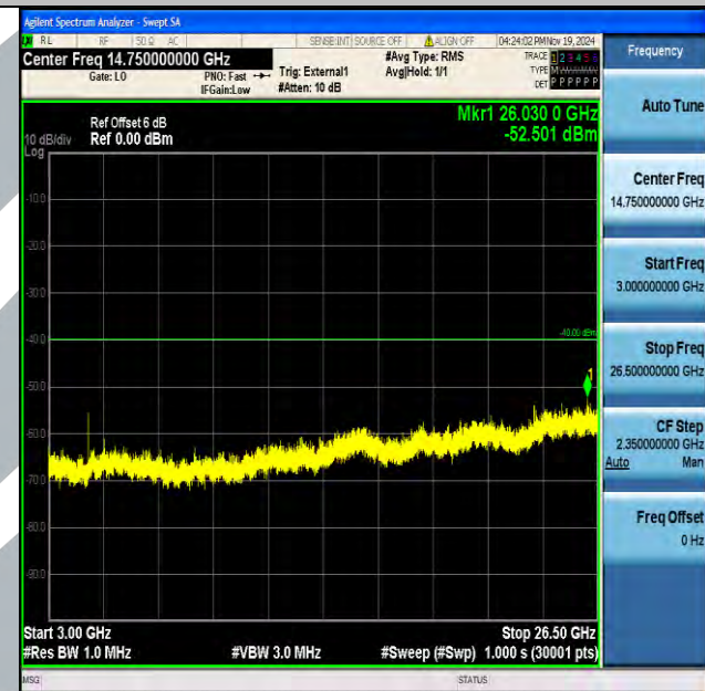
Band40_10MHz_16QAM_39200_1RB#0_3000~26500_3000~26500
