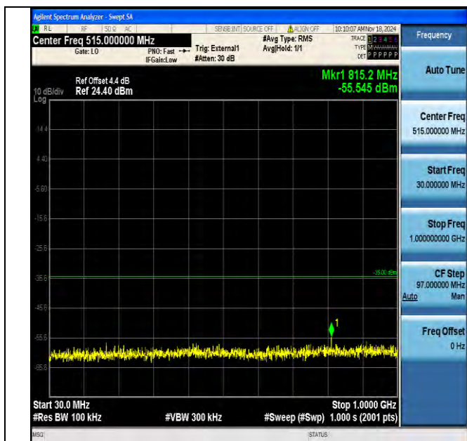
Band41 5MHz QPSK 40065 1RB#0 30~1000 30~1000
