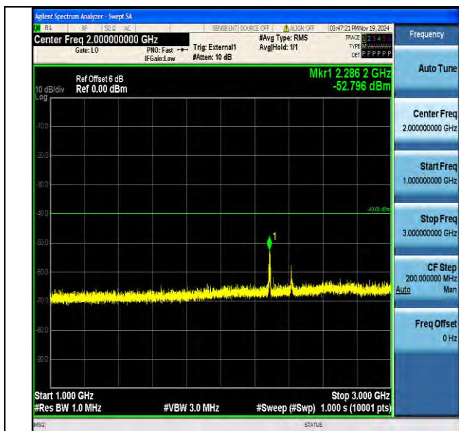
Band40_5MHz_16QAM_38775_1RB#0_1000~3000_1000~3000
