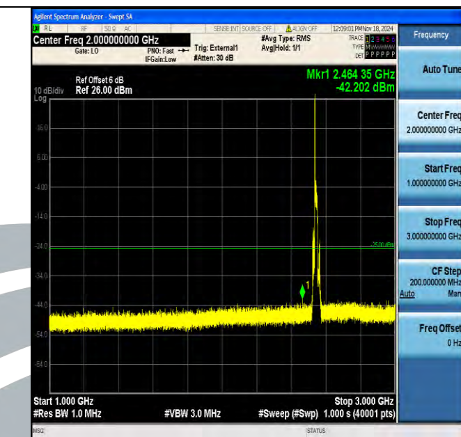
Band41_15MHz_16QAM_40115_1RB#0_1000~3000_1000~3000
