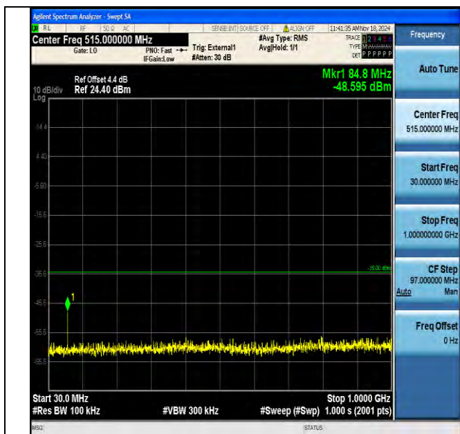
Band41_10MHz_16QAM_41190_1RB#0_30~1000_30~1000
