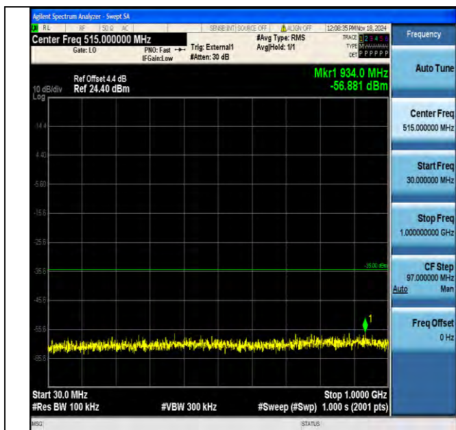
Band41_15MHz_16QAM_40115_1RB#0_30~1000_30~1000
