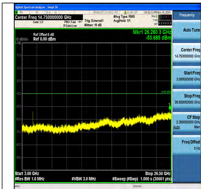
Band40_5MHz_QPSK_39225_1RB#0_3000~26500_3000~26500
