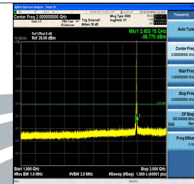
Band41 5MHz 16QAM 40590 1RB#0 1000~3000 1000~3000
