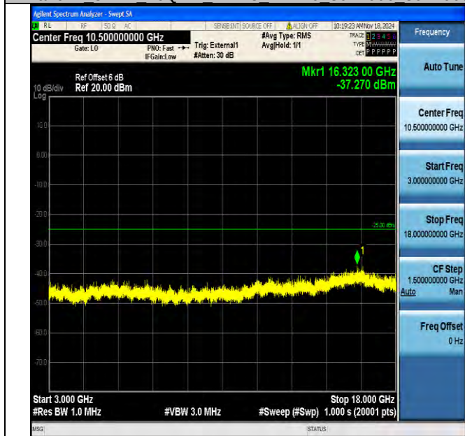
Band41_5MHz_16QAM_41215_1RB#0_3000~18000_3000~18000
