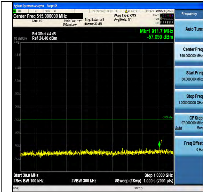
Band41 10MHz QPSK 40590 1RB#0 30~1000 30~1000
