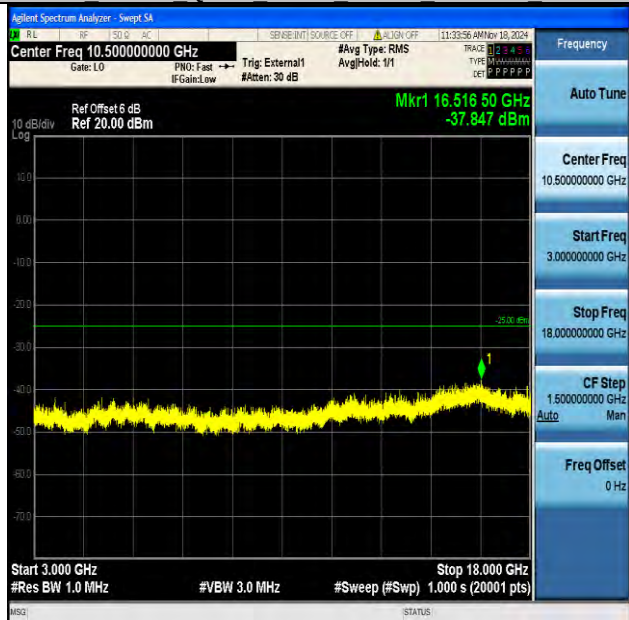
Band41_10MHz_QPSK_40090_1RB#0_3000~18000_3000~18000
