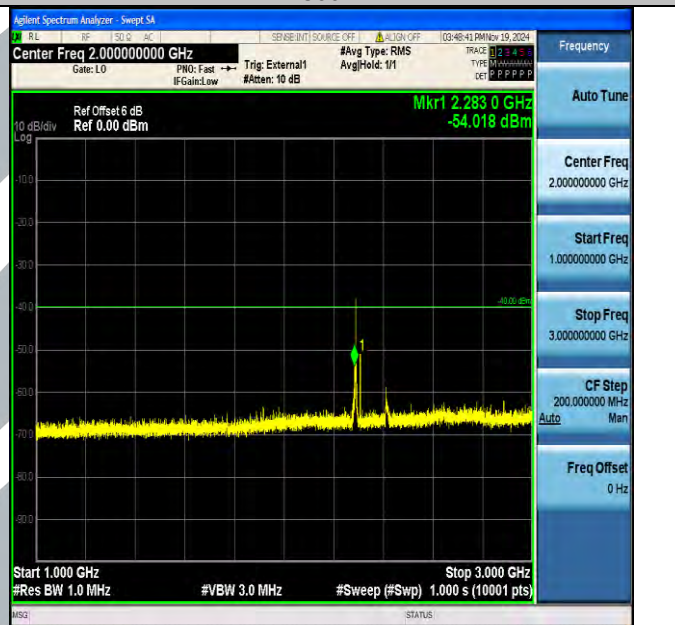
Band40_10MHz_QPSK_38750_1RB#0_1000~3000_1000~3000
