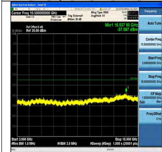
Band41_5MHz_16QAM_40590_1RB#0_3000~18000_3000~18000
