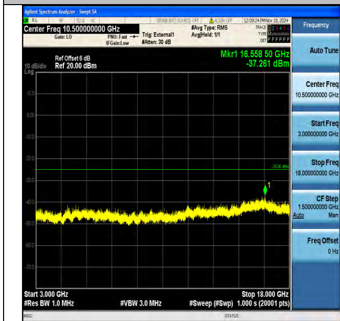
Band41_15MHz_16QAM_40115_1RB#0_3000~18000_3000~18000
