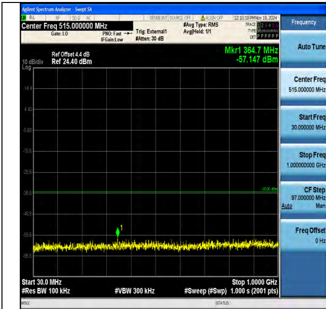
Band41 15MHz QPSK 40590 1RB#0 30~1000 30~1000
