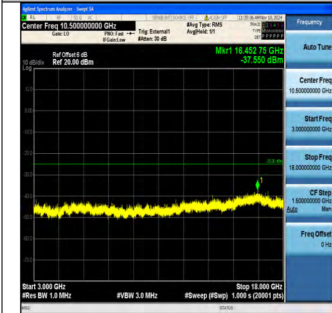
Band41_10MHz_16QAM_40090_1RB#0_3000~18000_3000~18000
