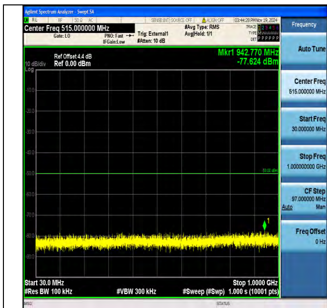
Band40_5MHz_16QAM_38750_1RB#0_30~1000_30~1000
