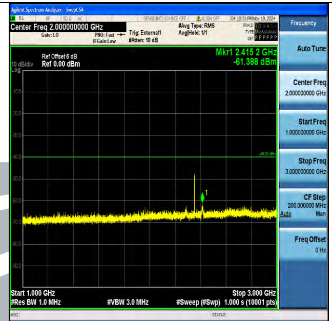
Band40_5MHz_16QAM_39200_1RB#0_1000~3000_1000~3000
