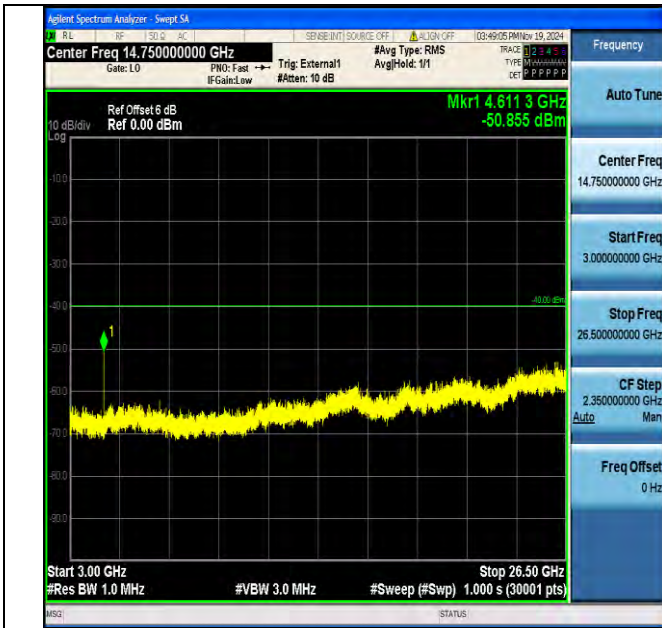
Band40_10MHz_QPSK_38750_1RB#0_3000~26500_3000~26500
