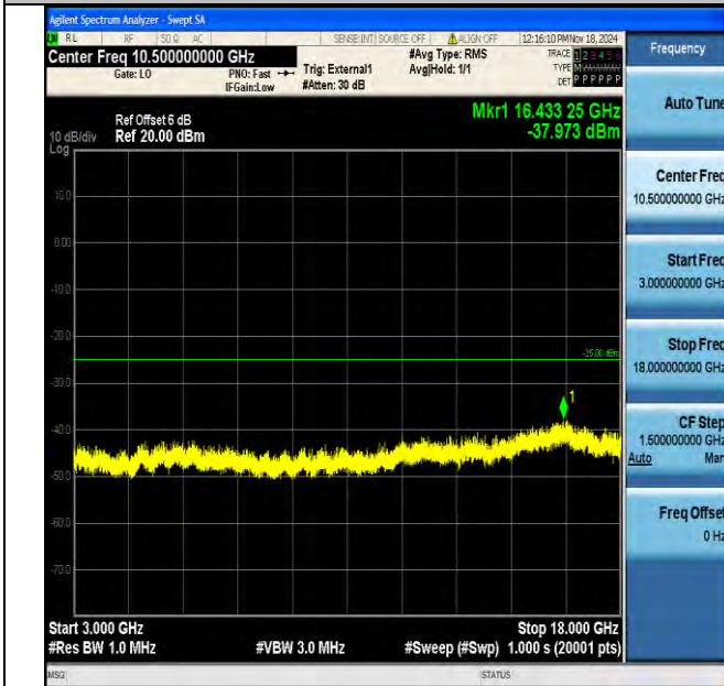
Band41_15MHz_16QAM_41165_1RB#0_3000~18000_3000~18000
