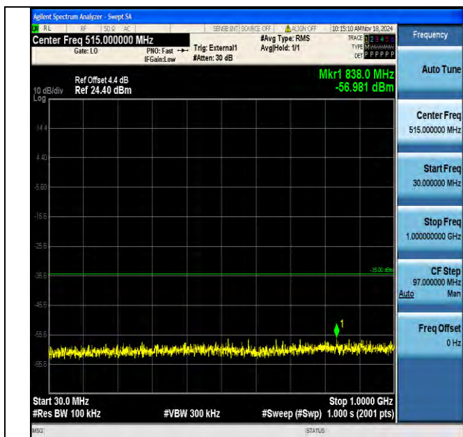
Band41 5MHz 16QAM 40590 1RB#0 30~1000 30~1000
