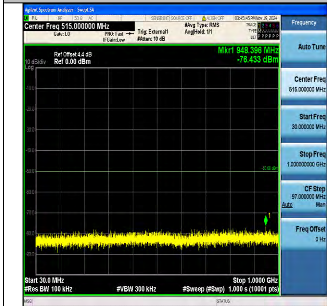
Band40_5MHz_QPSK_38775_1RB#0_30~1000_30~1000
