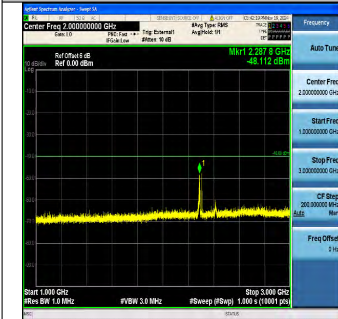
Band40_5MHz_16QAM_38725_1RB#0_1000~3000_1000~3000
