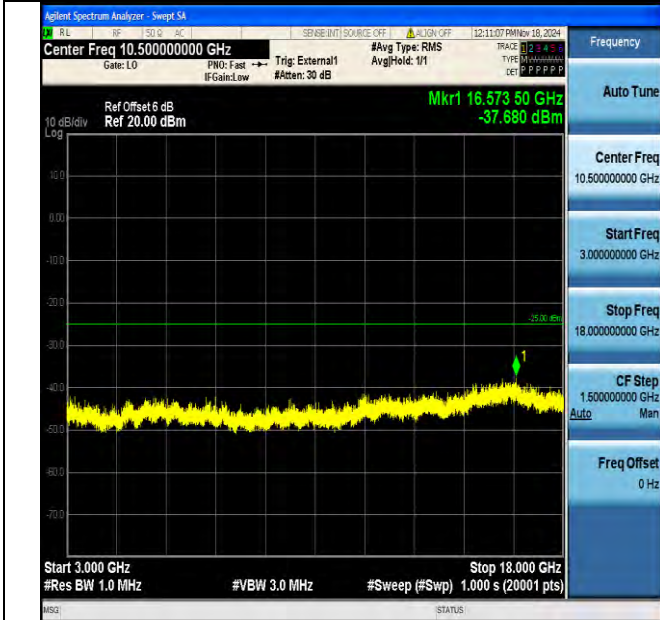
Band41_15MHz_QPSK_40590_1RB#0_3000~18000_3000~18000
