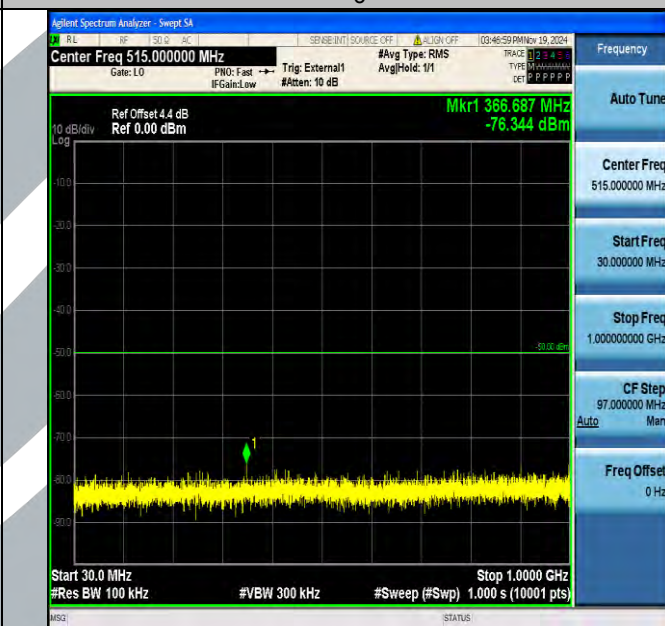
Band40_5MHz_16QAM_38775_1RB#0_30~1000_30~1000
