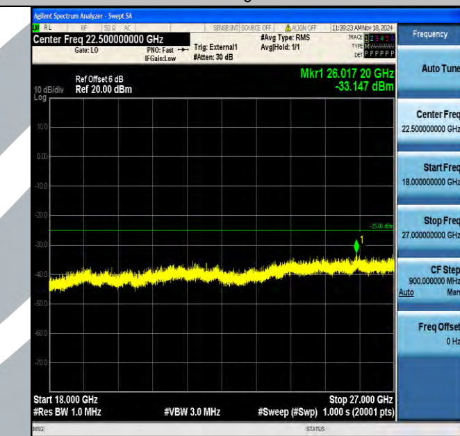
Band41_10MHz_16QAM_40590_1RB#0_18000~27000_18000~27000
