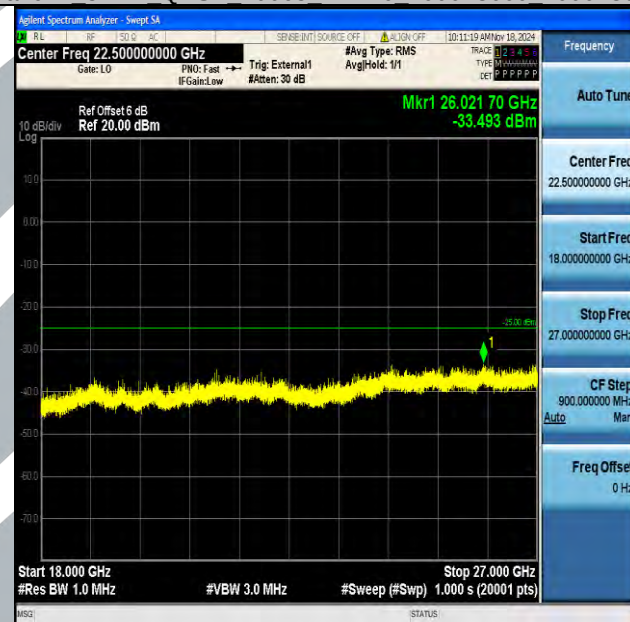
Band41_5MHz_QPSK_40065_1RB#0_18000~27000_18000~27000
