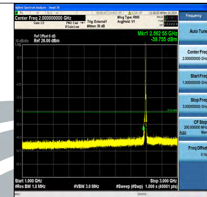
Band41_10MHz_16QAM_40590_1RB#0_1000~3000_1000~3000
