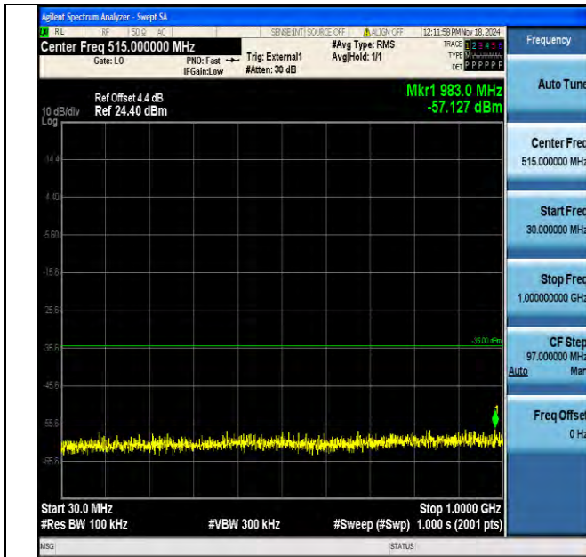
Band41_15MHz_16QAM_40590_1RB#0_30~1000_30~1000
