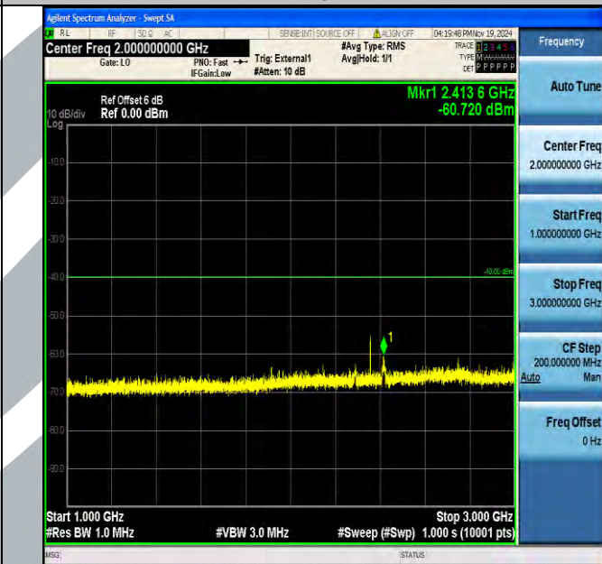
Band40_5MHz_QPSK_39225_1RB#0_1000~3000_1000~3000
