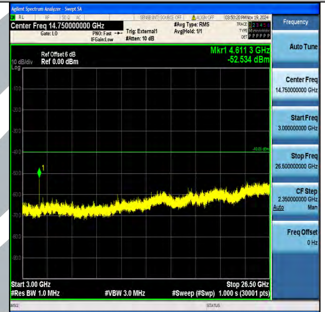
Band40_10MHz_16QAM_38750_1RB#0_3000~26500_3000~26500
