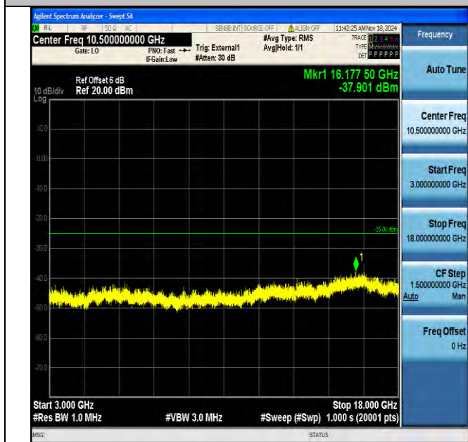
Band41_10MHz_16QAM_41190_1RB#0_3000~18000_3000~18000
