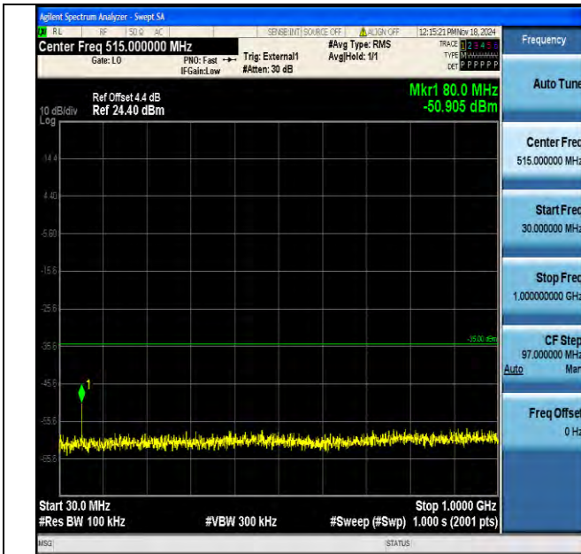
Band41_15MHz_16QAM_41165_1RB#0_30~1000_30~1000
