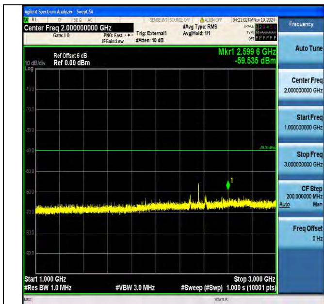
Band40_5MHz_16QAM_39225_1RB#0_1000~3000_1000~3000
