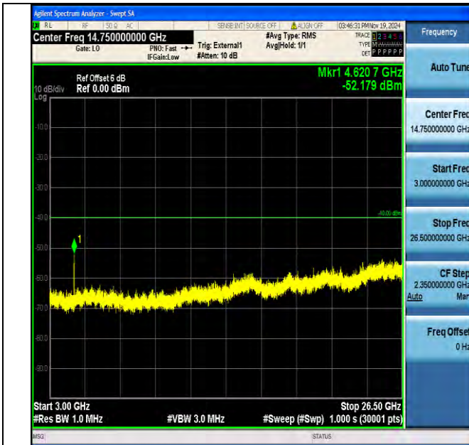
Band40_5MHz_QPSK_38775_1RB#0_3000~26500_3000~26500
