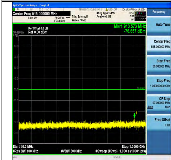
Band40_5MHz_QPSK_39225_1RB#0_30~1000_30~1000
