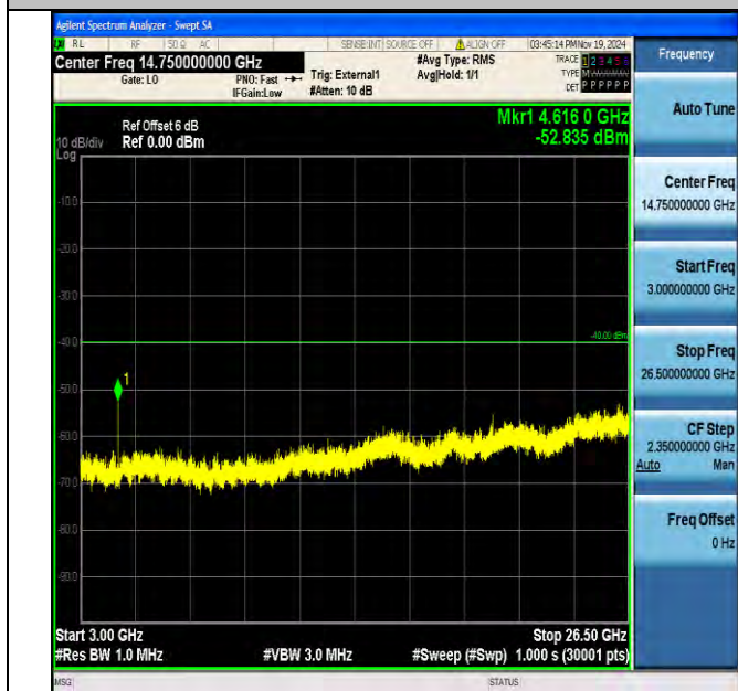
Band40_5MHz_16QAM_38750_1RB#0_3000~26500_3000~26500
