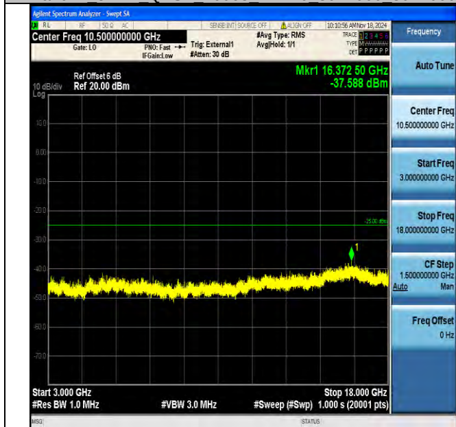
Band41_5MHz_QPSK_40065_1RB#0_3000~18000_3000~18000
