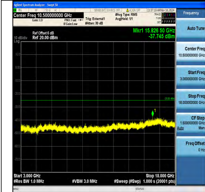
Band41_10MHz_QPSK_40590_1RB#0_3000~18000_3000~18000
