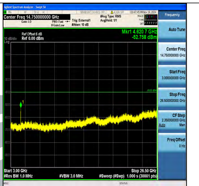
Band40_5MHz_16QAM_38775_1RB#0_3000~26500_3000~26500
