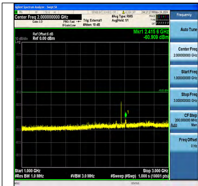
Band40_5MHz_QPSK_39200_1RB#0_1000~3000_1000~3000
