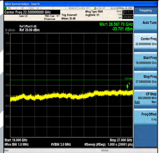
Band41_15MHz_QPSK_40590_1RB#0_18000~27000_18000~27000
