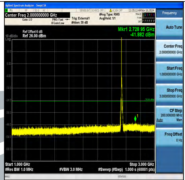
Band41_10MHz_16QAM_40090_1RB#0_1000~3000_1000~3000
