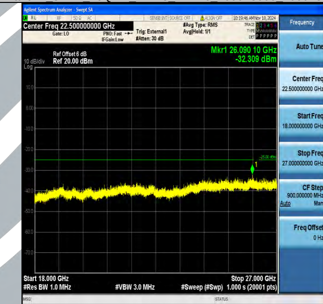
Band41_5MHz_16QAM_41215_1RB#0_18000~27000_18000~27000
