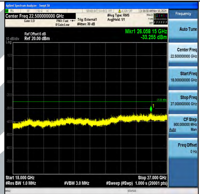
Band41_10MHz_16QAM_40090_1RB#0_18000~27000_18000~27000
