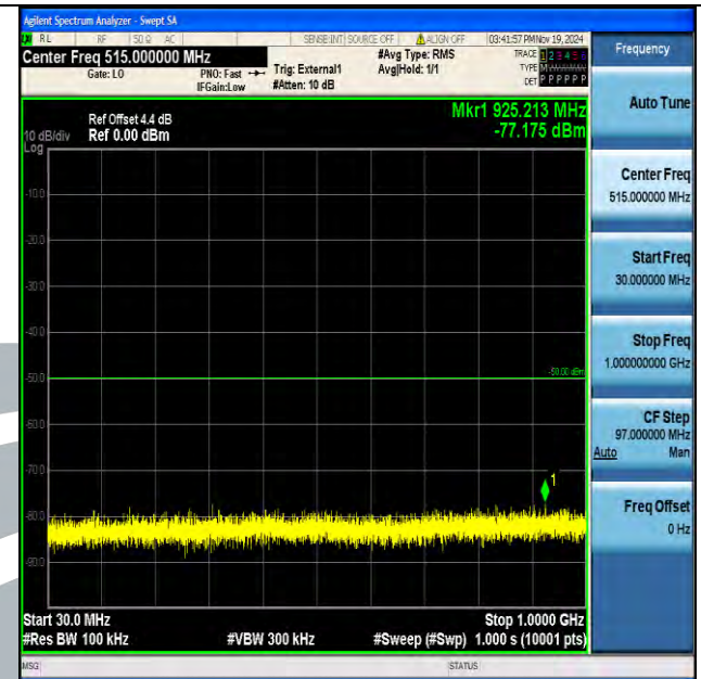
Band40_5MHz_16QAM_38725_1RB#0_30~1000_30~1000
