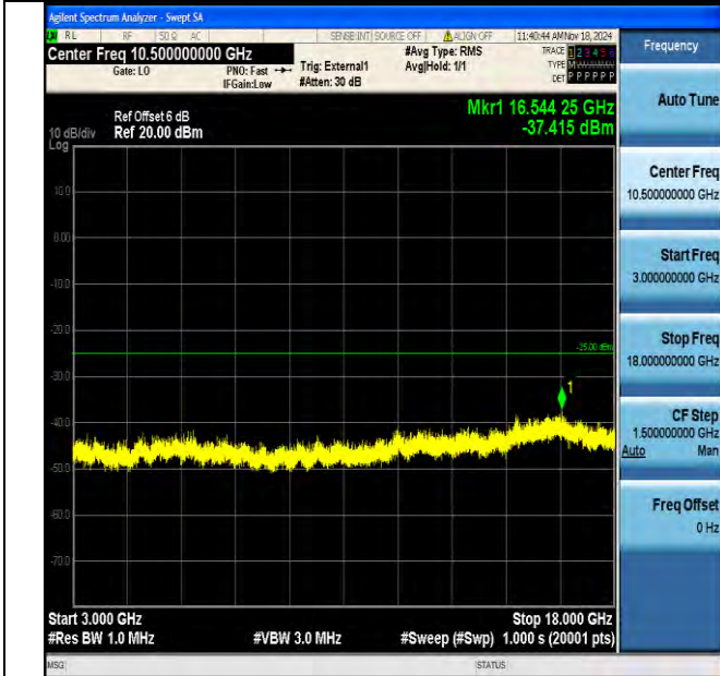
Band41_10MHz_QPSK_41190_1RB#0_3000~18000_3000~18000
