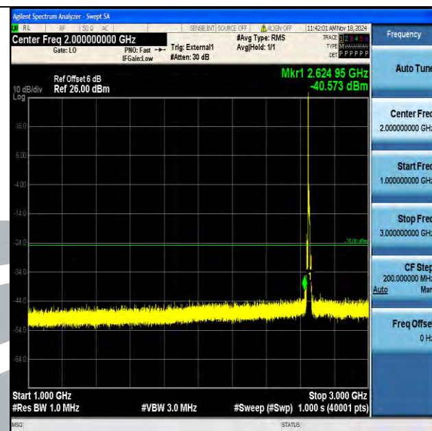
Band41_10MHz_16QAM_41190_1RB#0_1000~3000_1000~3000
