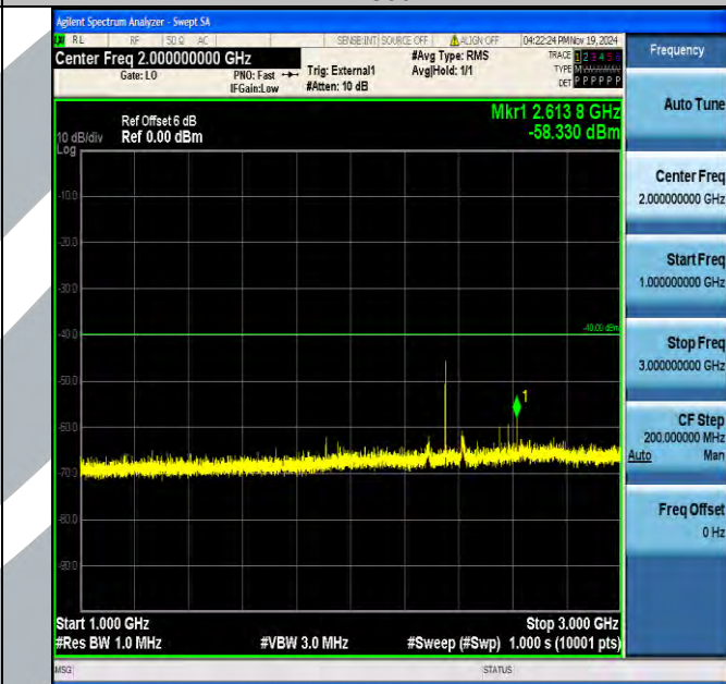
Band40_10MHz_QPSK_39200_1RB#0_1000~3000_1000~3000
