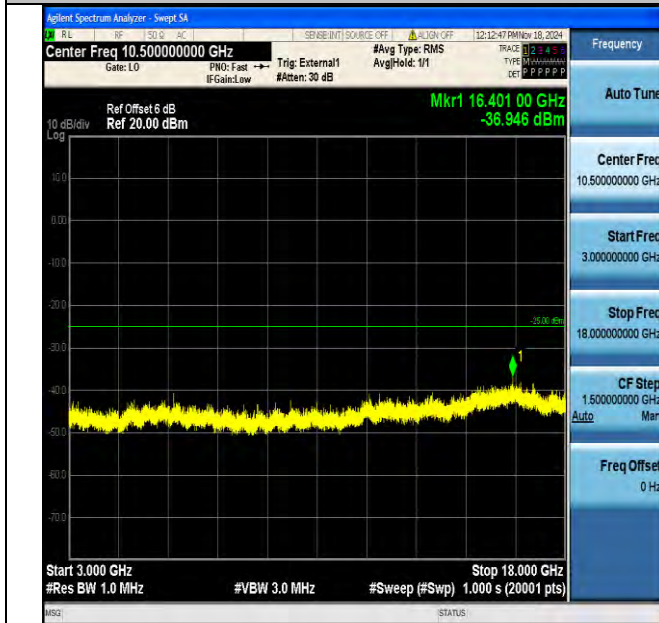
Band41_15MHz_16QAM_40590_1RB#0_3000~18000_3000~18000
