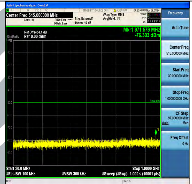
Band40_5MHz_16QAM_39225_1RB#0_30~1000_30~1000
