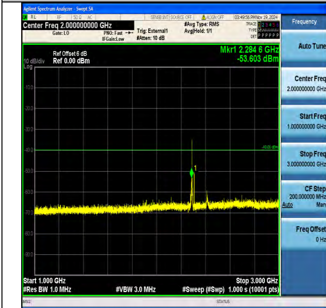
Band40_10MHz_16QAM_38750_1RB#0_1000~3000_1000~3000
