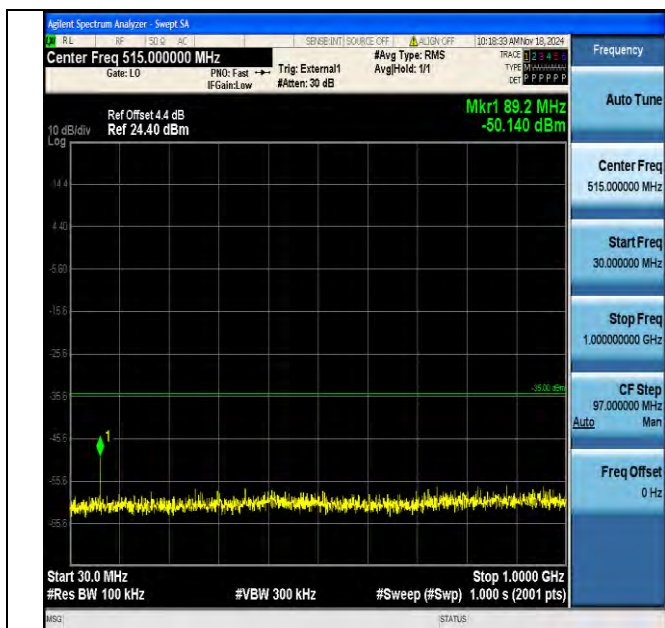
Band41 5MHz 16QAM 41215 1RB#0 30~1000 30~1000
