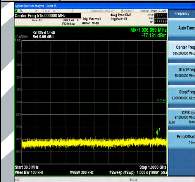
Band40_5MHz_QPSK_38750_1RB#0_30~1000_30~1000
