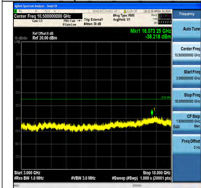
Band41_5MHz_16QAM_40065_1RB#0_3000~18000_3000~18000
