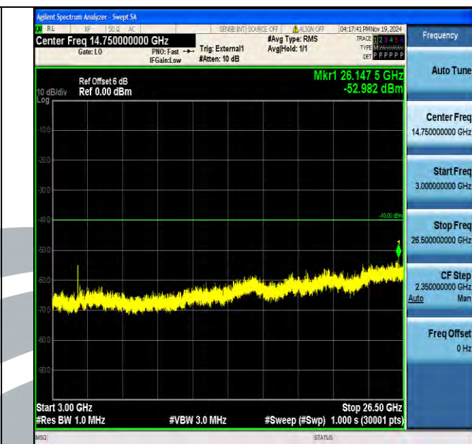
Band40_5MHz_QPSK_39200_1RB#0_3000~26500_3000~26500
