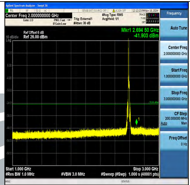
Band41_15MHz_16QAM_40590_1RB#0_1000~3000_1000~3000
