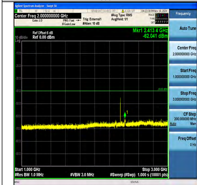
Band40_10MHz_16QAM_39200_1RB#0_1000~3000_1000~3000
