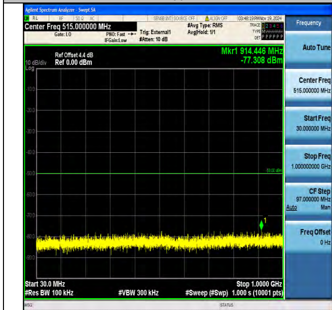
Band40_10MHz_QPSK_38750_1RB#0_30~1000_30~1000
