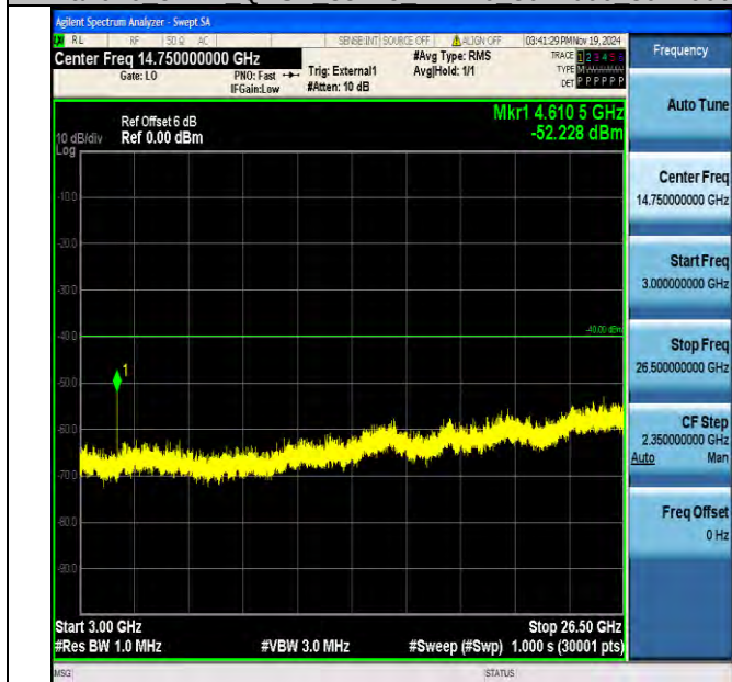
Band40_5MHz_QPSK_38725_1RB#0_3000~26500_3000~26500
