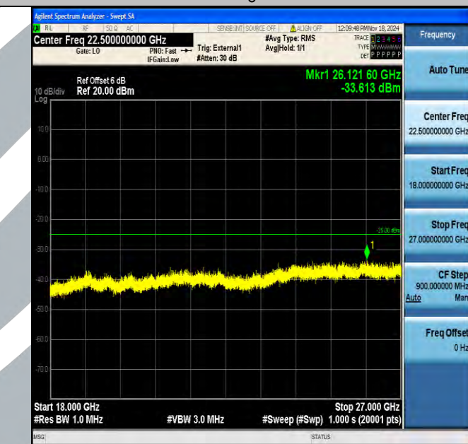
Band41_15MHz_16QAM_40115_1RB#0_18000~27000_18000~27000
