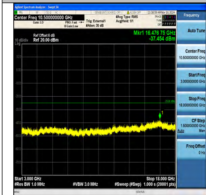
Band41_10MHz_16QAM_40590_1RB#0_3000~18000_3000~18000
