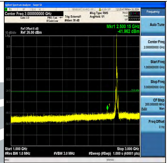
Band41_15MHz_16QAM_41165_1RB#0_1000~3000_1000~3000
