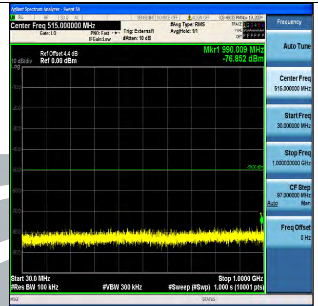
Band40_10MHz_16QAM_38750_1RB#0_30~1000_30~1000
