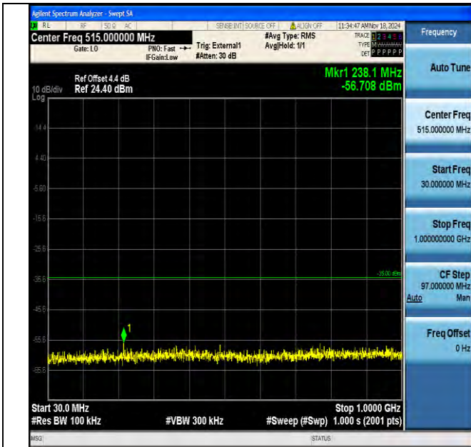
Band41_10MHz_16QAM_40090_1RB#0_30~1000_30~1000
