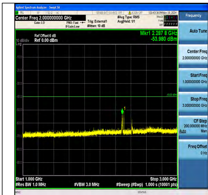
Band40_5MHz_QPSK_38750_1RB#0_1000~3000_1000~3000
