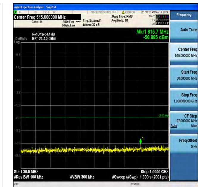
Band41_10MHz_16QAM_40590_1RB#0_30~1000_30~1000
