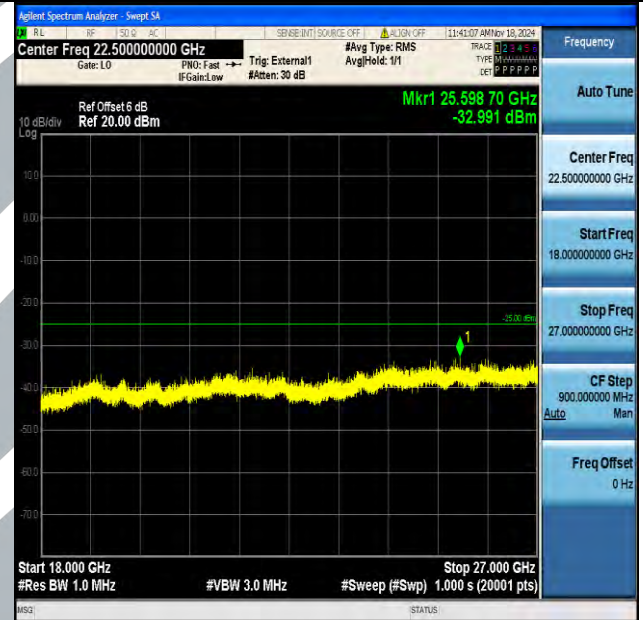
Band41_10MHz_QPSK_41190_1RB#0_18000~27000_18000~27000
