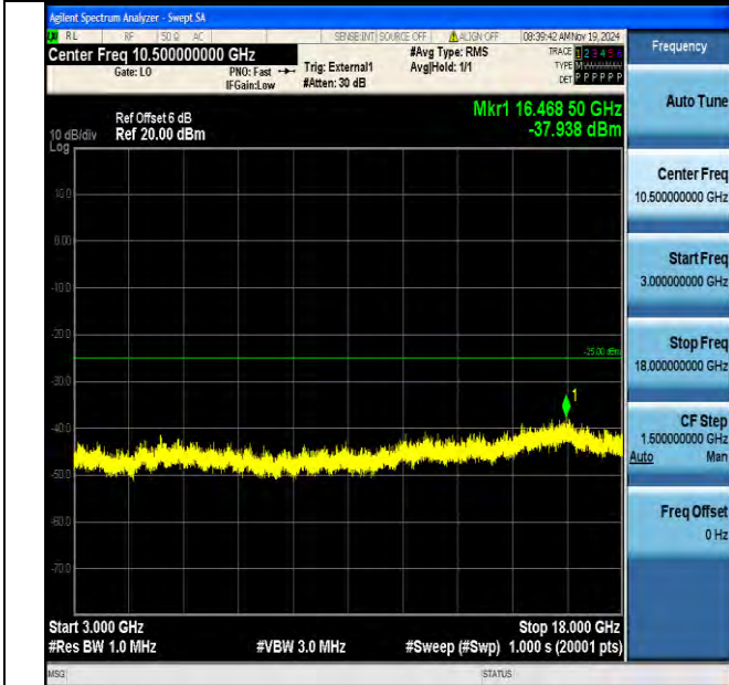
Band38_5MHz_QPSK_38225_1RB#0_3000~18000_3000~18000
