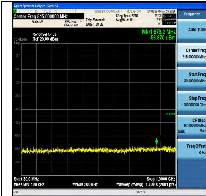
Band38_10MHz_16QAM_37800_1RB#0_30~1000_30~1000
