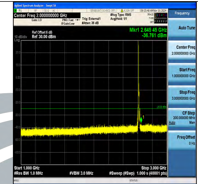
Band38_10MHz_16QAM_38200_1RB#0_1000~3000_1000~3000 0
