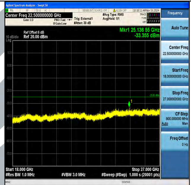
Band38_20MHz_16QAM_37850_1RB#0_18000~27000_18000~27000
