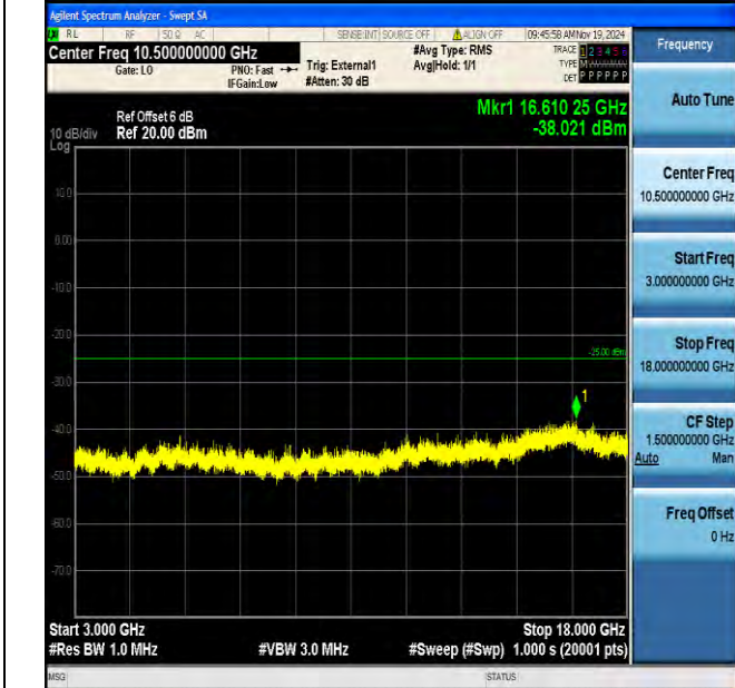
Band38_15MHz_QPSK_38000_1RB#0_3000~18000_3000~18000
