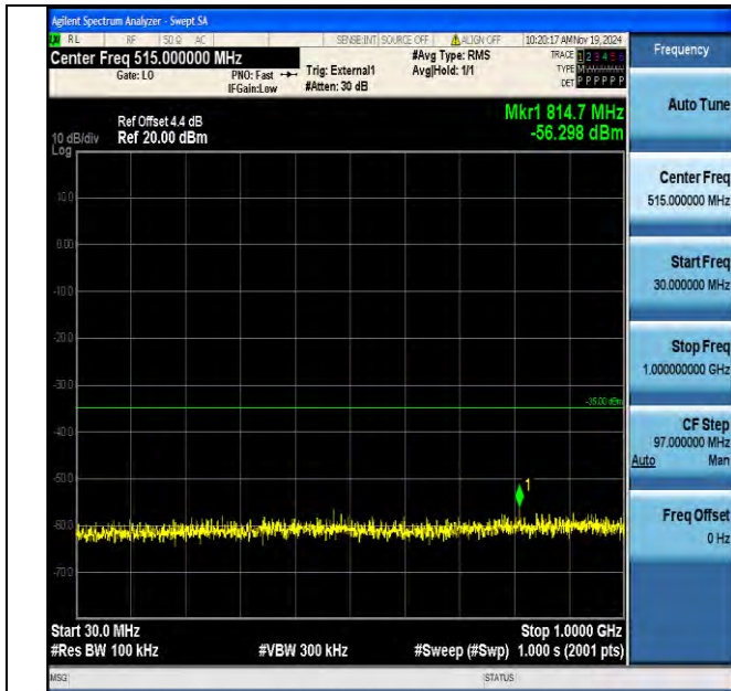
Band38_20MHz_16QAM_38000_1RB#0_30~1000_30~1000
