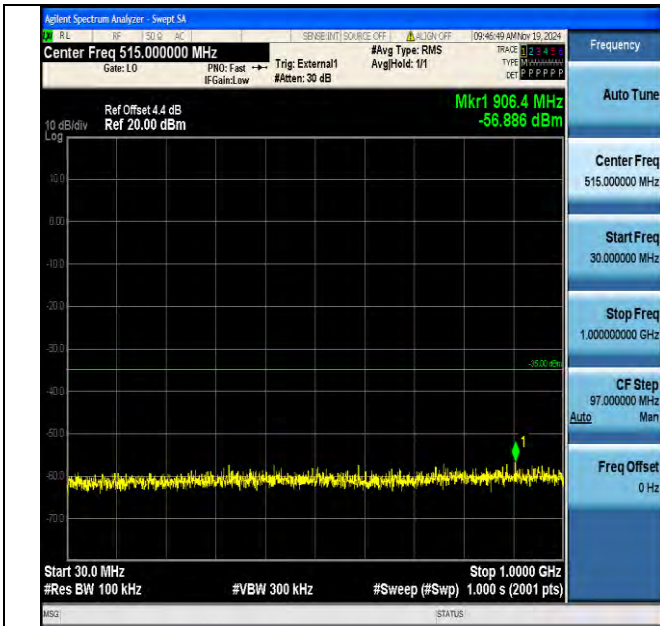
Band38_15MHz_16QAM_38000_1RB#0_30~1000_30~1000
