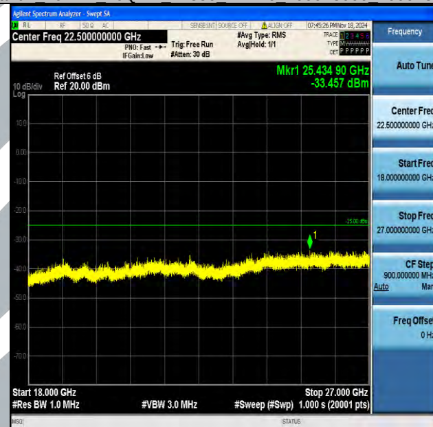
Band7_20MHz_16QAM_21350_1RB#0_18000~27000_18000~27000
