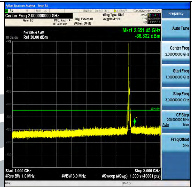
Band38_15MHz_16QAM_37825_1RB#0_1000~3000_1000~3000
