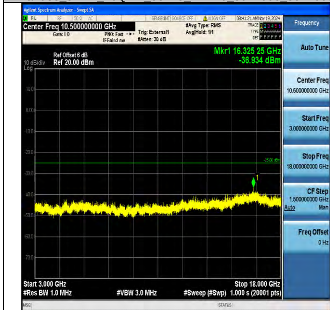
Band38_5MHz_16QAM_38225_1RB#0_3000~18000_3000~18000
