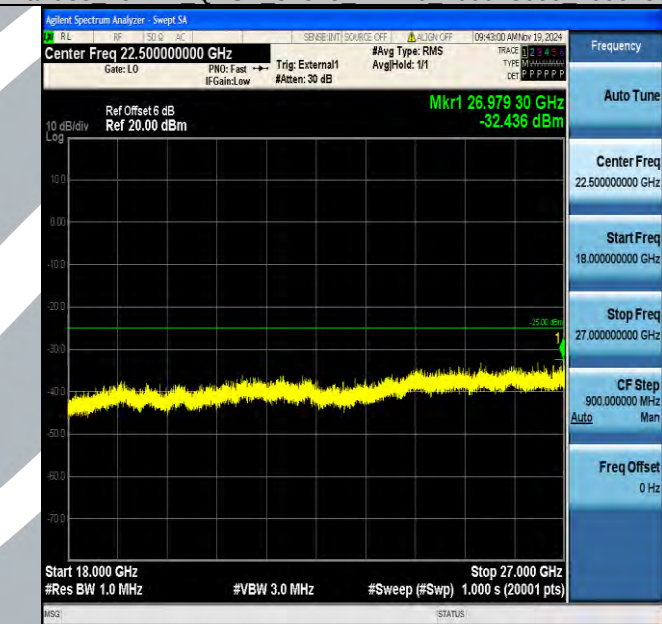
Band38_15MHz_QPSK_37825_1RB#0_18000~27000_18000~27000
