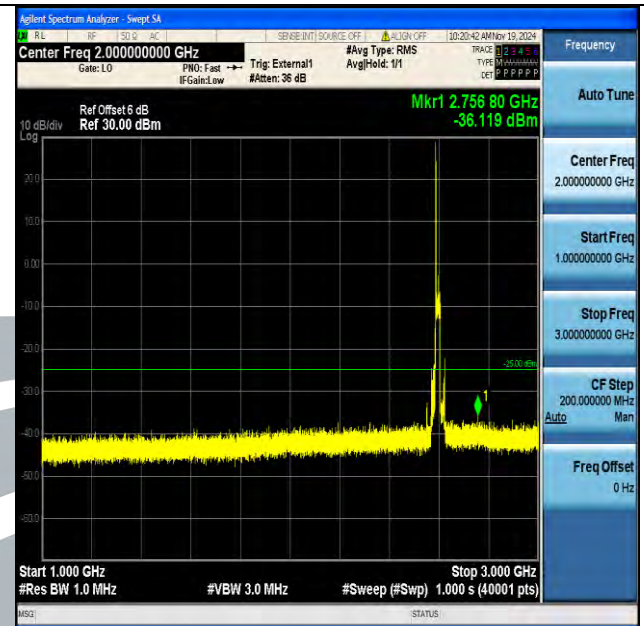
Band38_20MHz_16QAM_38000_1RB#0_1000~3000_1000~3000
