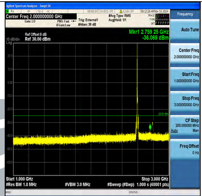
Band38_10MHz_16QAM_38000_1RB#0_1000~3000_1000~3000
