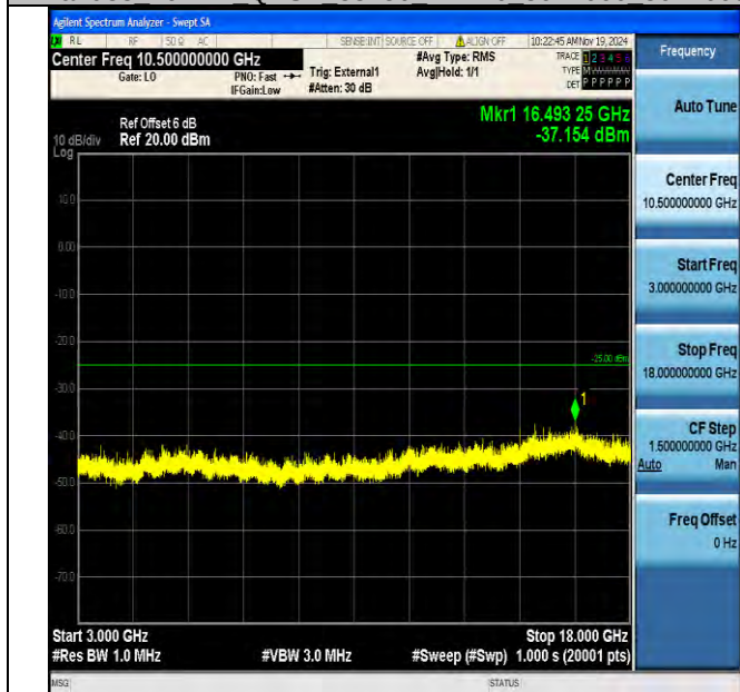
Band38_20MHz_QPSK_38150_1RB#0_3000~18000_3000~18000
