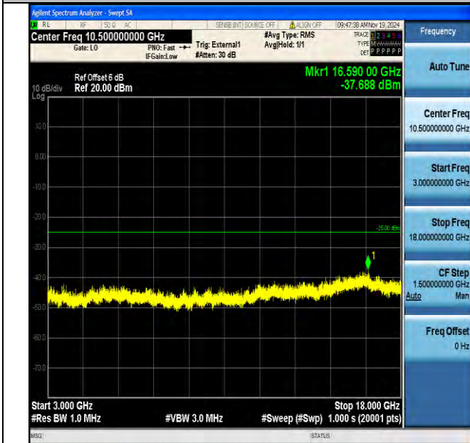
Band38_15MHz_16QAM_38000_1RB#0_3000~18000_3000~18000
