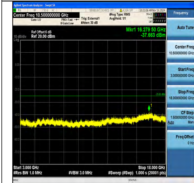
Band38_20MHz_16QAM_38000_1RB#0_3000~18000_3000~18000
