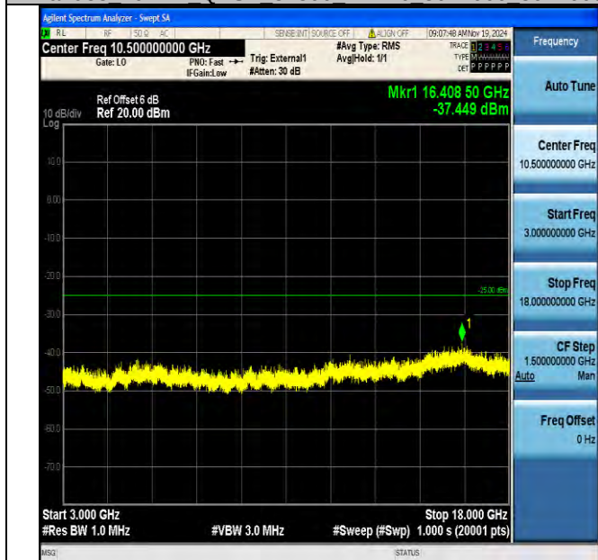
Band38_10MHz_QPSK_37800_1RB#0_3000~18000_3000~18000
