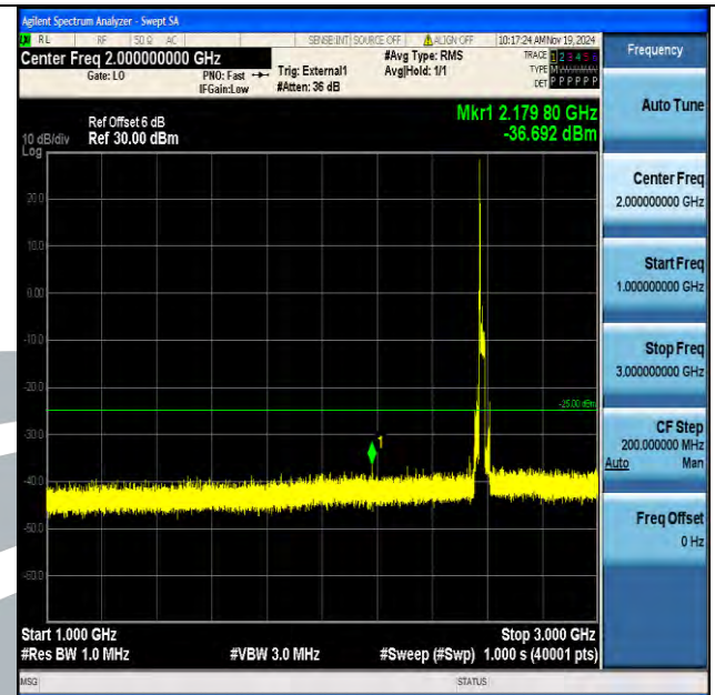
Band38_20MHz_16QAM_37850_1RB#0_1000~3000_1000~3000
