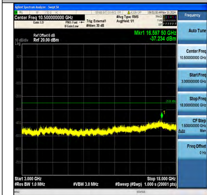
Band38_15MHz_16QAM_38175_1RB#0_3000~18000_3000~18000
