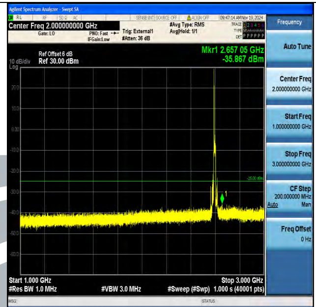
Band38_15MHz_16QAM_38000_1RB#0_1000~3000_1000~3000
