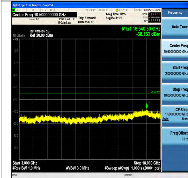
Band38_10MHz_16QAM_38200_1RB#0_3000~18000_3000~18000
