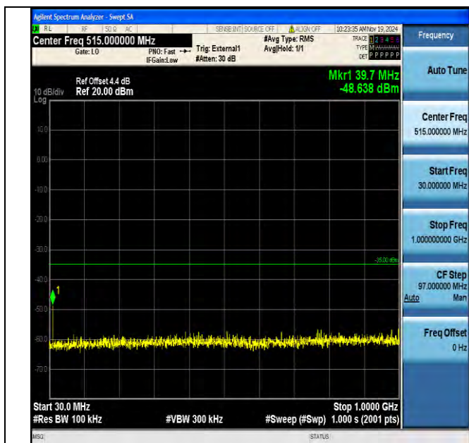
Band38_20MHz_16QAM_38150_1RB#0_30~1000_30~1000
