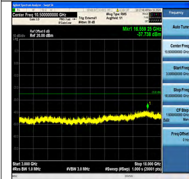
Band38_20MHz_16QAM_37850_1RB#0_3000~18000_3000~18000
