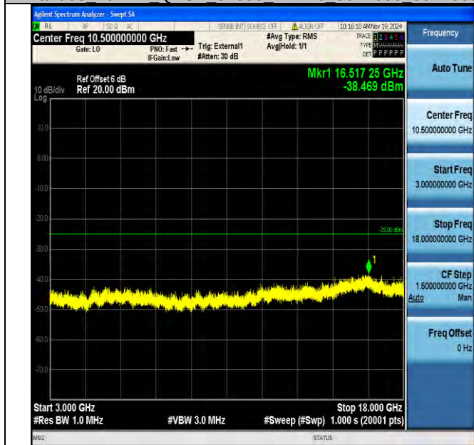
Band38_20MHz_QPSK_37850_1RB#0_3000~18000_3000~18000
