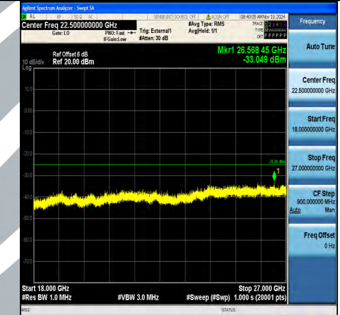
Band38_5MHz_QPSK_38225_1RB#0_18000~27000_18000~27000
