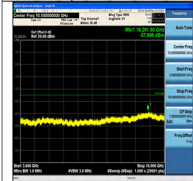
Band38_5MHz_16QAM_37775_1RB#0_3000~18000_3000~18000
