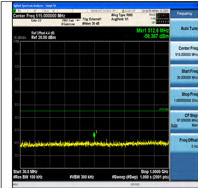
Band38_20MHz_16QAM_37850_1RB#0_30~1000_30~1000
