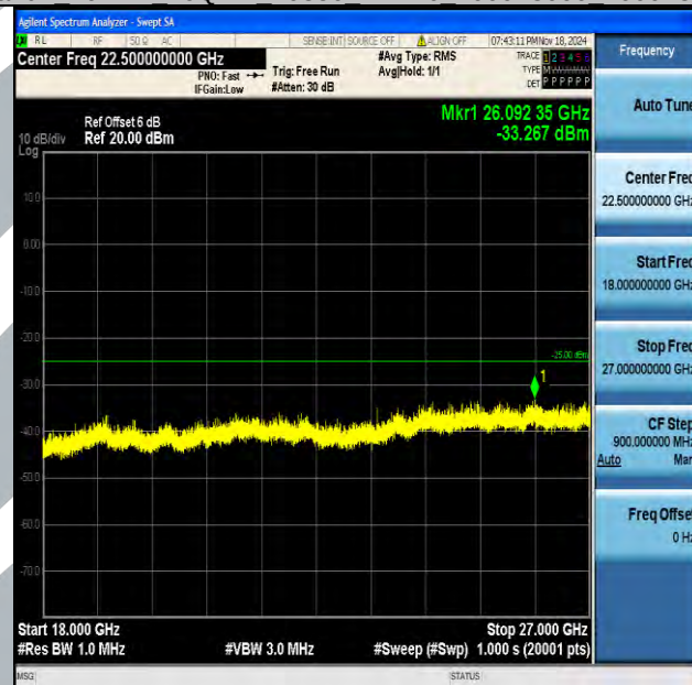
Band7_20MHz_16QAM_20850_1RB#0_18000~27000_18000~27000
