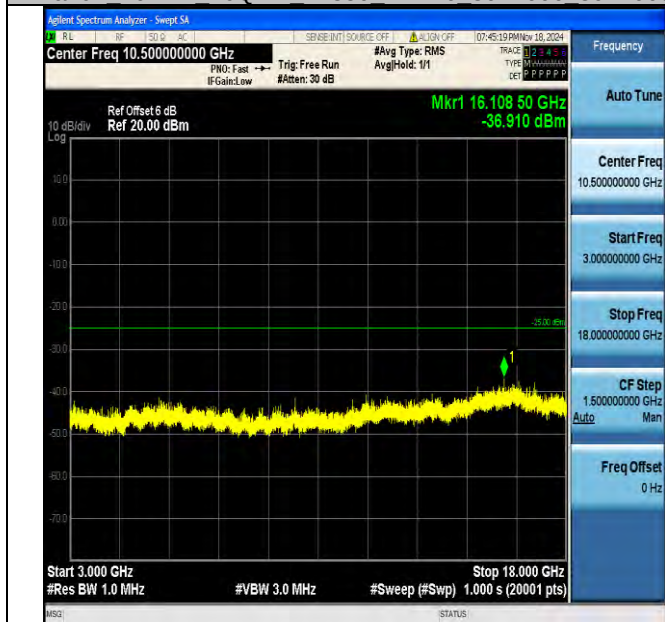
Band7_20MHz_16QAM_21350_1RB#0_3000~18000_3000~18000
