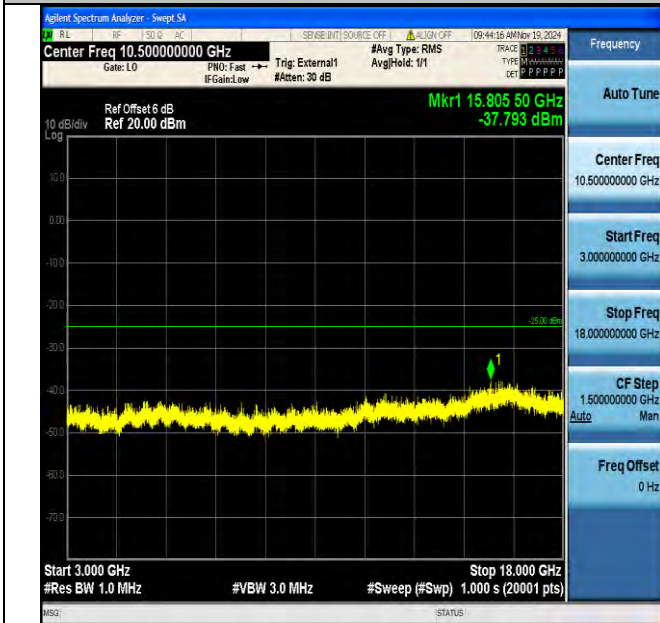
Band38_15MHz_16QAM_37825_1RB#0_3000~18000_3000~18000
