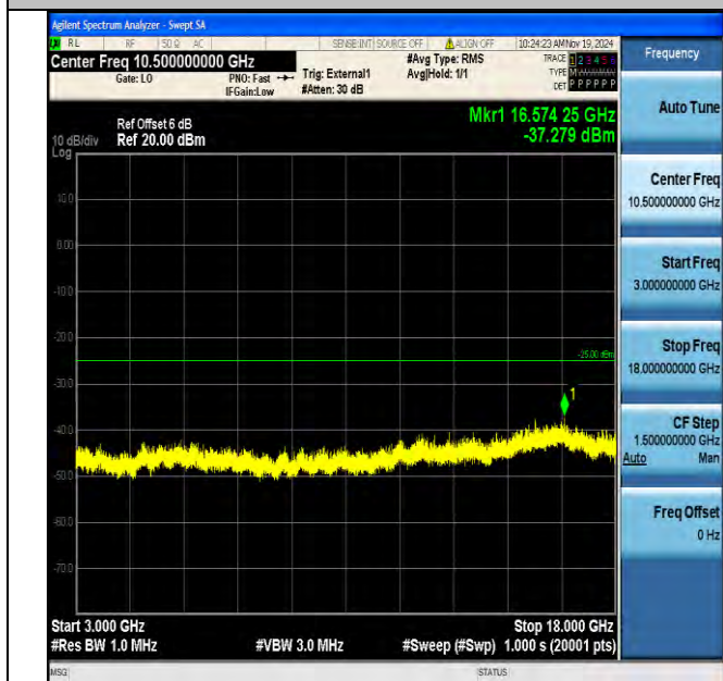
Band38_20MHz_16QAM_38150_1RB#0_3000~18000_3000~18000
