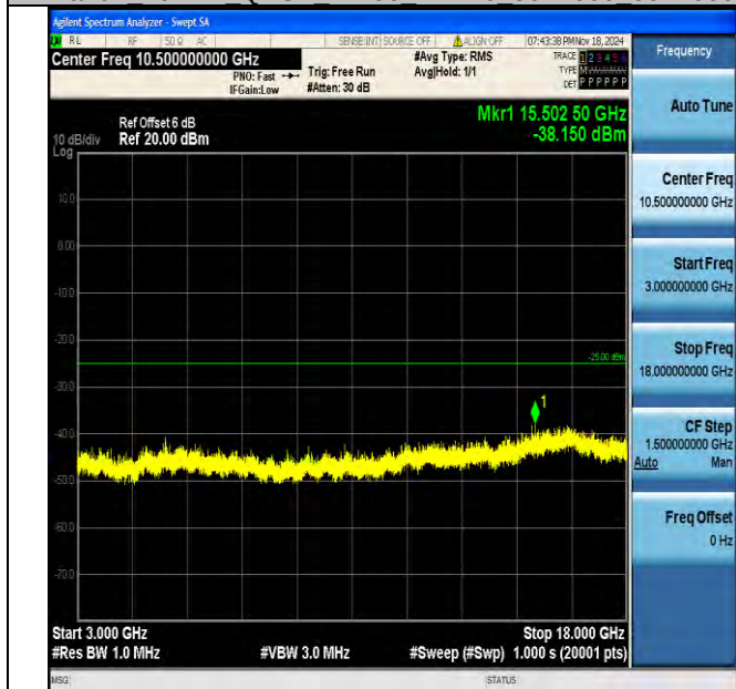
Band7_20MHz_QPSK_21100_1RB#0_3000~18000_3000~18000
