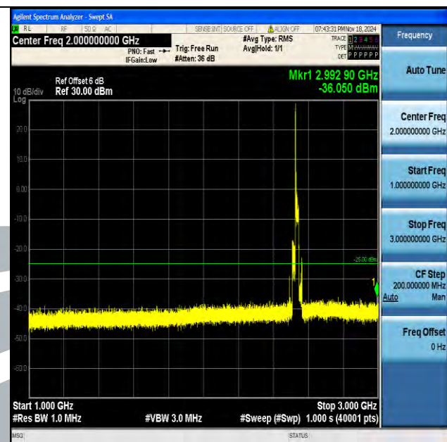
Band7_20MHz_QPSK_21100_1RB#0_1000~3000_1000~3000
