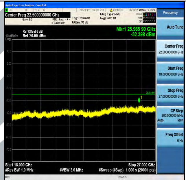
Band38_10MHz_16QAM_37800_1RB#0_18000~27000_18000~27000
