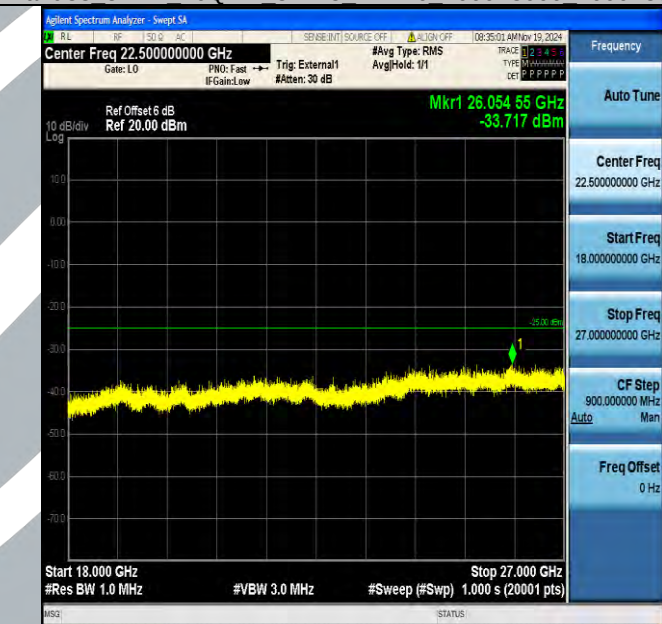
Band38_5MHz_16QAM_37775_1RB#0_18000~27000_18000~27000
