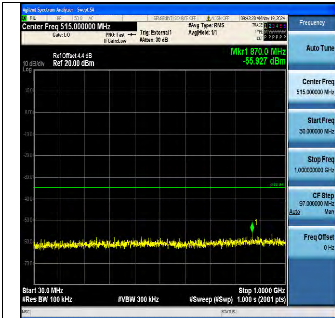
Band38_15MHz_16QAM_37825_1RB#0_30~1000_30~1000
