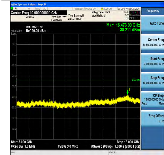
Band38_10MHz_16QAM_38000_1RB#0_3000~18000_3000~18000
