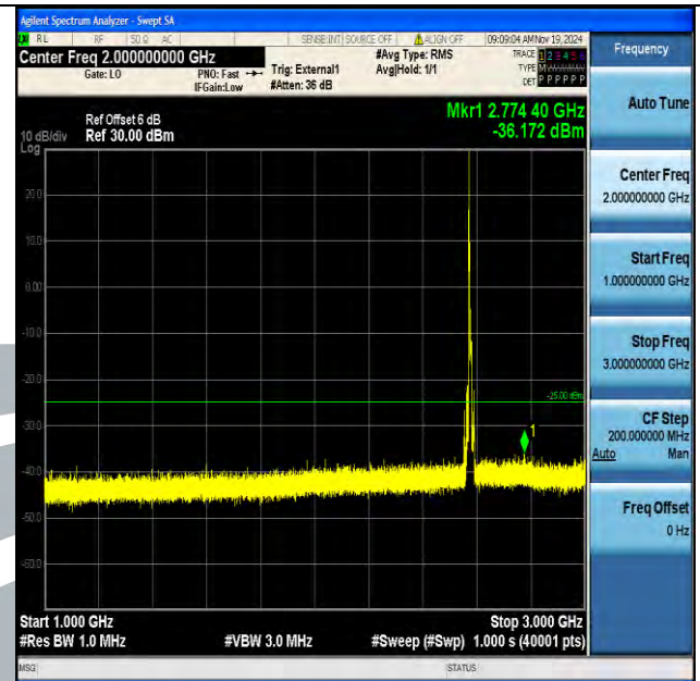
Band38_10MHz_16QAM_37800_1RB#0_1000~3000_1000~3000
