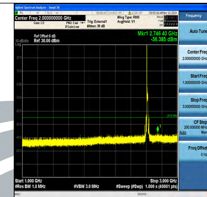
Band38_15MHz_16QAM_38175_1RB#0_1000~3000_1000~3000
