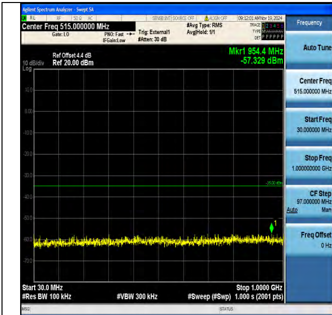
Band38_10MHz_16QAM_38000_1RB#0_30~1000_30~1000
