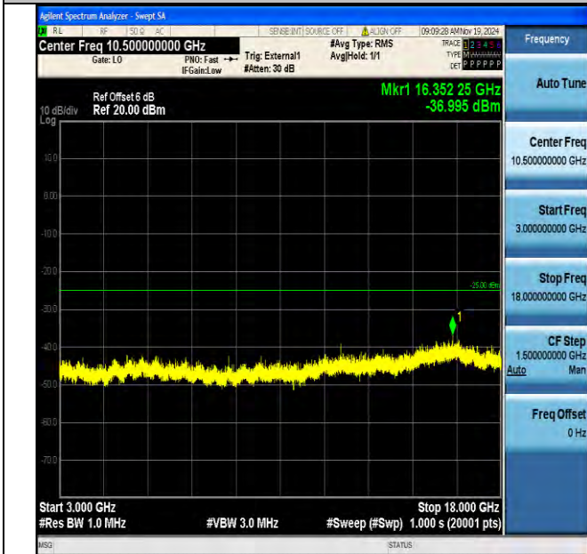
Band38_10MHz_16QAM_37800_1RB#0_3000~18000_3000~18000
