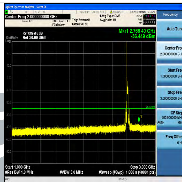
Band38_20MHz_16QAM_38150_1RB#0_1000~3000_1000~3000
