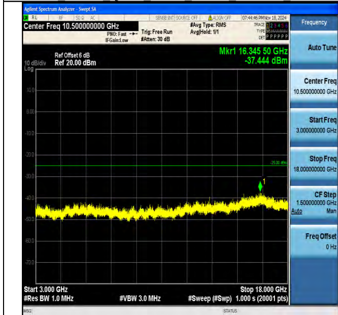
Band7_20MHz_QPSK_21350_1RB#0_3000~18000_3000~18000
