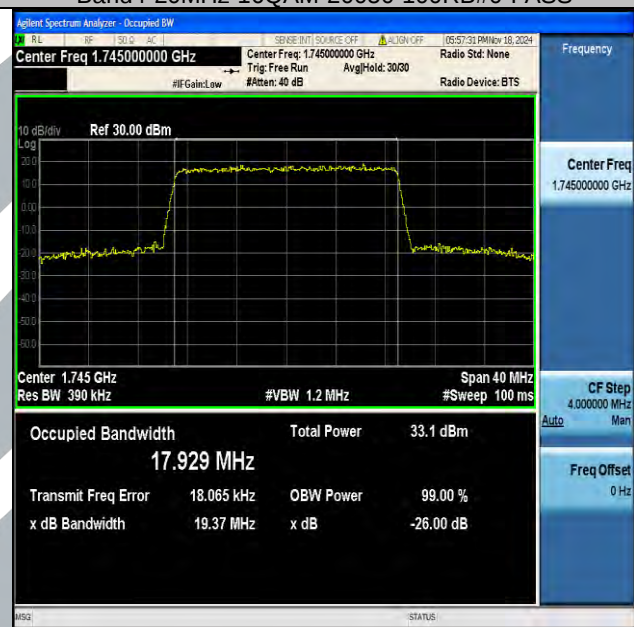
Band4-20MHz-16QAM-20300-100RB#0-PASS
