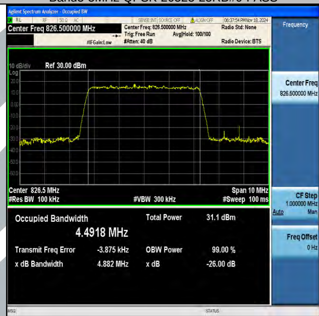
Band5-5MHz-16QAM-20425-25RB#0-PASS
