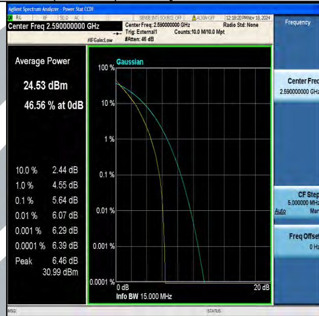
Band41(2535-2655)-15MHz-QPSK-40590-75RB#0-PASS
