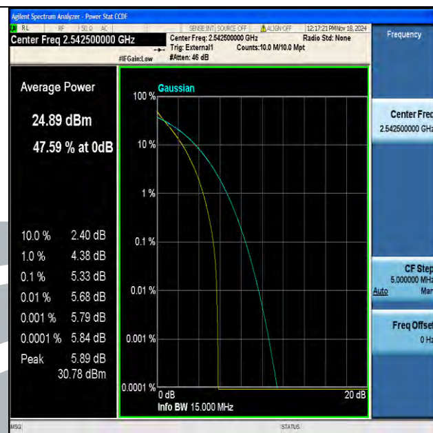
Band41(2535-2655)-15MHz-QPSK-40115-75RB#0-PASS
