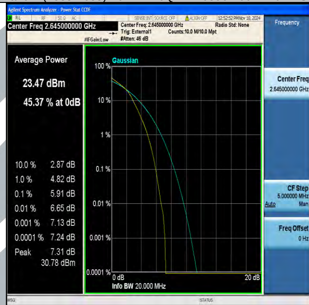
Band41(2535-2655)-20MHz-16QAM-41140-100RB#0-PASS
