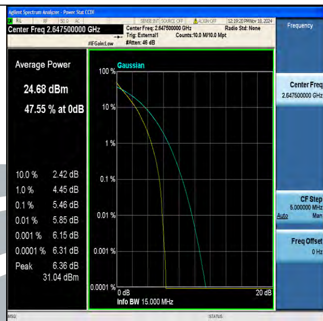
Band41(2535-2655)-15MHz-QPSK-41165-75RB#0-PASS
