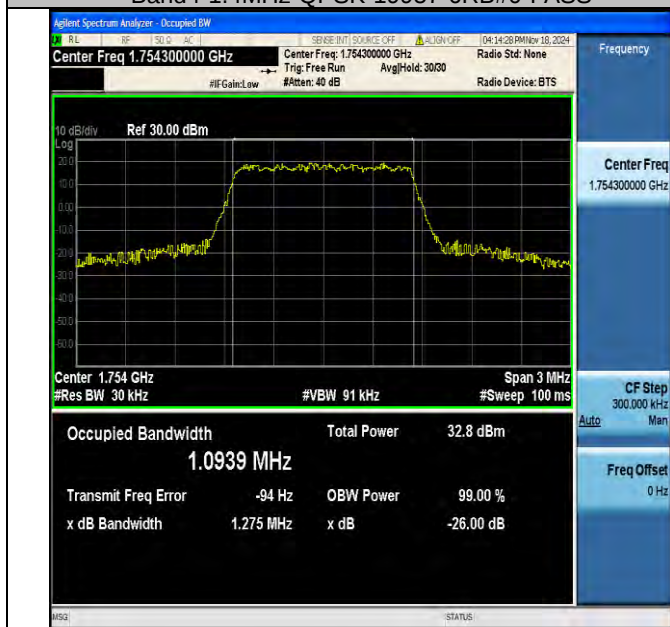
Band4-1.4MHz-QPSK-20393-6RB#0-PASS
