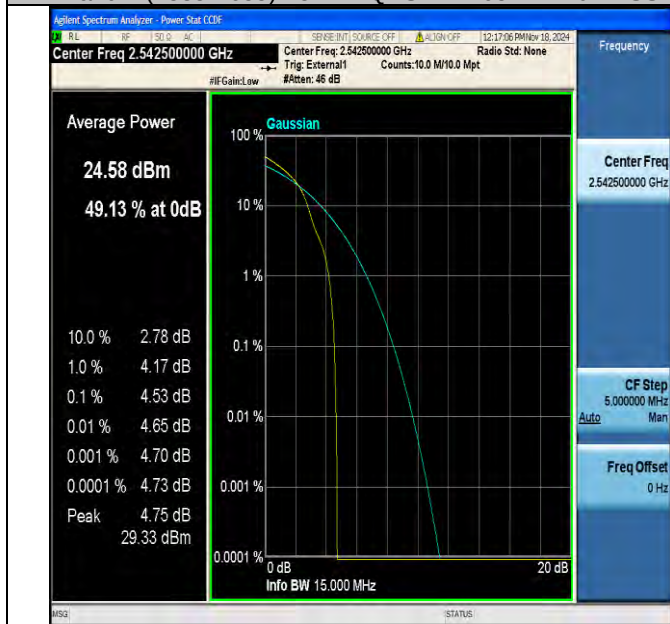
Band41(2535-2655)-15MHz-16QAM-40115-1RB#0-PASS
