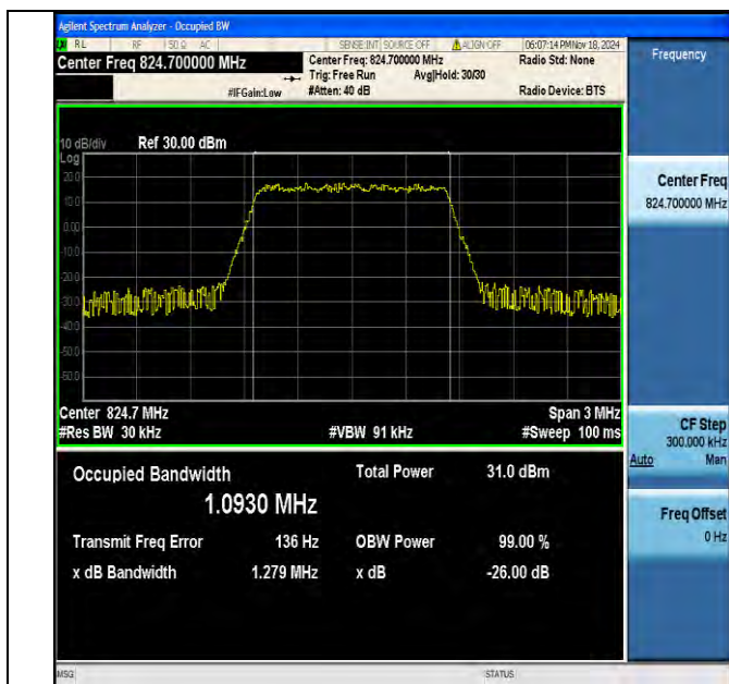
Band5-1.4MHz-QPSK-20407-6RB#0-PASS
