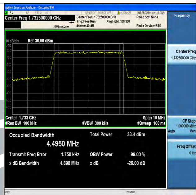
Band4-5MHz-QPSK-20175-25RB#0-PASS
