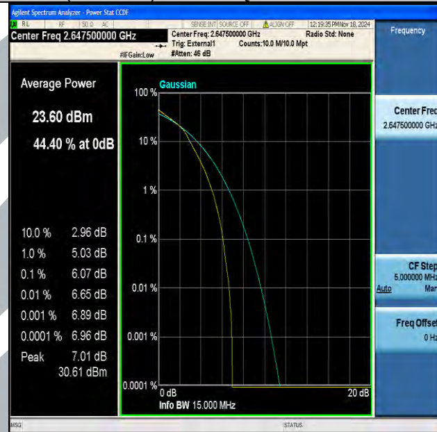
Band41(2535-2655)-15MHz-16QAM-41165-75RB#0-PASS
