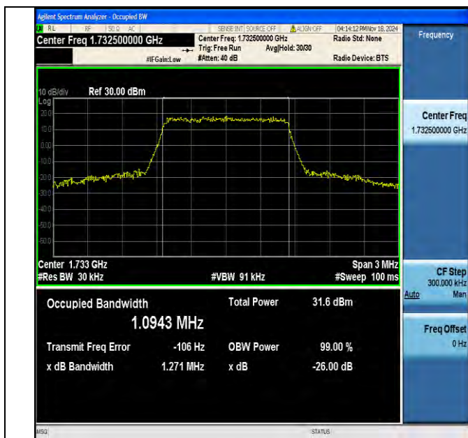
Band4-1.4MHz-16QAM-20175-6RB#0-PASS
