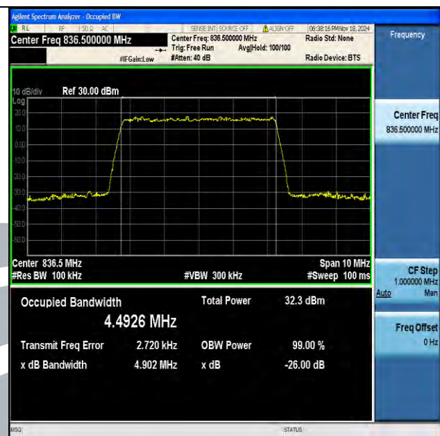
Band5-5MHz-QPSK-20525-25RB#0-PASS
