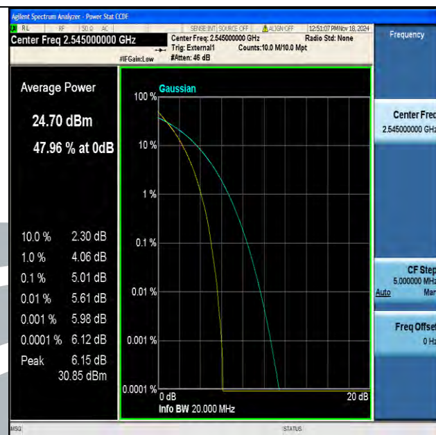
Band41(2535-2655)-20MHz-QPSK-40140-100RB#0-PASS
