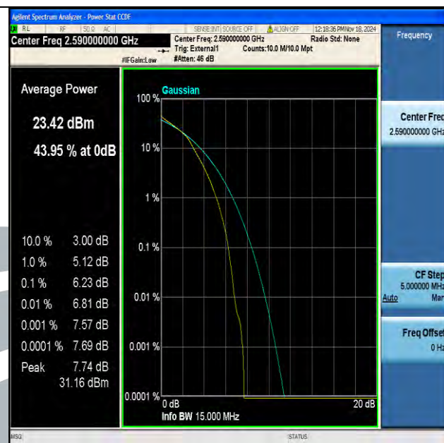
Band41(2535-2655)-15MHz-16QAM-40590-75RB#0-PASS
