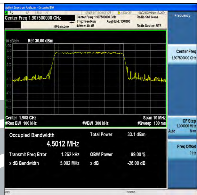
Band2-5MHz-16QAM-19175-25RB#0-PASS
