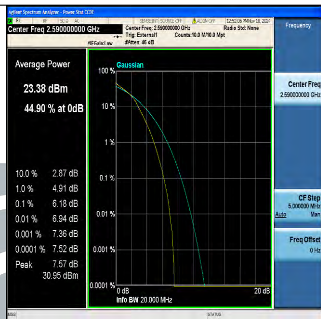
Band41(2535-2655)-20MHz-16QAM-40590-100RB#0-PASS
