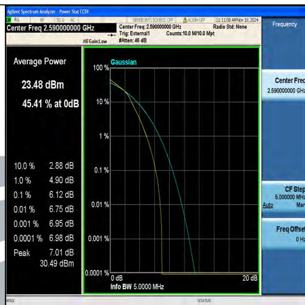
Band41(2535-2655)-5MHz-16QAM-40590-25RB#0-PASS
