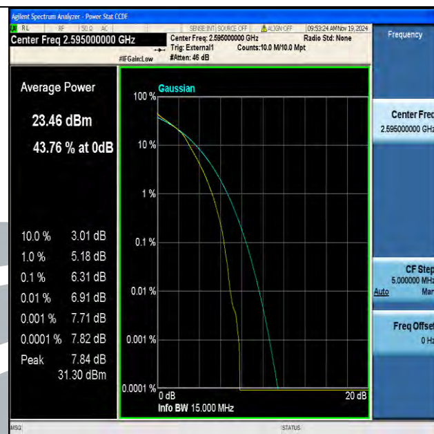
Band38-15MHz-16QAM-38000-75RB#0-PASS
