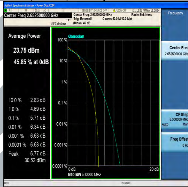
Band41(2535-2655)-5MHz-16QAM-41215-25RB#0-PASS
