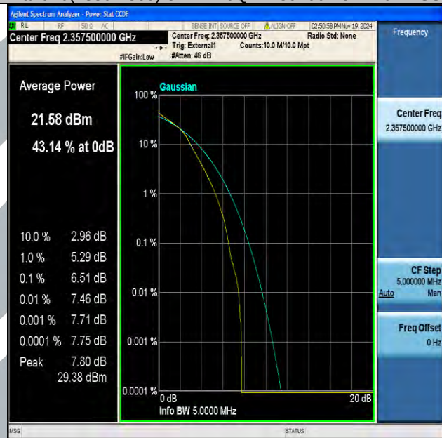
Band40(2350-2360)-5MHz-16QAM-39225-25RB#0-PASS
