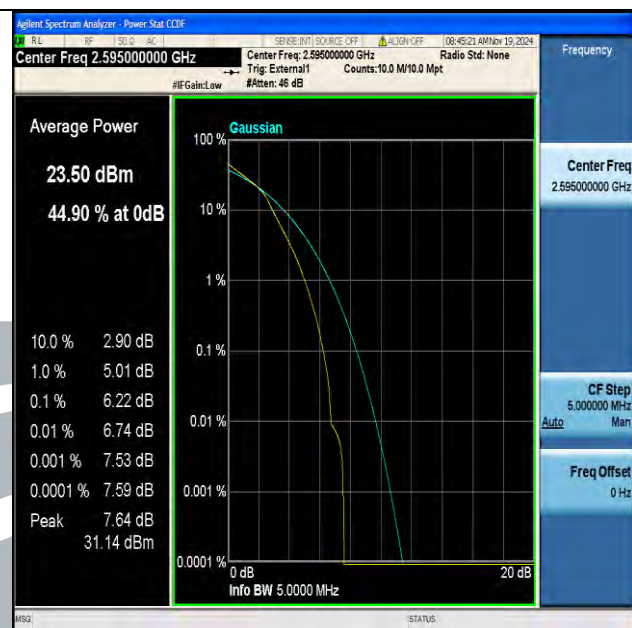
Band38-5MHz-16QAM-38000-25RB#0-PASS
