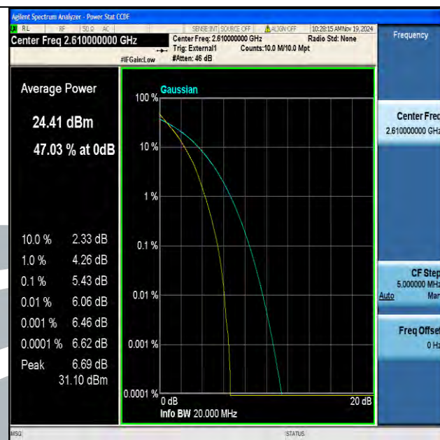
Band38-20MHz-QPSK-38150-100RB#0-PASS
