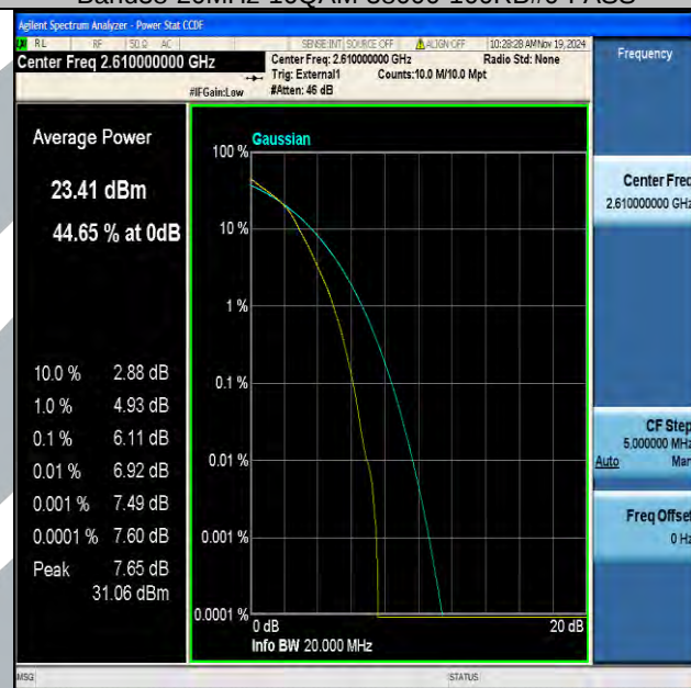
Band38-20MHz-16QAM-38150-100RB#0-PASS
