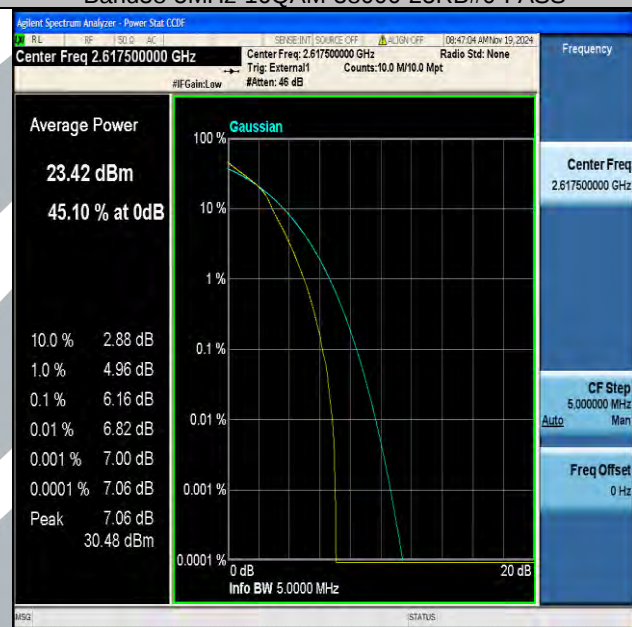
Band38-5MHz-16QAM-38225-25RB#0-PASS
