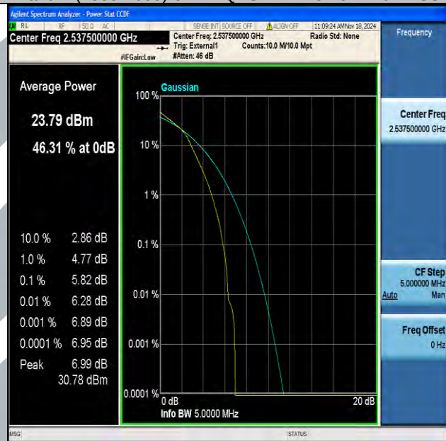
Band41(2535-2655)-5MHz-16QAM-40065-25RB#0-PASS
