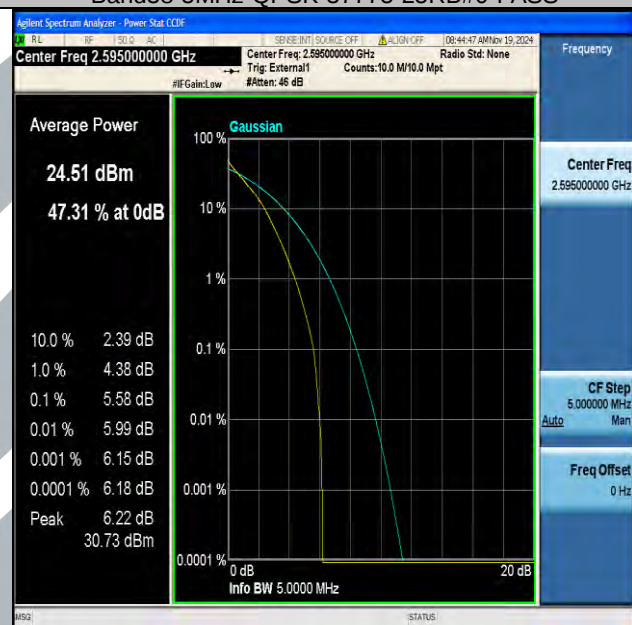
Band38-5MHz-QPSK-38000-25RB#0-PASS
