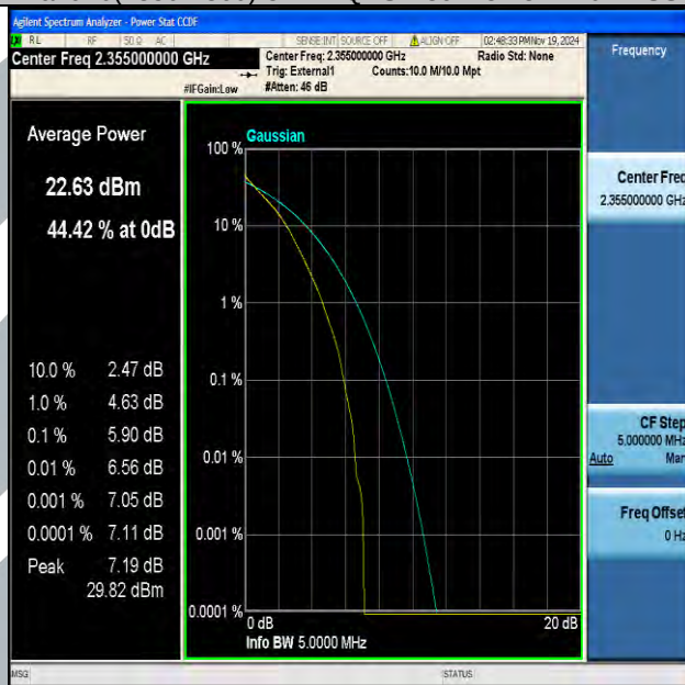
Band40(2350-2360)-5MHz-QPSK-39200-25RB#0-PASS
