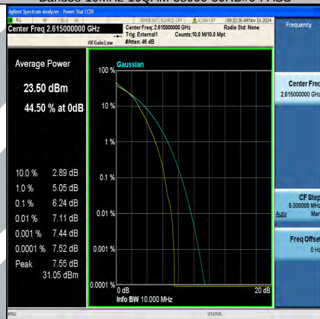
Band38-10MHz-16QAM-38200-50RB#0-PASS
