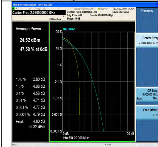
Band38-20MHz-16QAM-37850-1RB#0-PASS
