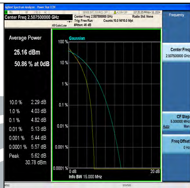
Band7-15MHz-QPSK-20825-75RB#0-PASS
