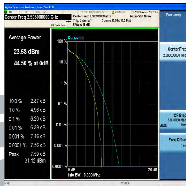
Band38-10MHz-16QAM-38000-50RB#0-PASS
