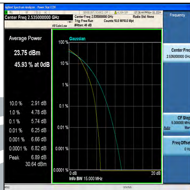
Band7-15MHz-16QAM-21100-75RB#0-PASS
