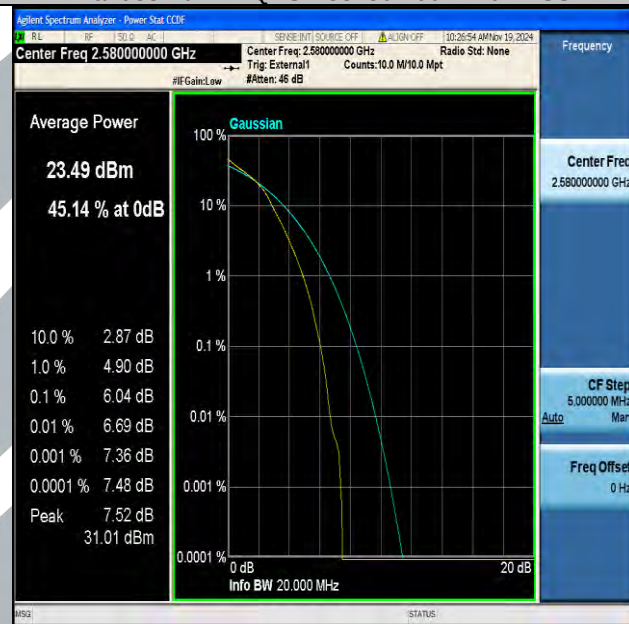
Band38-20MHz-16QAM-37850-100RB#0-PASS
