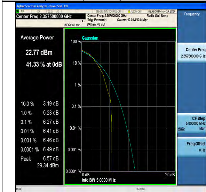
Band40(2350-2360)-5MHz-16QAM-39225-1RB#0-PASS
