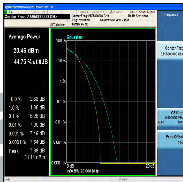
Band38-20MHz-16QAM-38000-100RB#0-PASS
