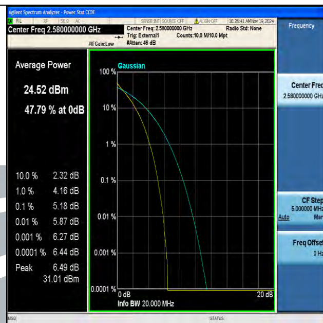
Band38-20MHz-QPSK-37850-100RB#0-PASS
