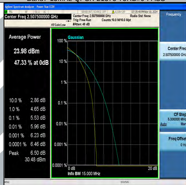
Band7-15MHz-16QAM-20825-75RB#0-PASS
