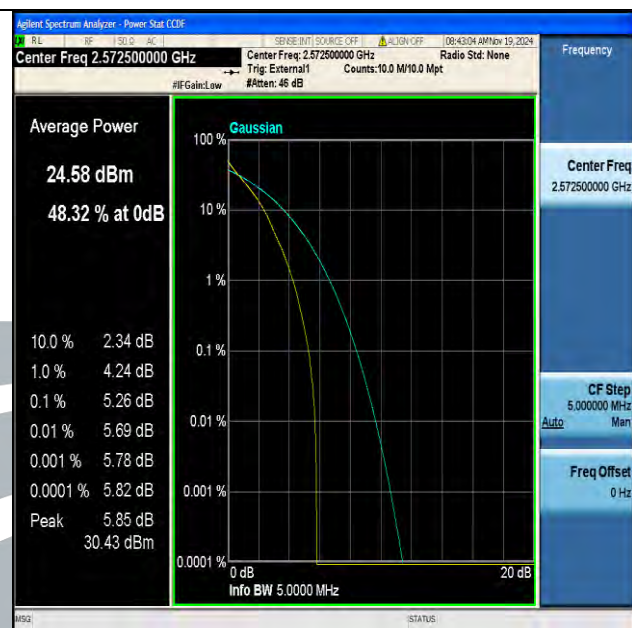
Band38-5MHz-QPSK-37775-25RB#0-PASS
