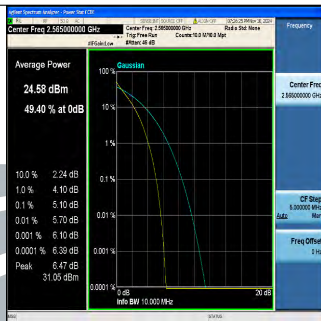
Band7-10MHz-QPSK-21400-50RB#0-PASS
