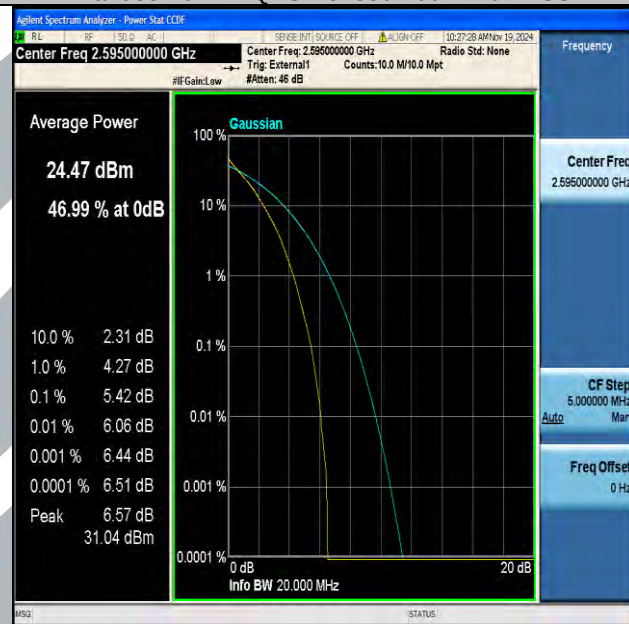
Band38-20MHz-QPSK-38000-100RB#0-PASS
