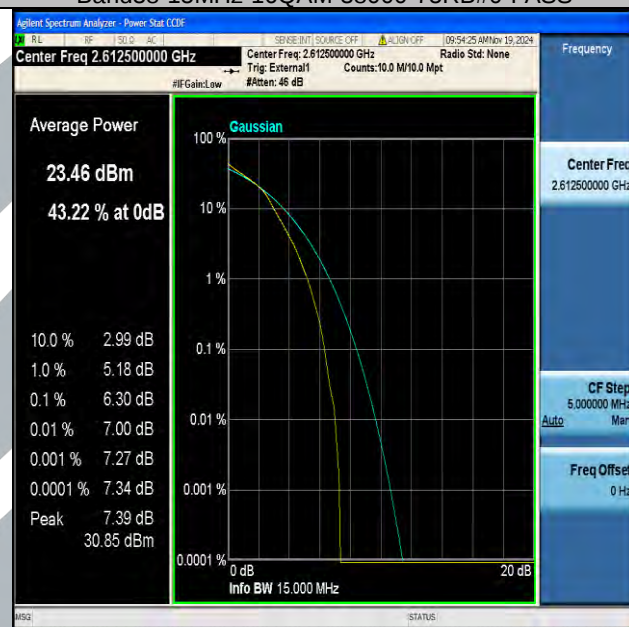
Band38-15MHz-16QAM-38175-75RB#0-PASS
