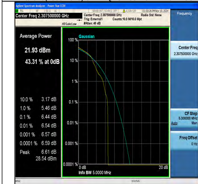
Band40(2305-2315)-5MHz-16QAM-38725-1RB#0-PASS
