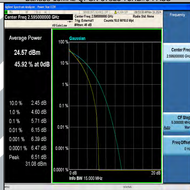
Band38-15MHz-QPSK-38000-75RB#0-PASS
