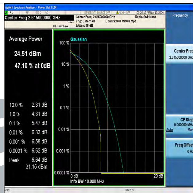
Band38-10MHz-QPSK-38200-50RB#0-PASS
