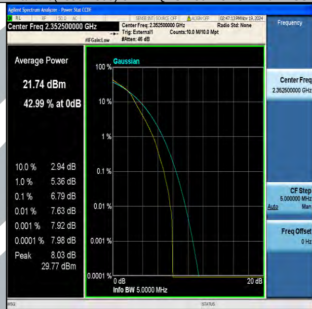
Band40(2350-2360)-5MHz-16QAM-39175-25RB#0-PASS
