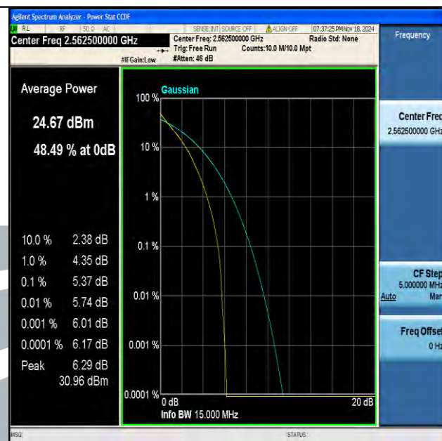
Band7-15MHz-QPSK-21375-75RB#0-PASS
