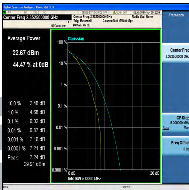
Band40(2350-2360)-5MHz-QPSK-39175-25RB#0-PASS
