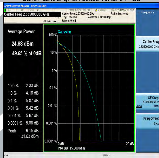
Band7-15MHz-QPSK-21100-75RB#0-PASS
