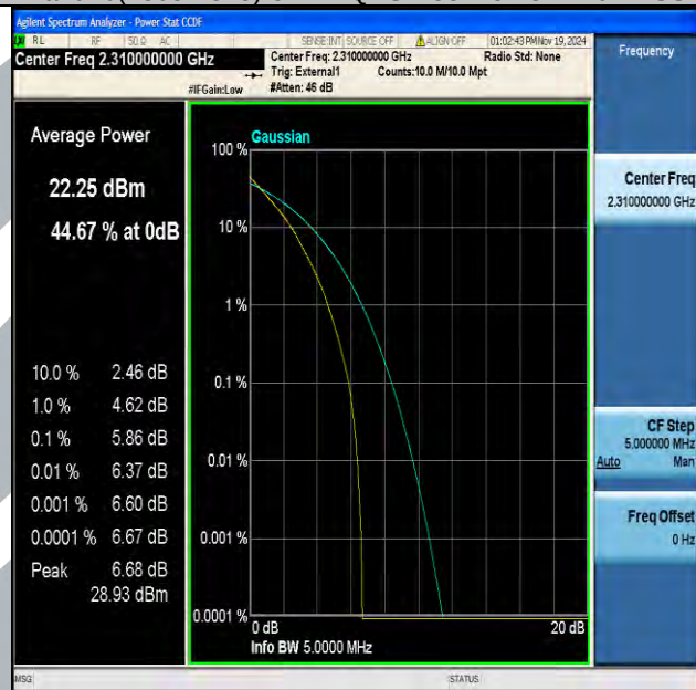
Band40(2305-2315)-5MHz-QPSK-38750-25RB#0-PASS
