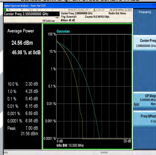
Band38-10MHz-QPSK-38000-50RB#0-PASS
