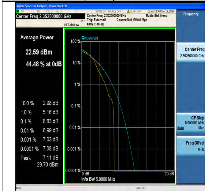
Band40(2350-2360)-5MHz-16QAM-39175-1RB#0-PASS
