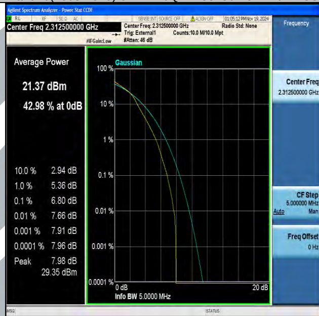
Band40(2305-2315)-5MHz-16QAM-38775-25RB#0-PASS
