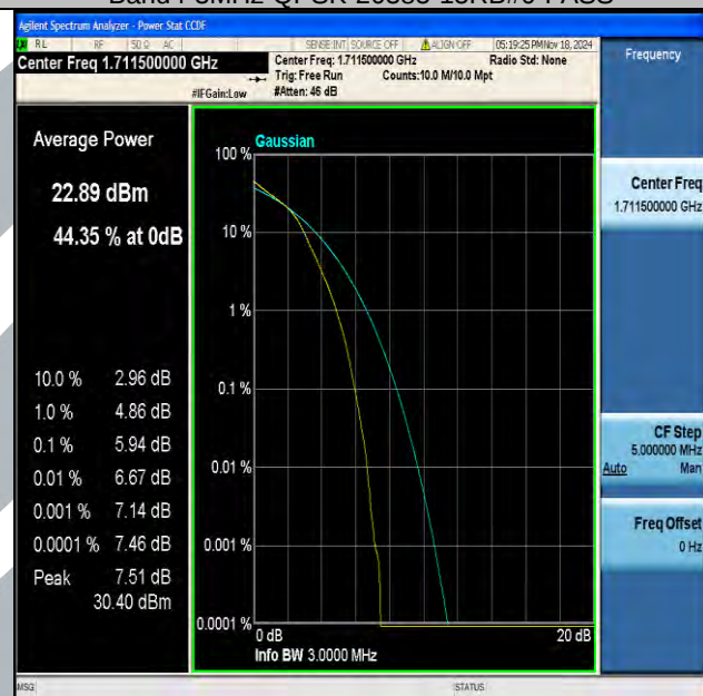
Band4-3MHz-16QAM-19965-15RB#0-PASS
