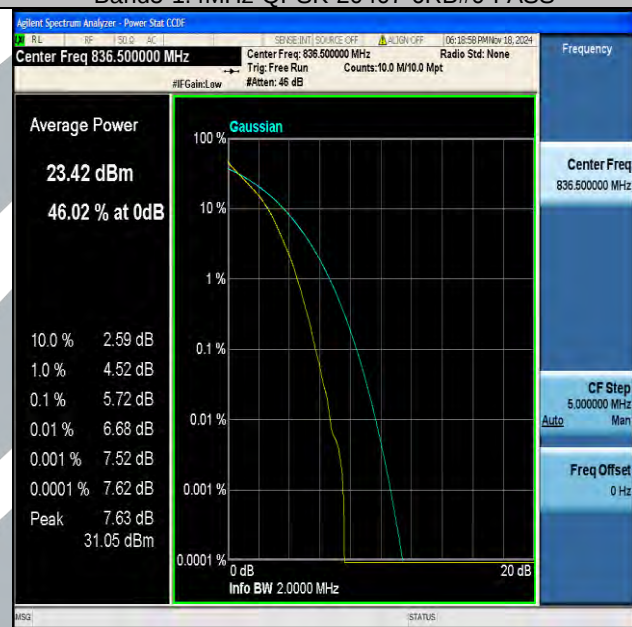
Band5-1.4MHz-QPSK-20525-6RB#0-PASS
