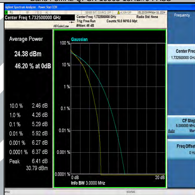
Band4-3MHz-QPSK-20175-15RB#0-PASS
