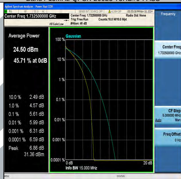
Band4-15MHz-QPSK-20175-75RB#0-PASS
