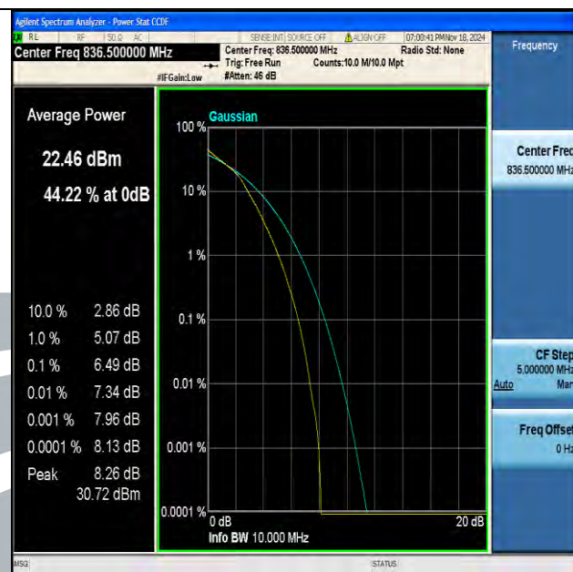
Band5-10MHz-16QAM-20525-50RB#0-PASS
