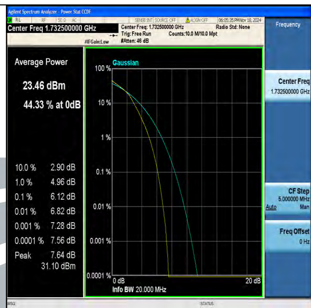
Band4-20MHz-16QAM-20175-100RB#0-PASS
