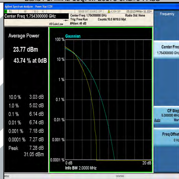
Band4-1.4MHz-16QAM-20393-6RB#0-PASS
