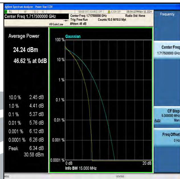
Band4-15MHz-QPSK-20025-75RB#0-PASS
