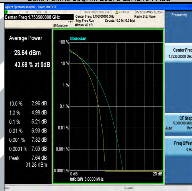
Band4-3MHz-16QAM-20385-15RB#0-PASS
