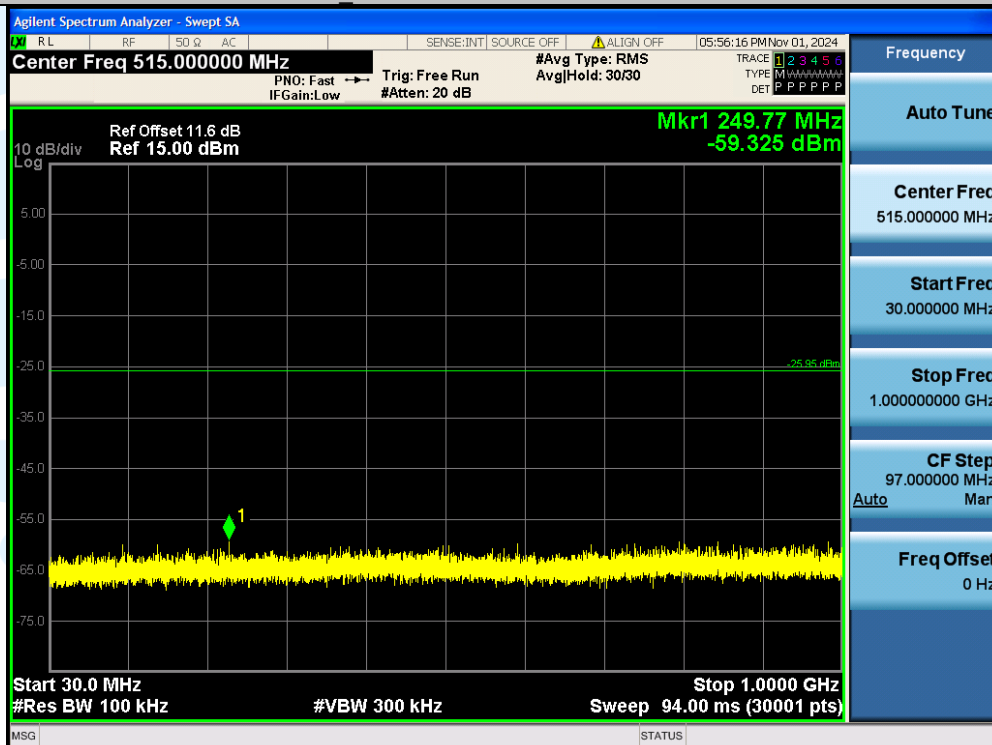
BLE_1M-Ant1-2440-30~1000-PASS
