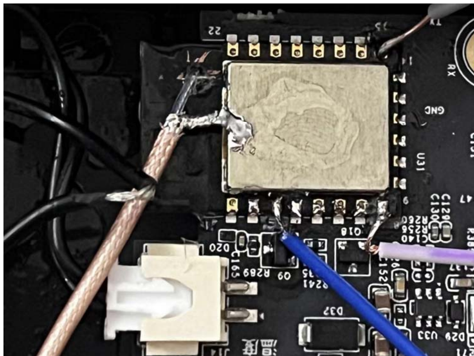
(Antenna connector)
