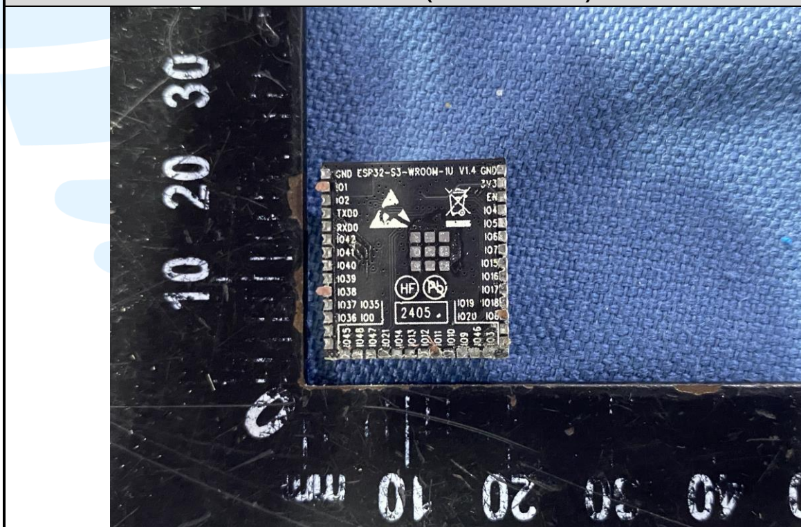
EUT Photo (BT&WI-Fi module)
