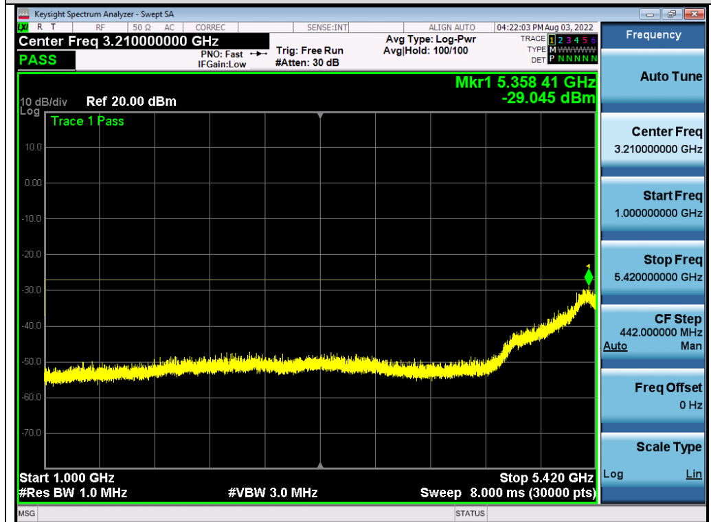
Test_Graph_802.11a_ANT1_5700_6Mbps_Frequency Band 2
