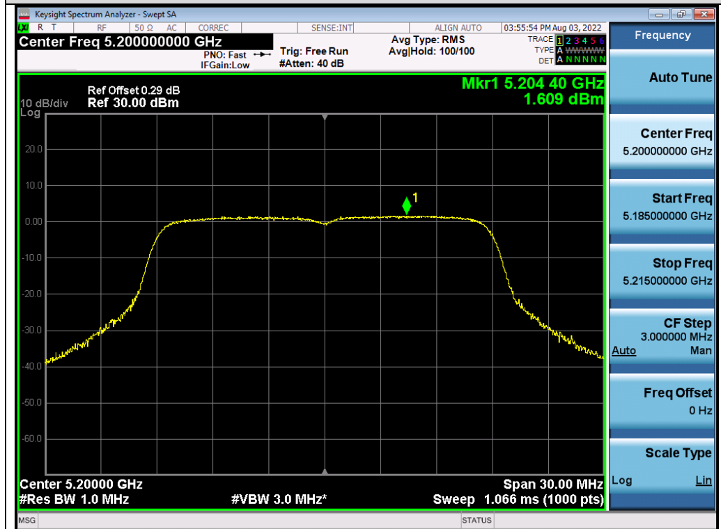
Test_Graph_802.11n20_ANT1_5200_MCS0_PSD
