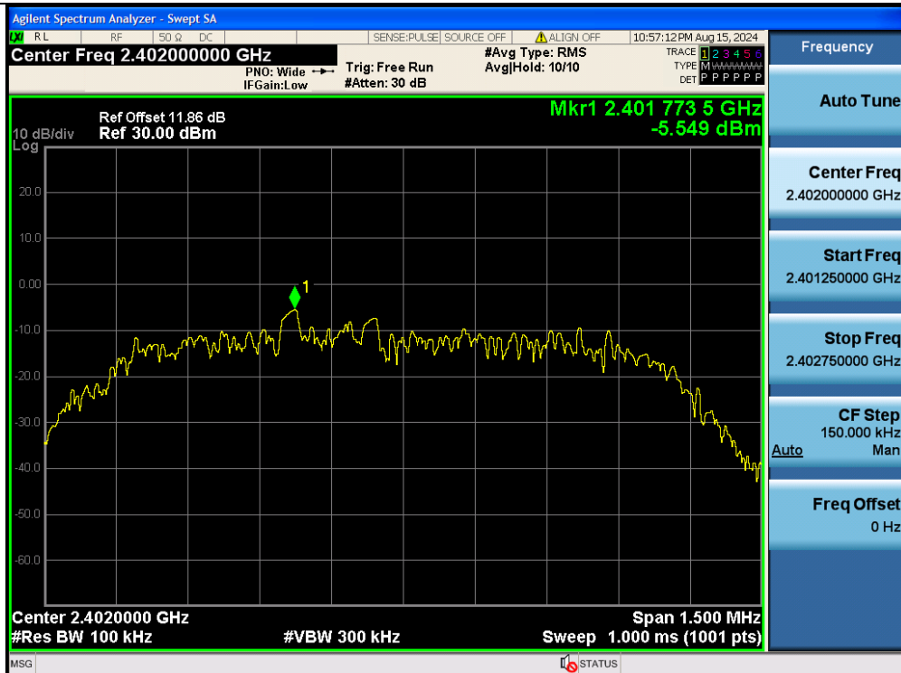
3DH5-Ant1-2402-30-1000-PASS
