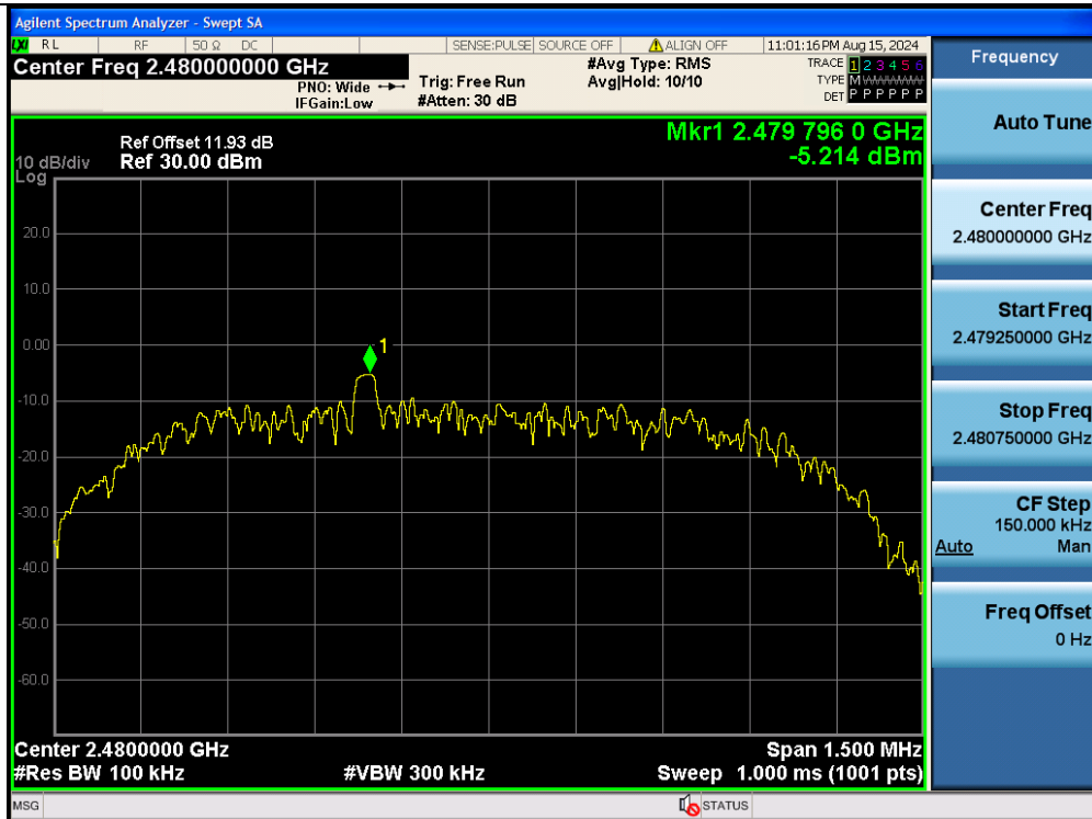
3DH5-Ant1-2480-30-1000-PASS
