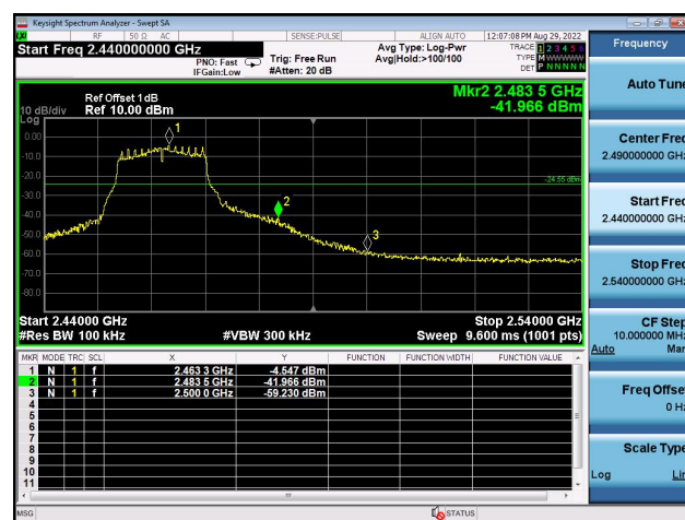
Right bandedge
