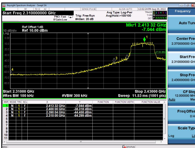
Left bandedge
