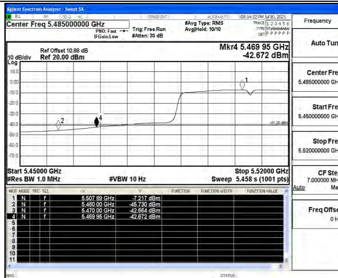
11AC40SISO_Ant1_Low_5510_Peak
