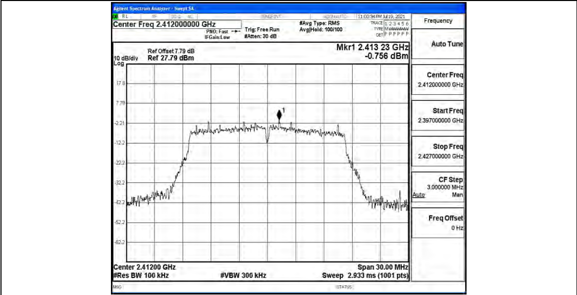
11G_Ant1_2412_0~Reference
