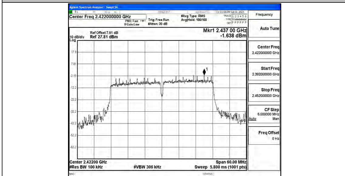
11N40ISO_Ant1_2422_0~Reference
