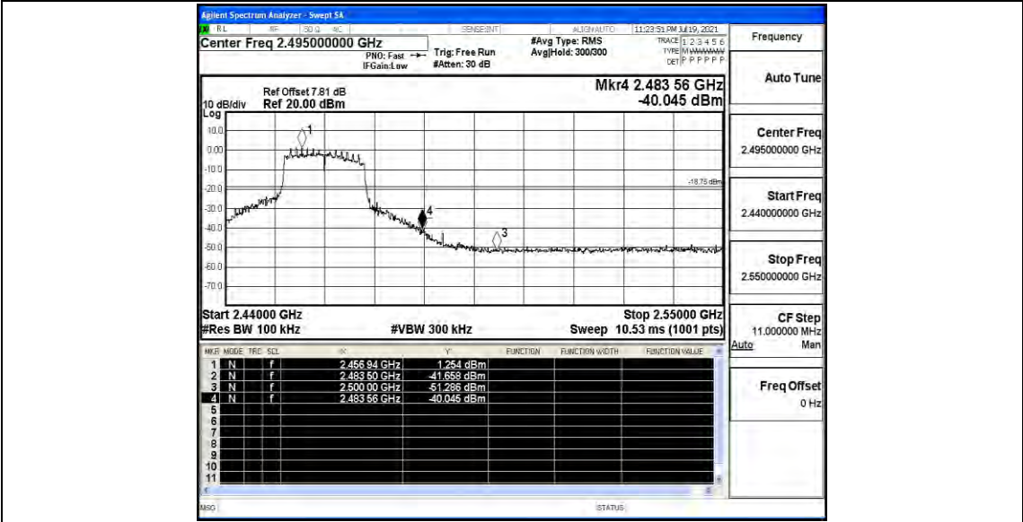
11N20SISO_Ant1_High_2462
