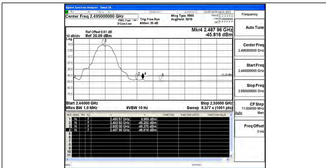
11B_Ant1_High_2462_AV
