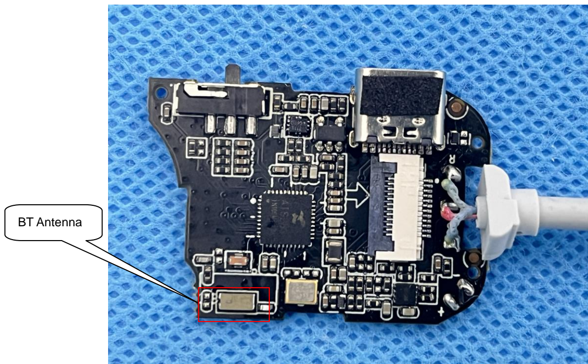
INTERNAL VIEW OF EUT (FIGURE 3)
