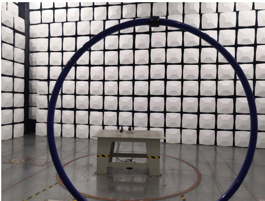
Radiated Emission Below 30M View
