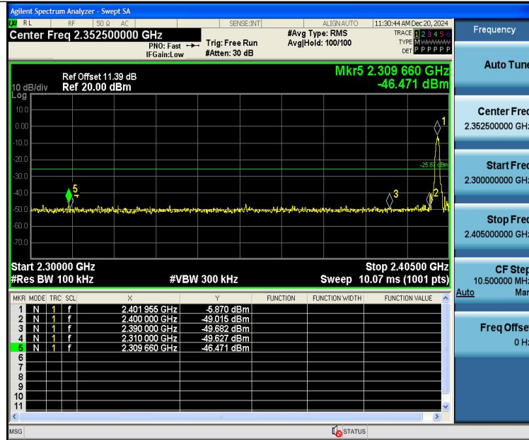
2.4G -Ant1-2402-PASS
