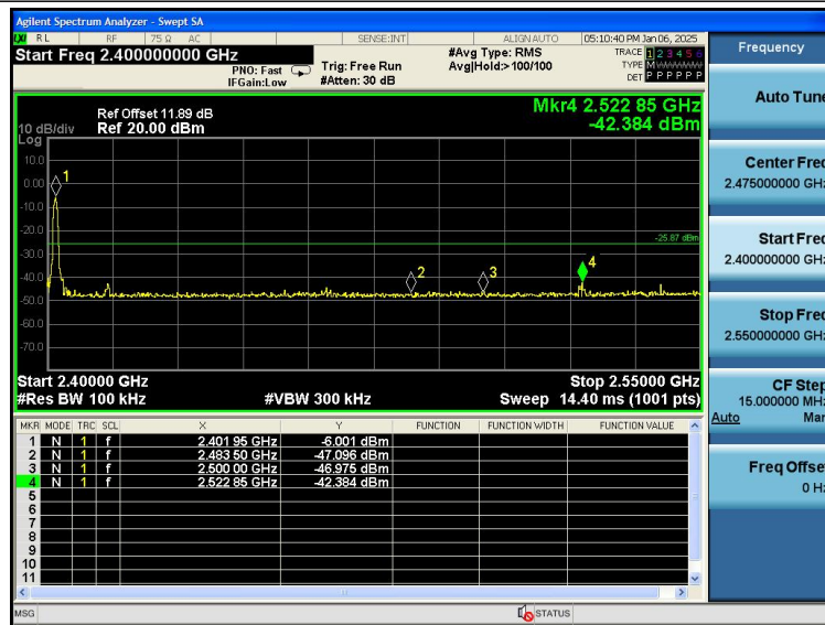
2.4G -Ant1-2402-PASS
