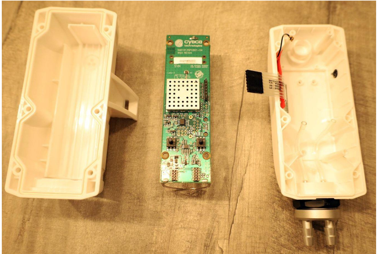
Removed main PCB view
