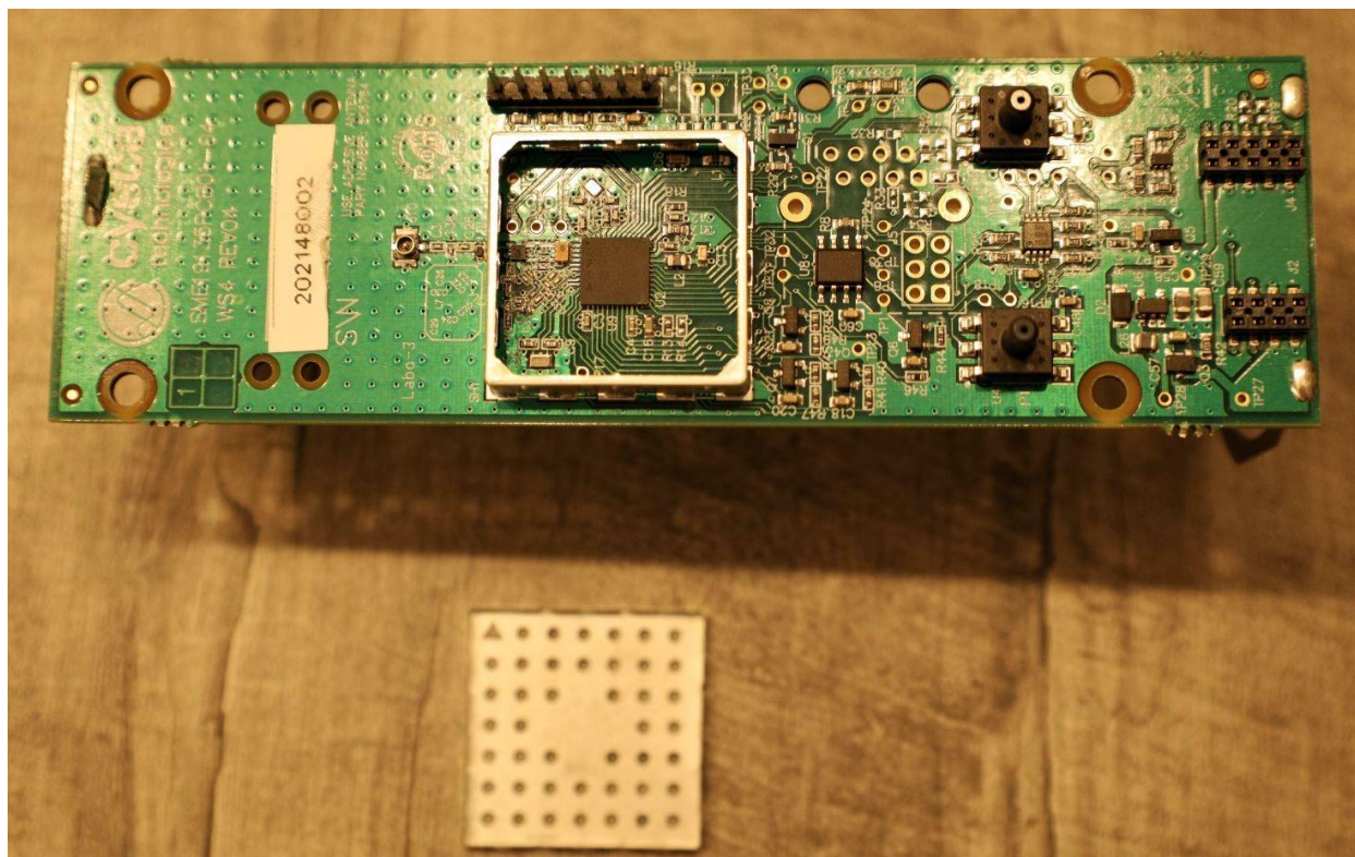
RF shielding removed view
