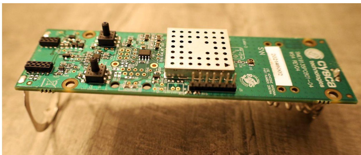
Main PCB top view
