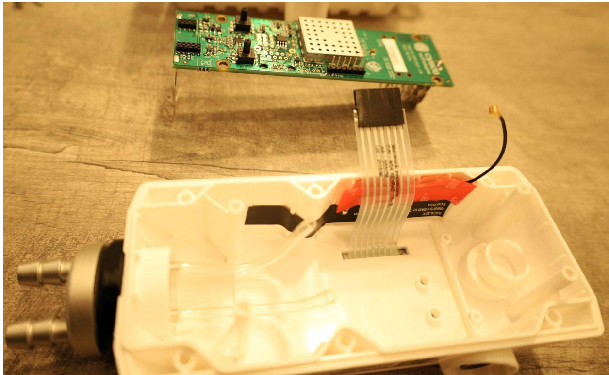
Antenna location view
