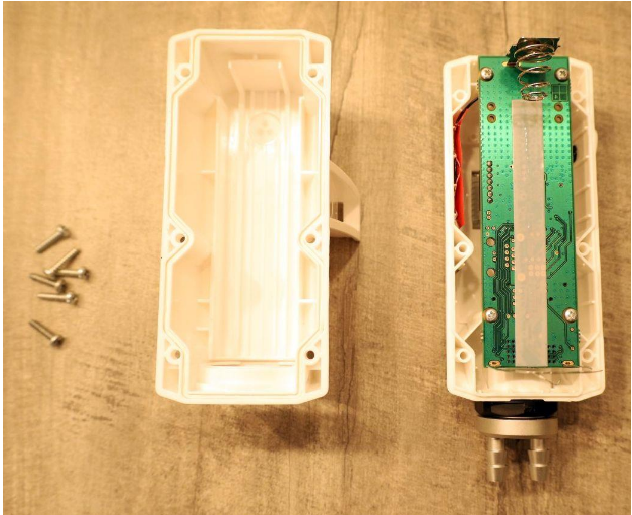
Removed back cover view
