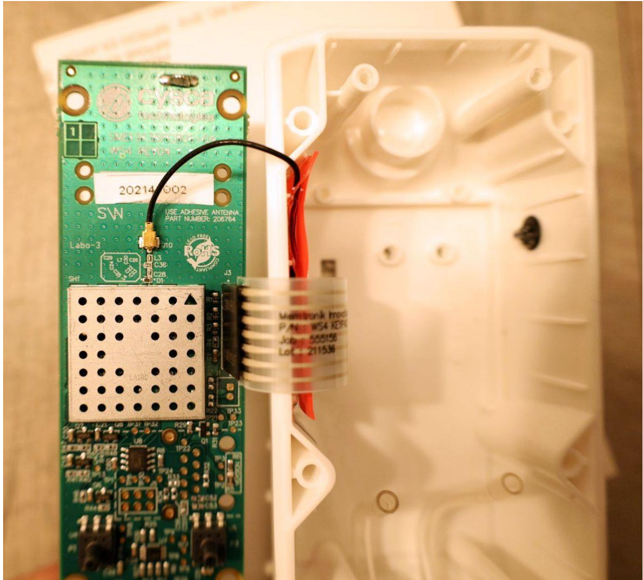
Removed main PCB view
