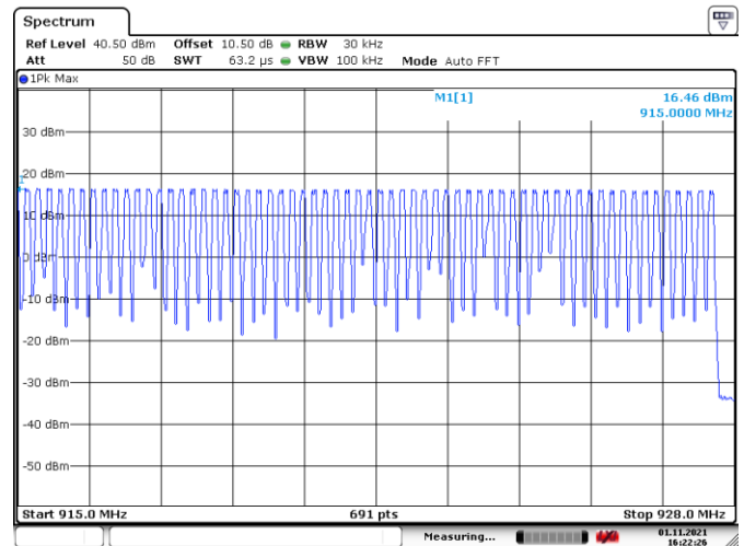
Figure 8.4-9: Number of hopping channels from 915-928 MHz
