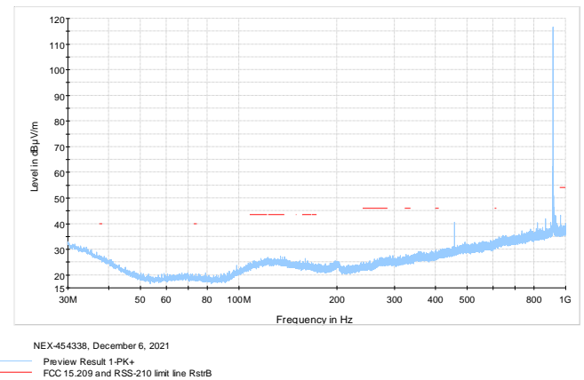
Figure 8.6-7: Radiated spurious emissions 30MHz-1GHz on Mid Ch
