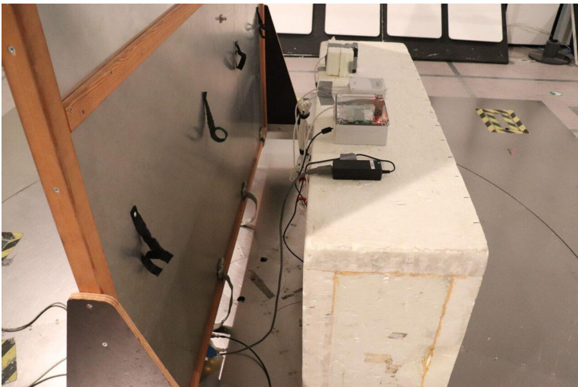
Photograph 2: Test setup for Conducted emissions
