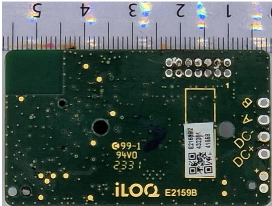
Figure 5: HW version E2159B2, bottom view.
