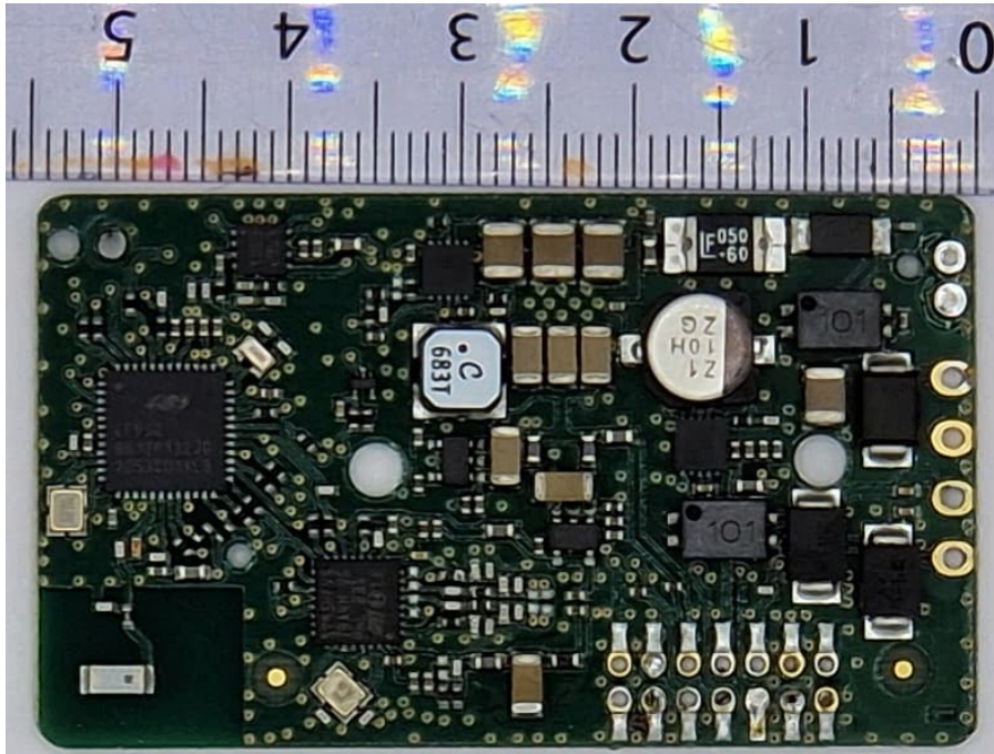
Figure 4: HW version E2159B2, top view.
