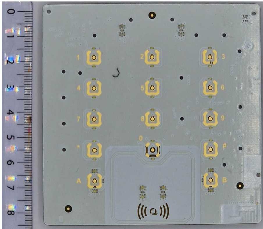
Figure 2: HW version E21336C, top view.
