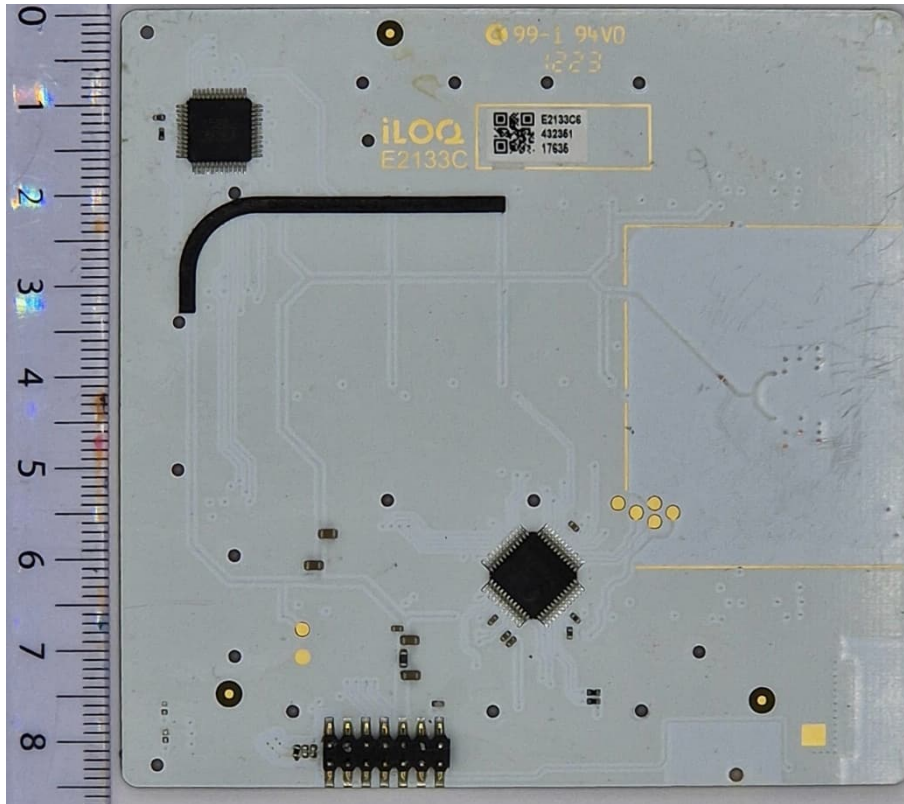
Figure 3: HW version E2133C6, bottom view.
