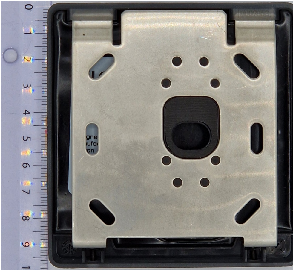
Figure 6: N505i, Bottom view. Mounting bracket assembled.
