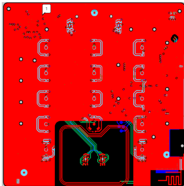
Figure 1. N505i NFC antenna integrated to UI PCB
