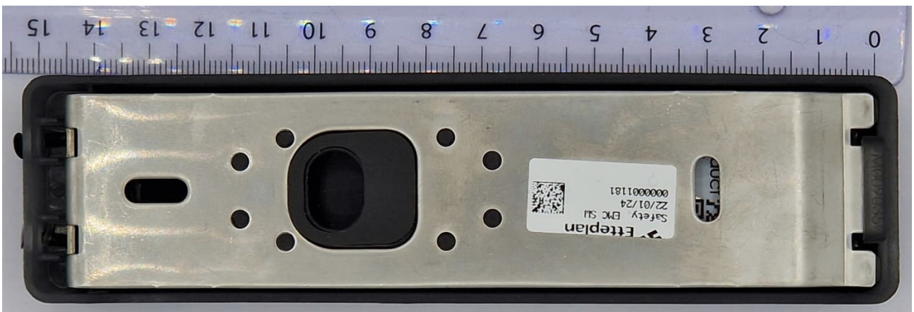
Figure 2: N504i, Bottom view. Mounting bracket assembled
