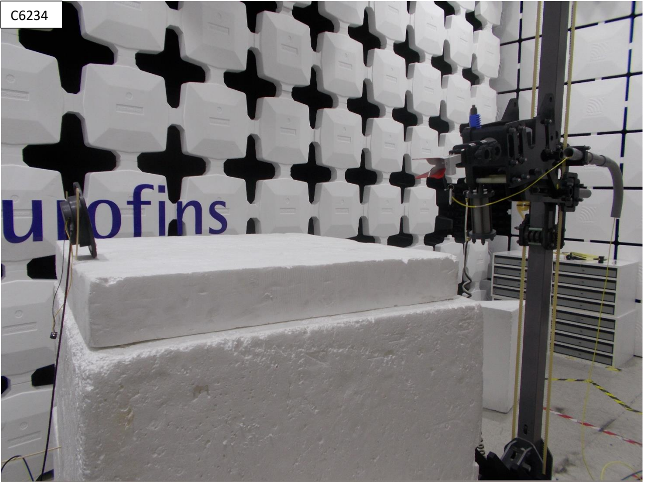
Radiated electric field emissions 18GHz to 26GHz
