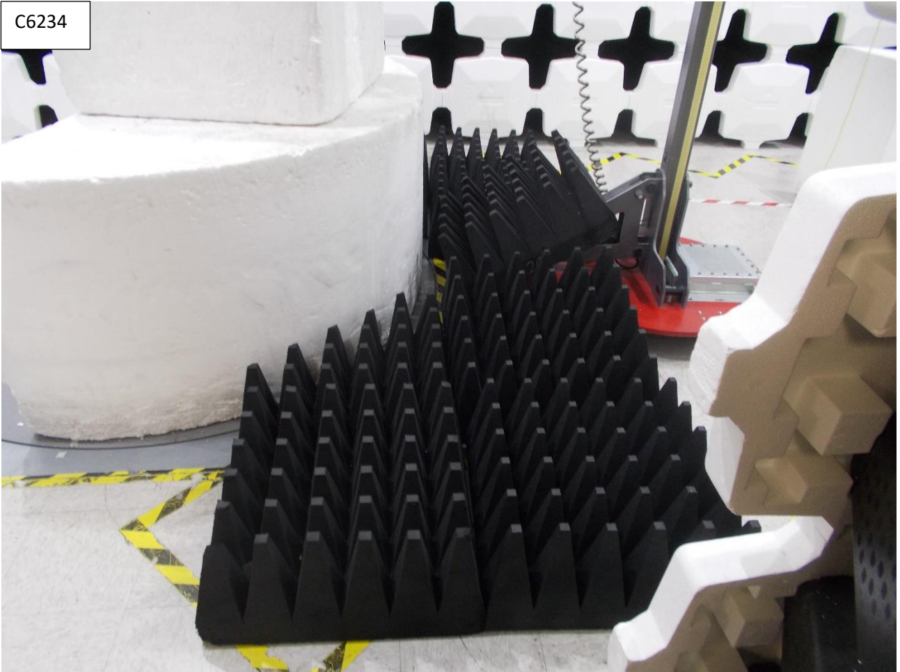
Radiated electric field emissions 18GHz to 26GHz showing position of absorber
