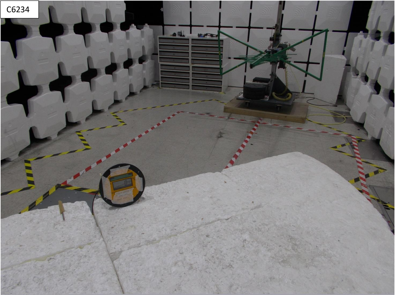
Radiated electric field emissions 30MHz to 1GHz
