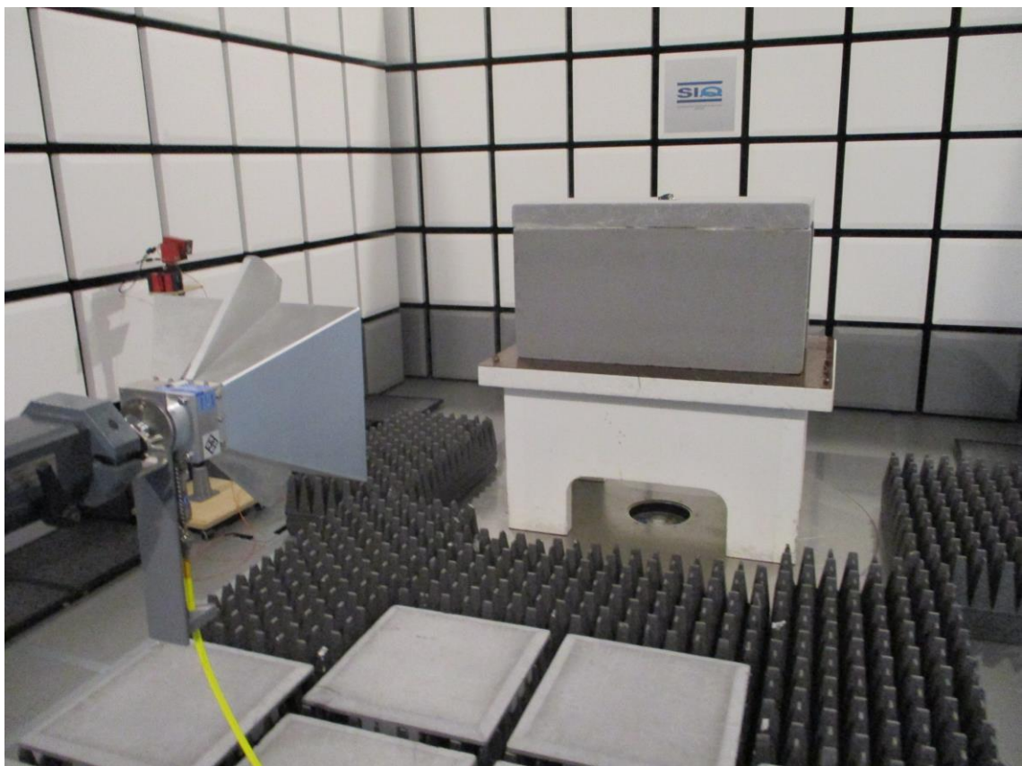
Figure 6: Spurious emission 1- 10 GHz
