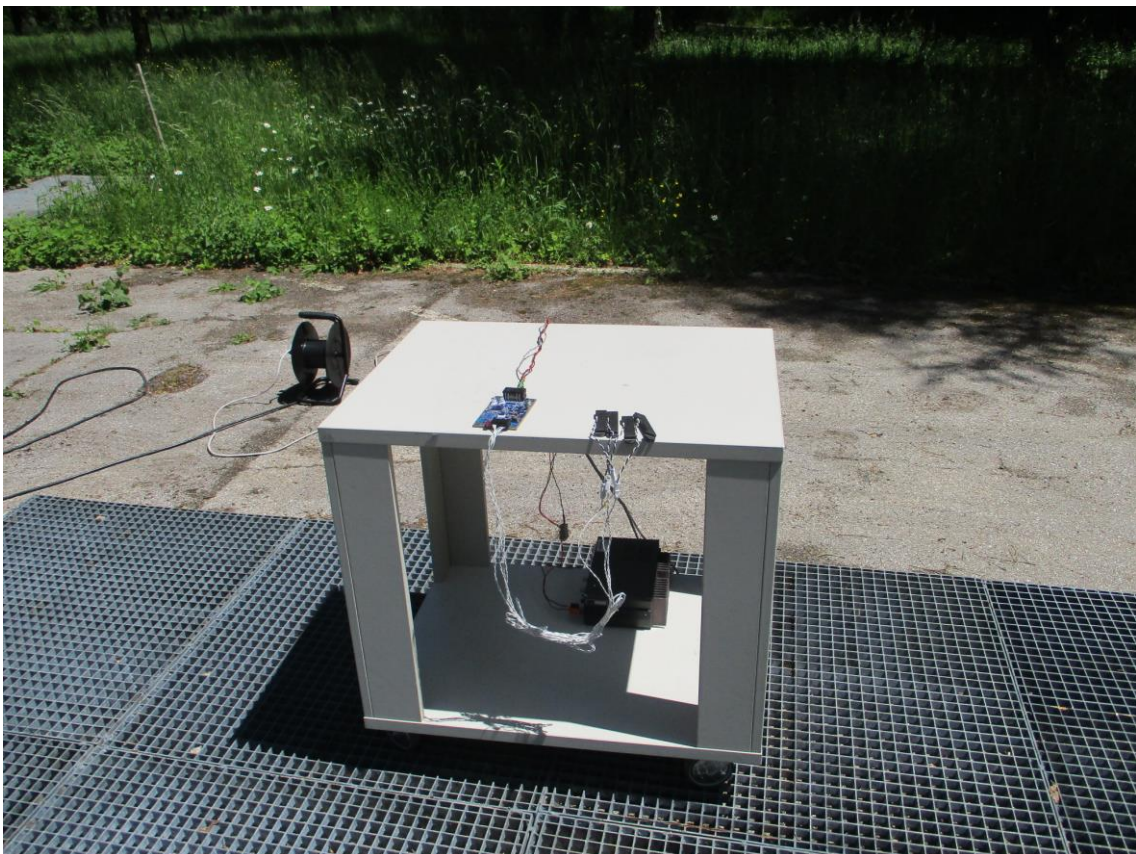
Figure 6: Measurements on OATS
