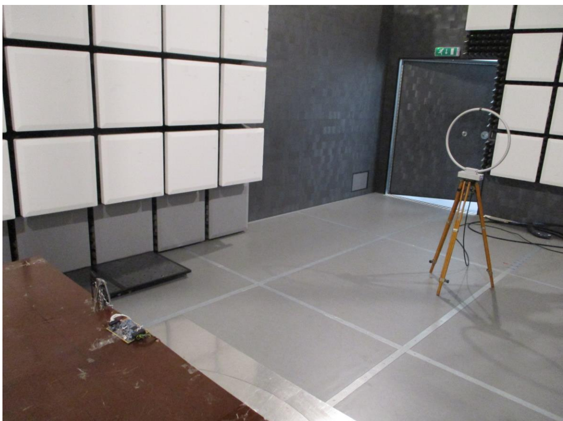
Figure 2: Spurious emission 9 kHz - 30 MHz
