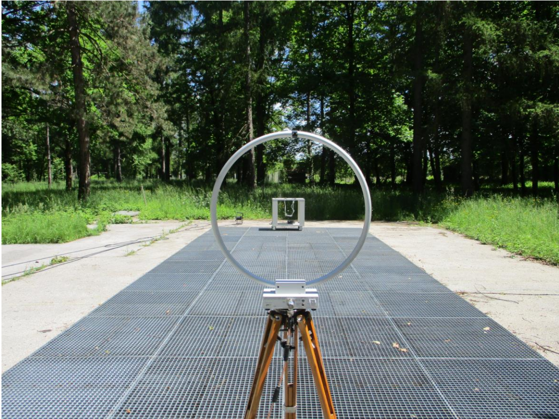
Figure 5: Measurements on OATS
